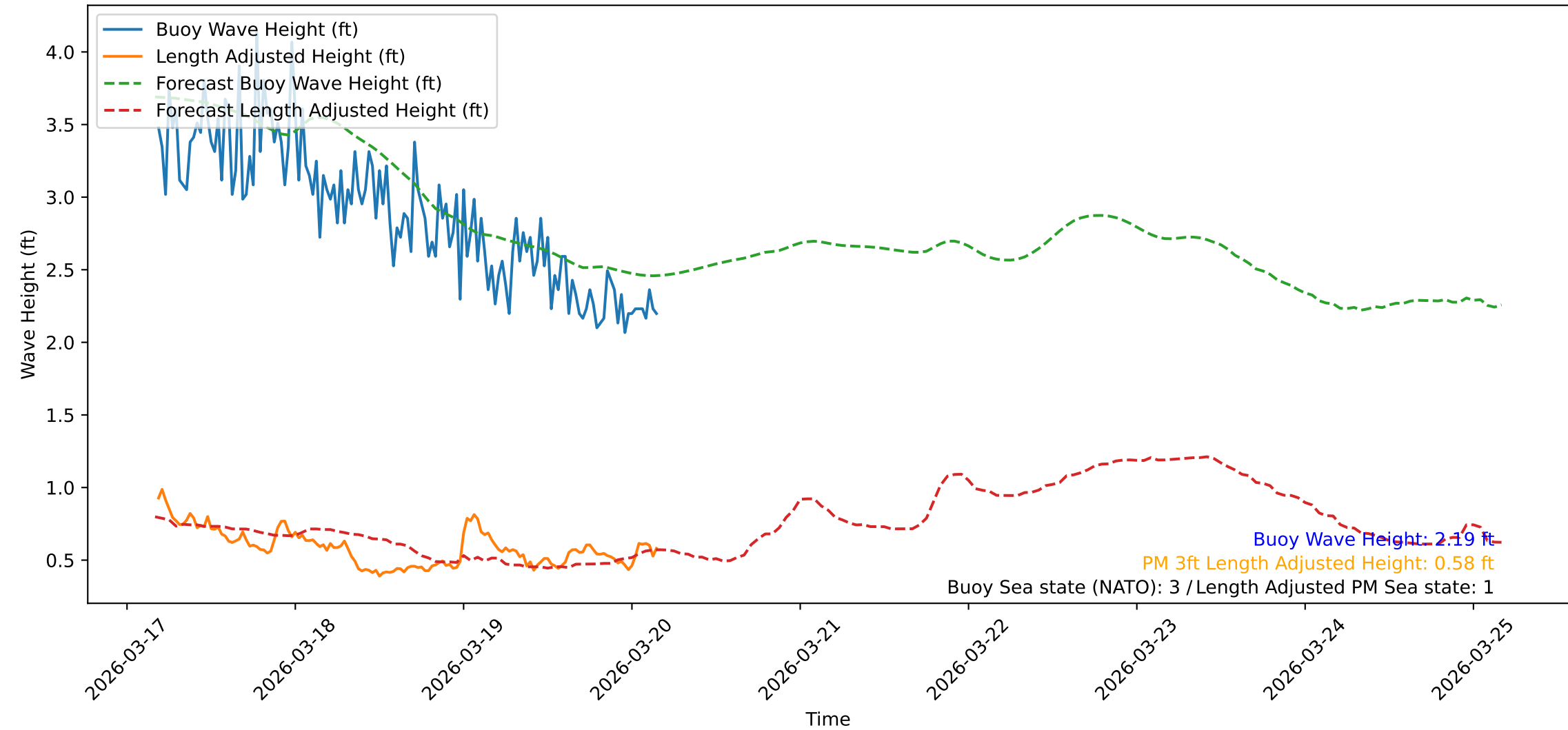
Wave Heights over Time for Green Beach at 2026-03-20 04:21:10
