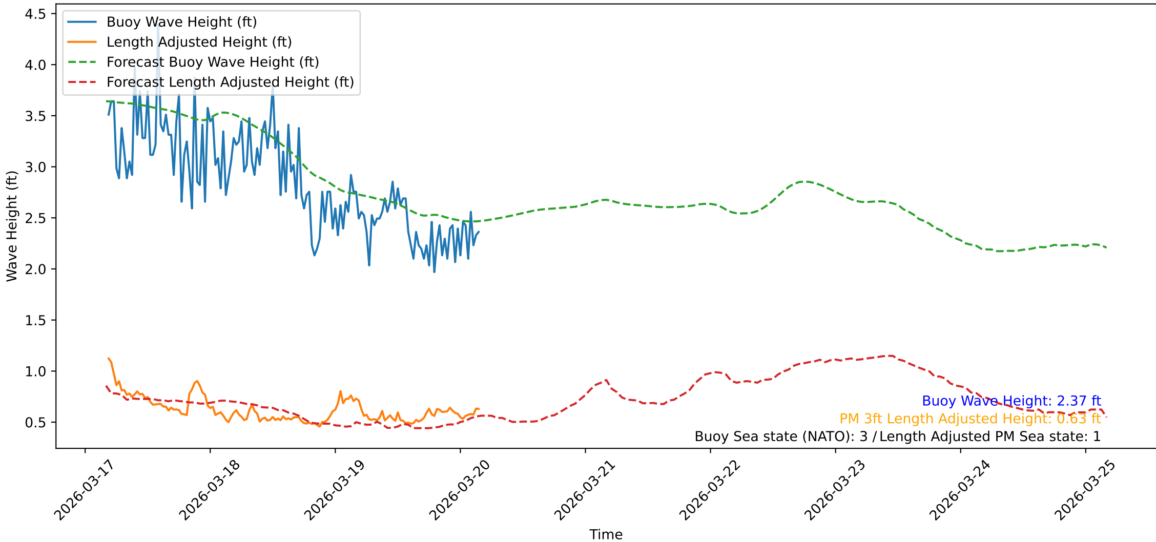
Wave Heights over Time for Oceanside Harbor at 2026-03-20 04:20:31
