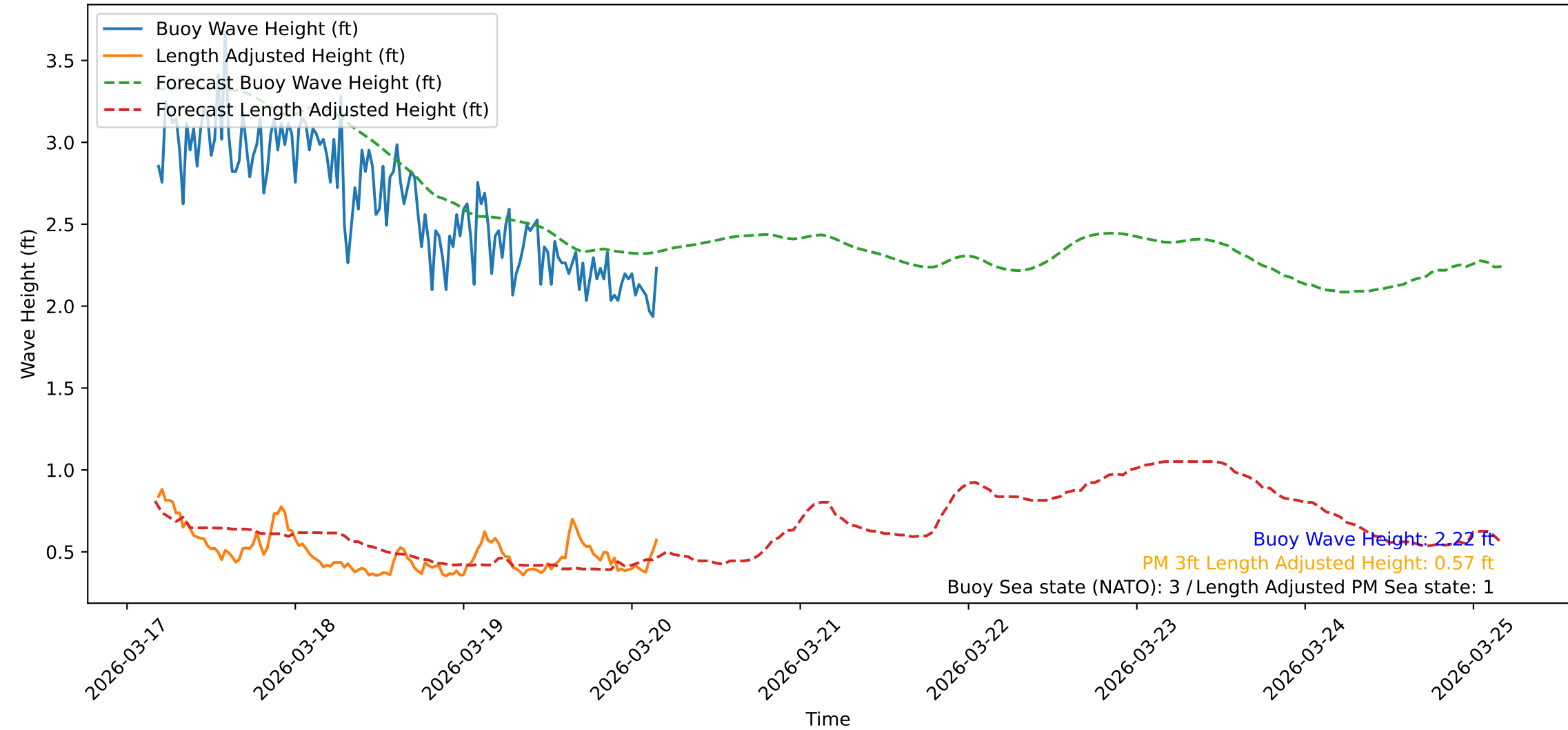
Wave Heights over Time for Red Beach at 2026-03-20 04:20:48
