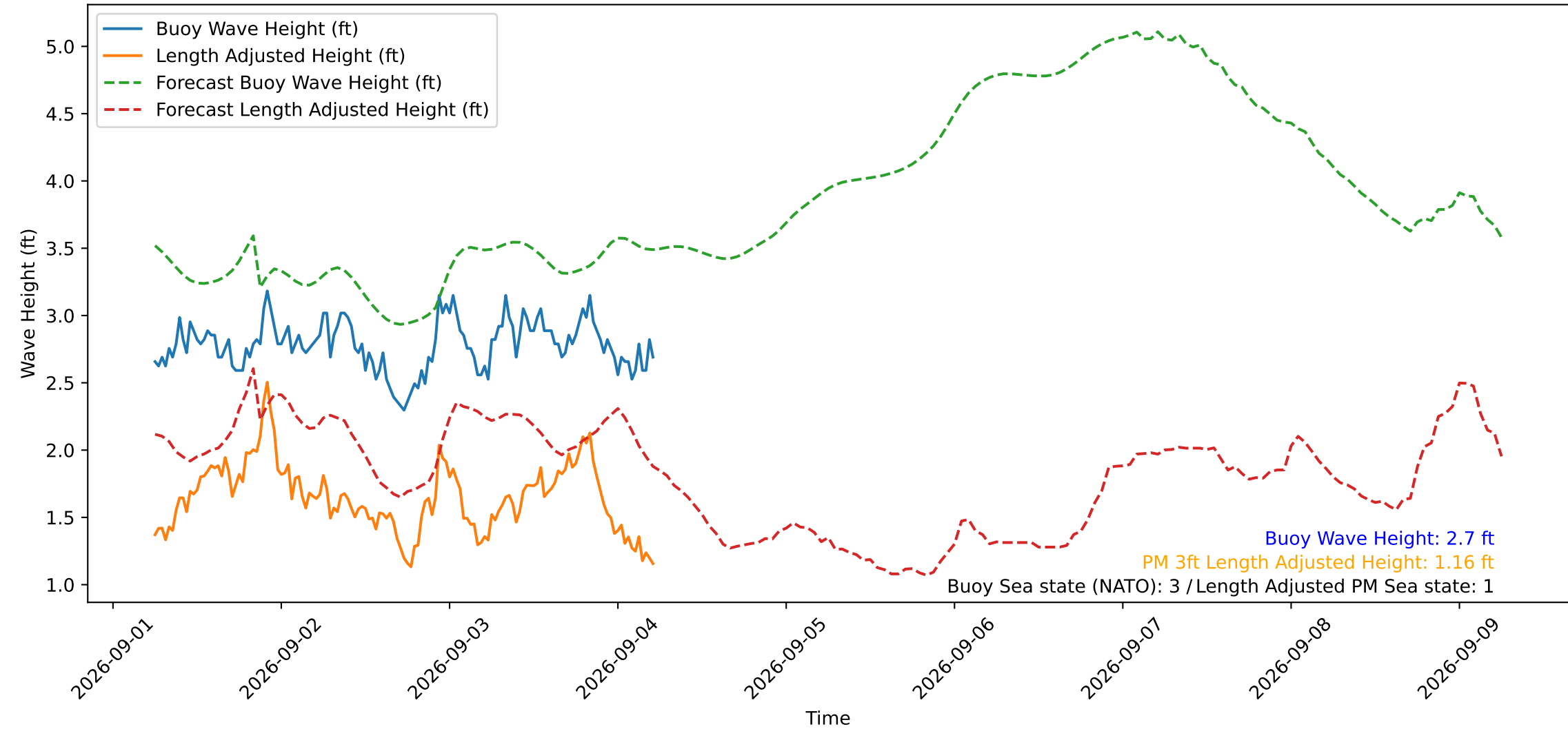
Wave Heights over Time for Red Beach at 2026-09-04 05:50:50
