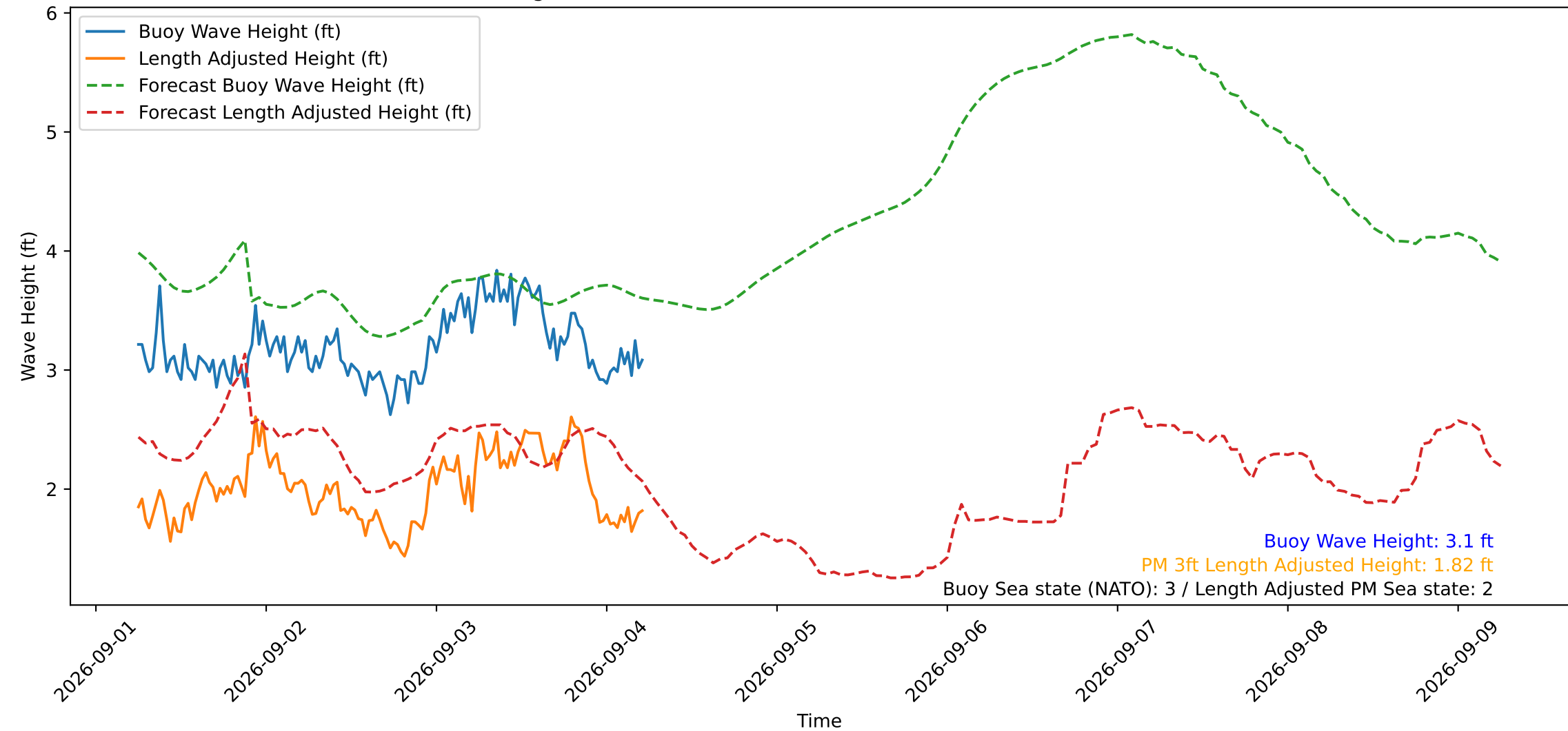
Wave Heights over Time for Oceanside Harbor at 2026-09-04 05:50:29
