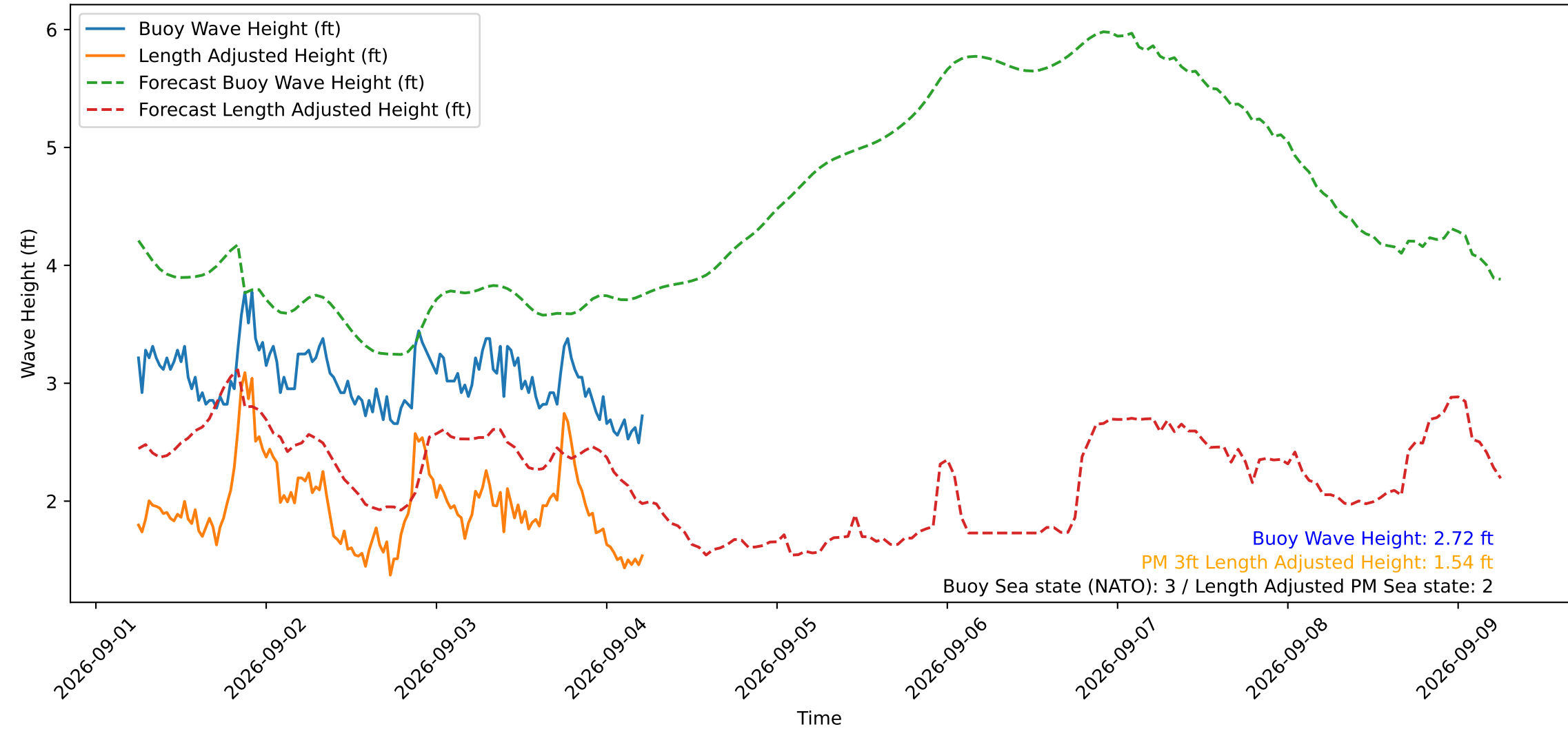
Wave Heights over Time for Green Beach at 2026-09-04 05:51:15
