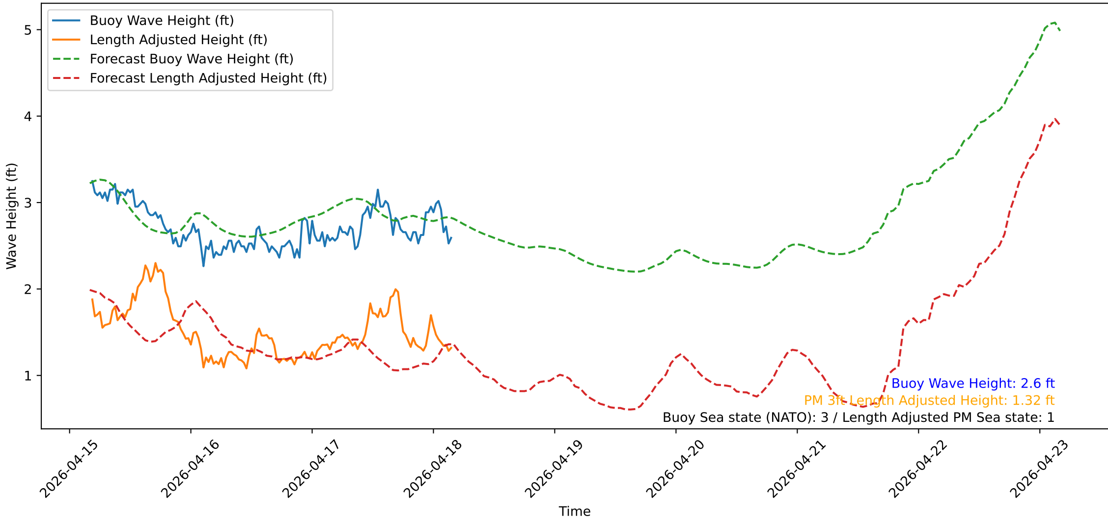
Wave Heights over Time for Red Beach at 2026-04-18 04:10:50
