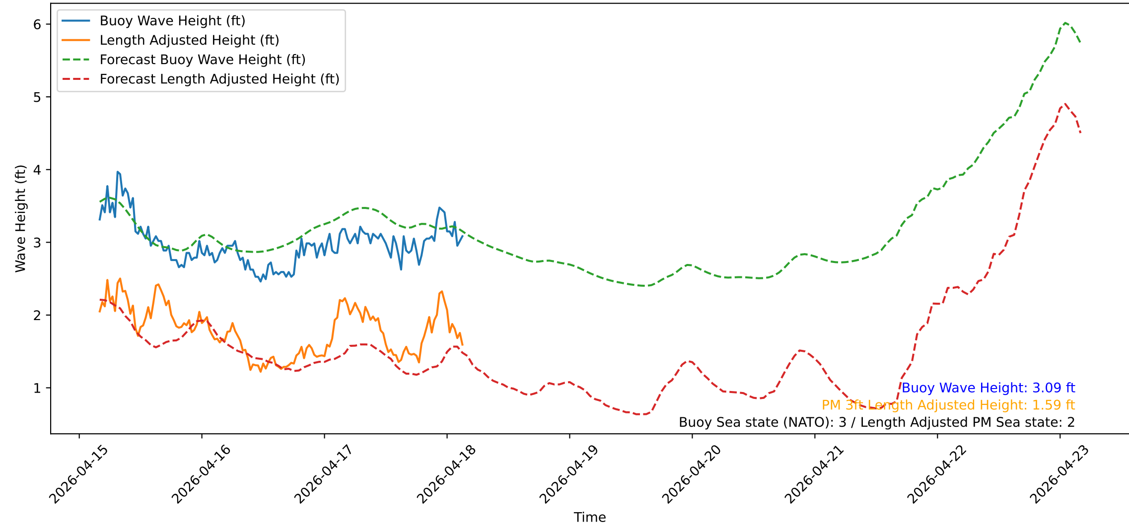
Wave Heights over Time for Green Beach at 2026-04-18 04:11:12
