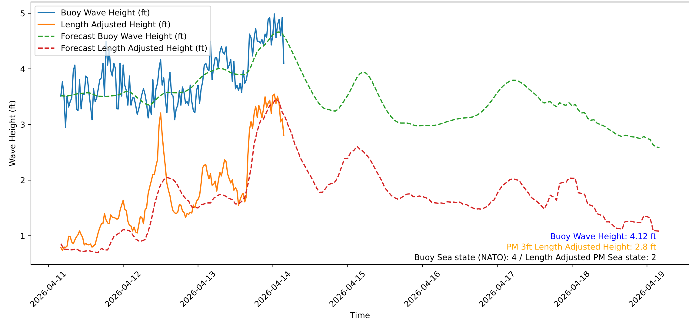
Wave Heights over Time for Green Beach at 2026-04-14 04:11:12
