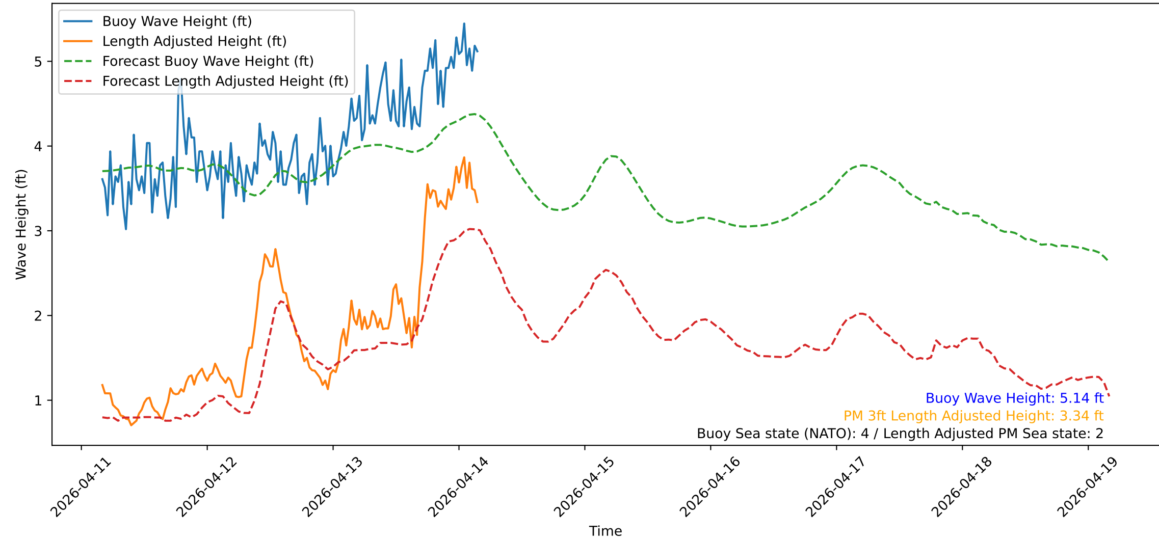
Wave Heights over Time for Oceanside Harbor at 2026-04-14 04:10:31
