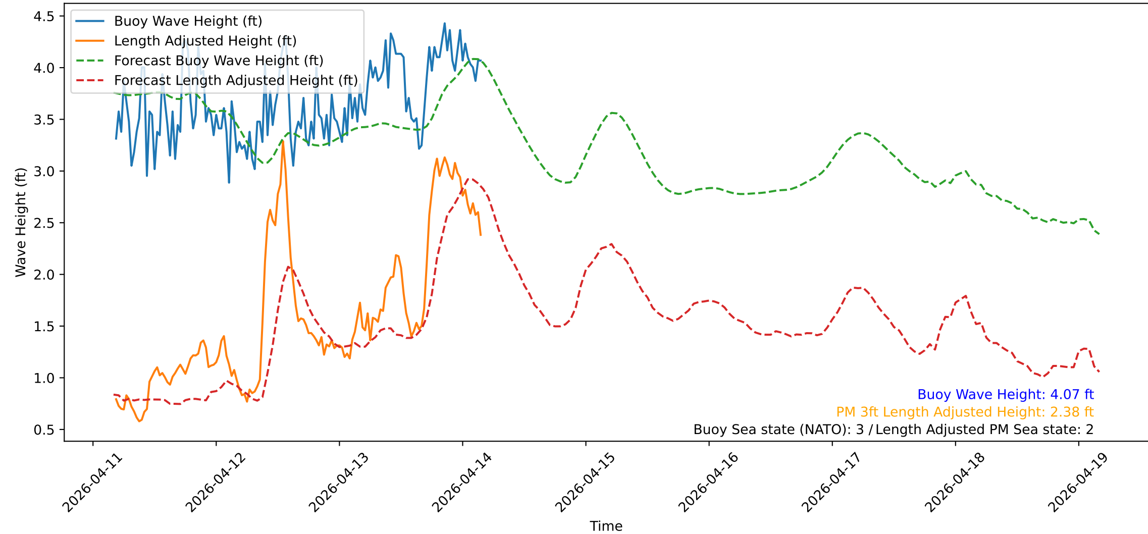
Wave Heights over Time for Red Beach at 2026-04-14 04:10:50
