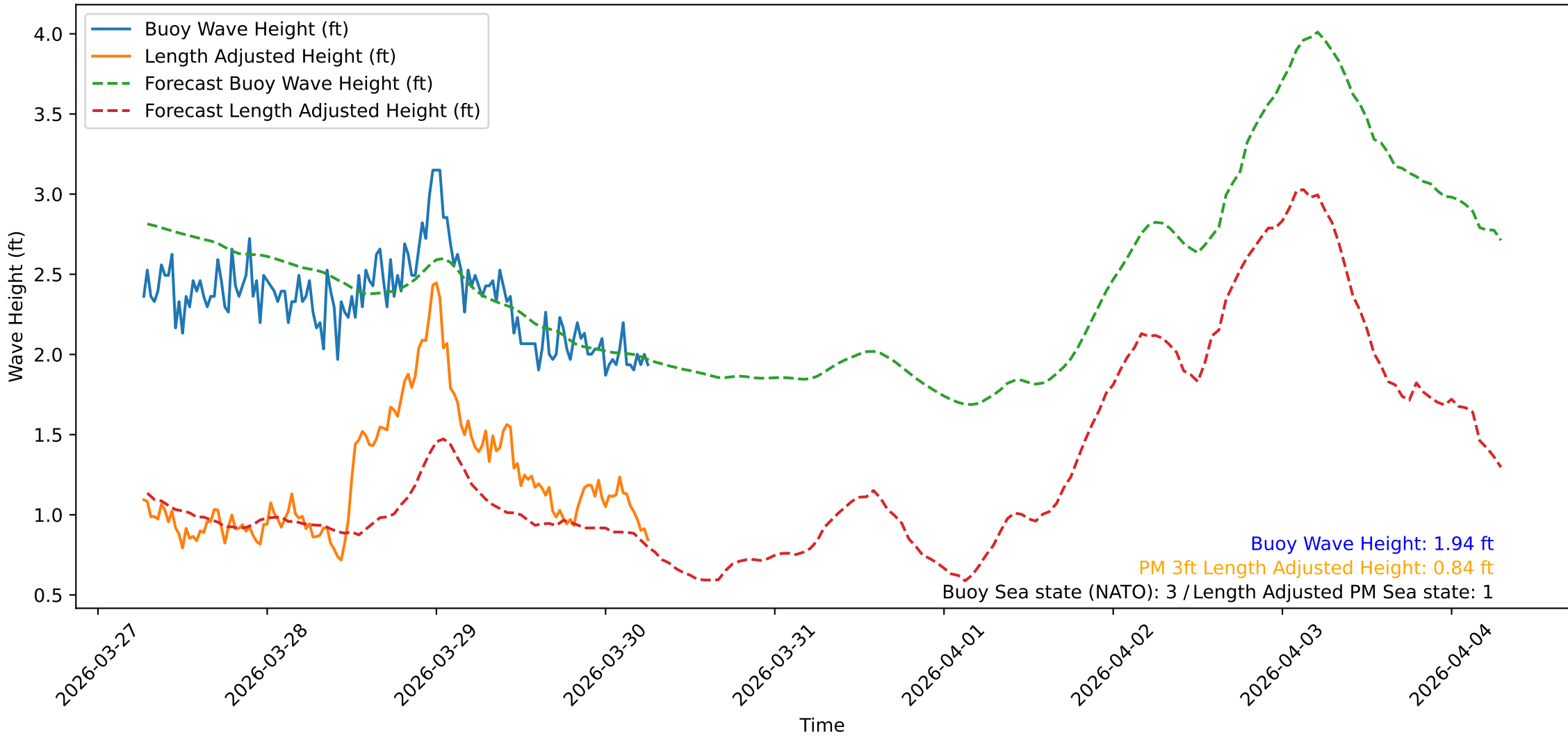
Wave Heights over Time for Oceanside Harbor at 2026-03-30 06:30:31
