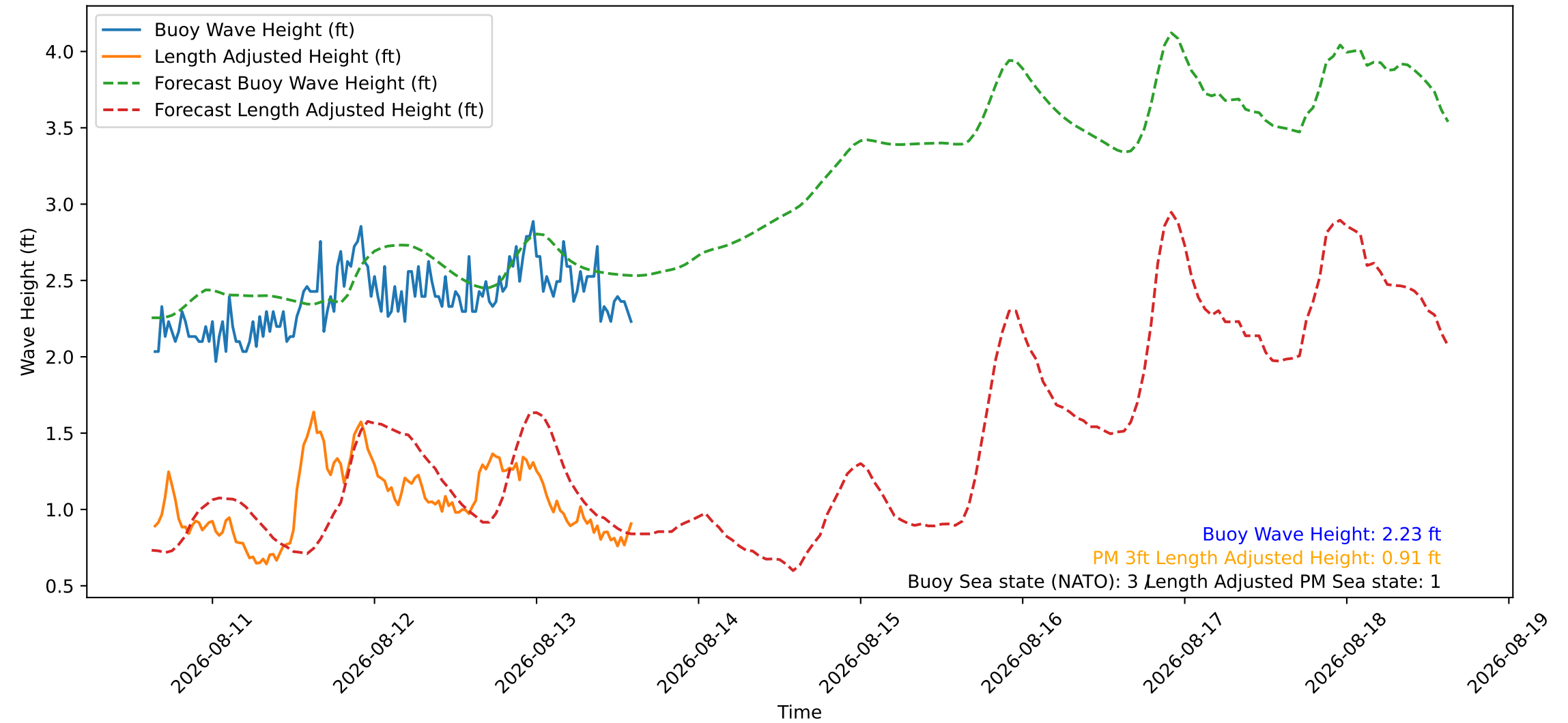
Wave Heights over Time for Red Beach at 2026-08-13 15:20:47
