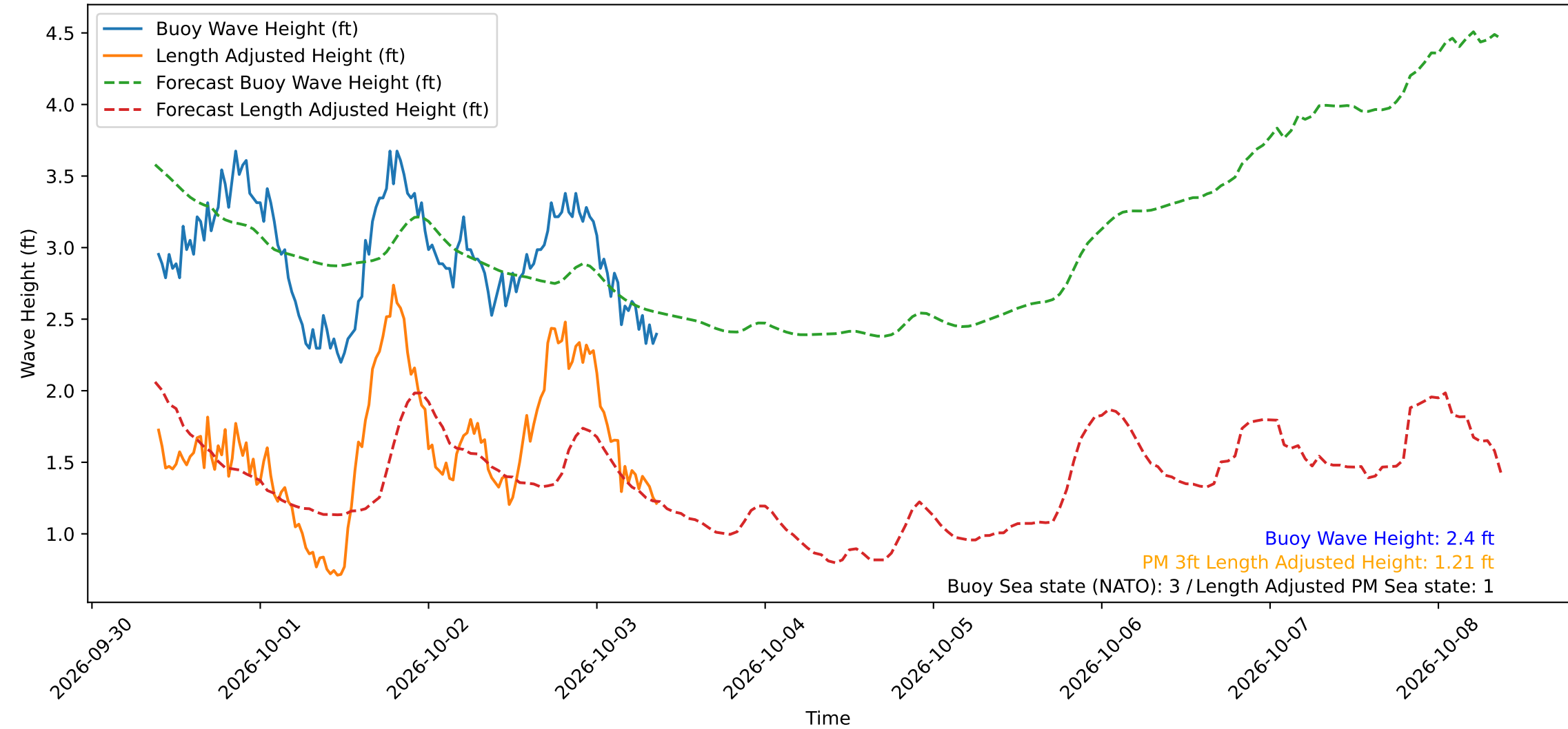
Wave Heights over Time for Green Beach at 2026-10-03 09:21:14
