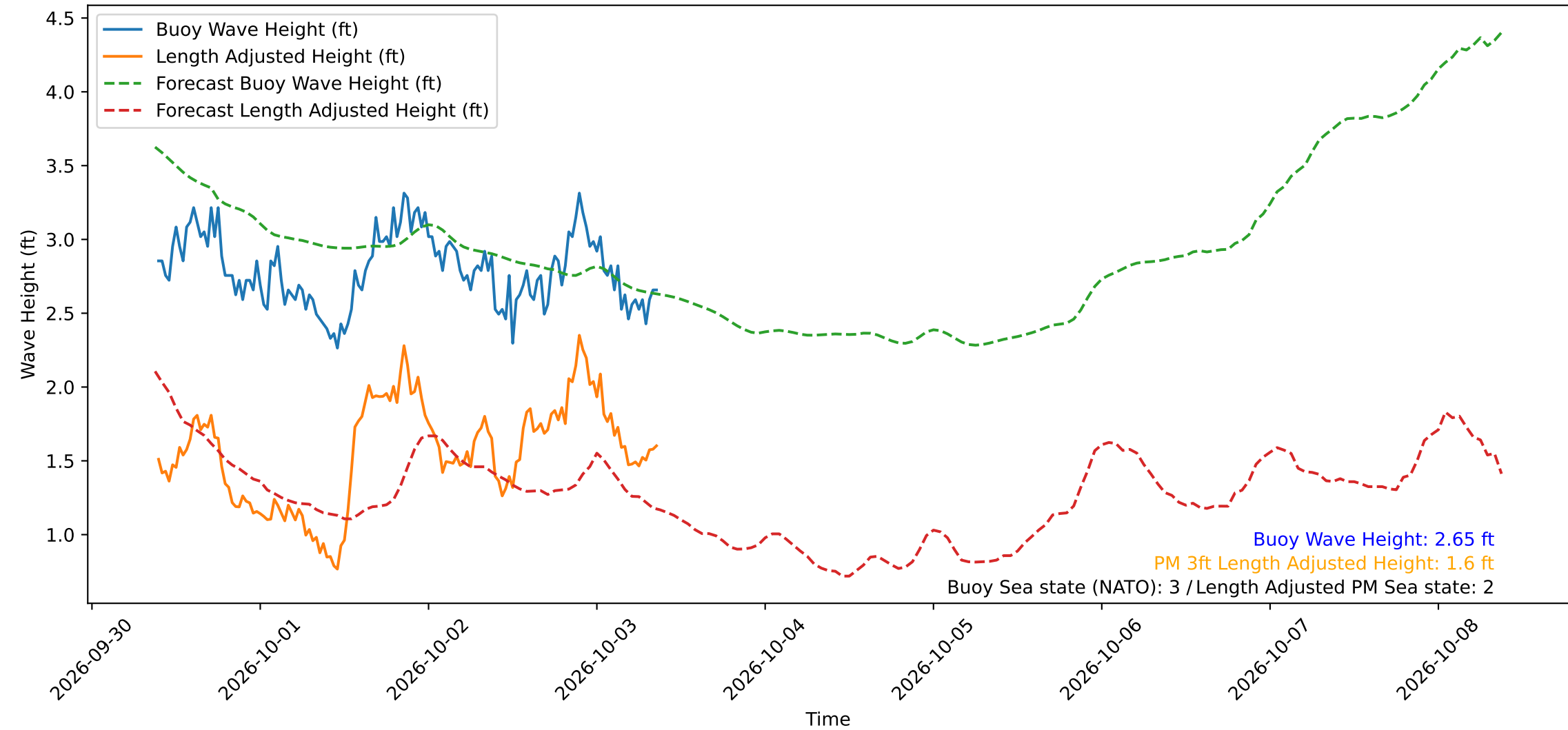
Wave Heights over Time for Oceanside Harbor at 2026-10-03 09:20:30
