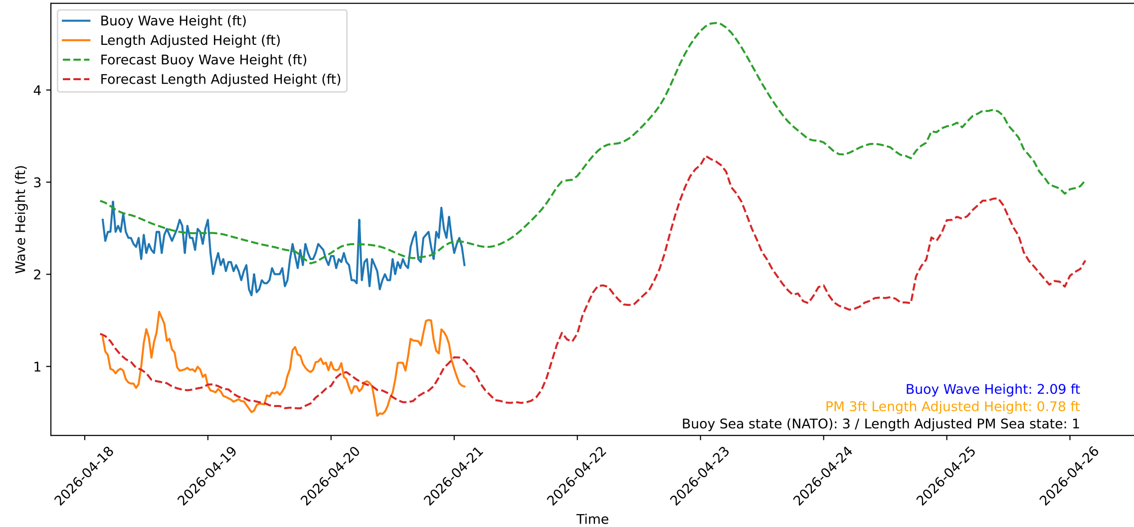
Wave Heights over Time for Red Beach at 2026-04-21 03:00:50
