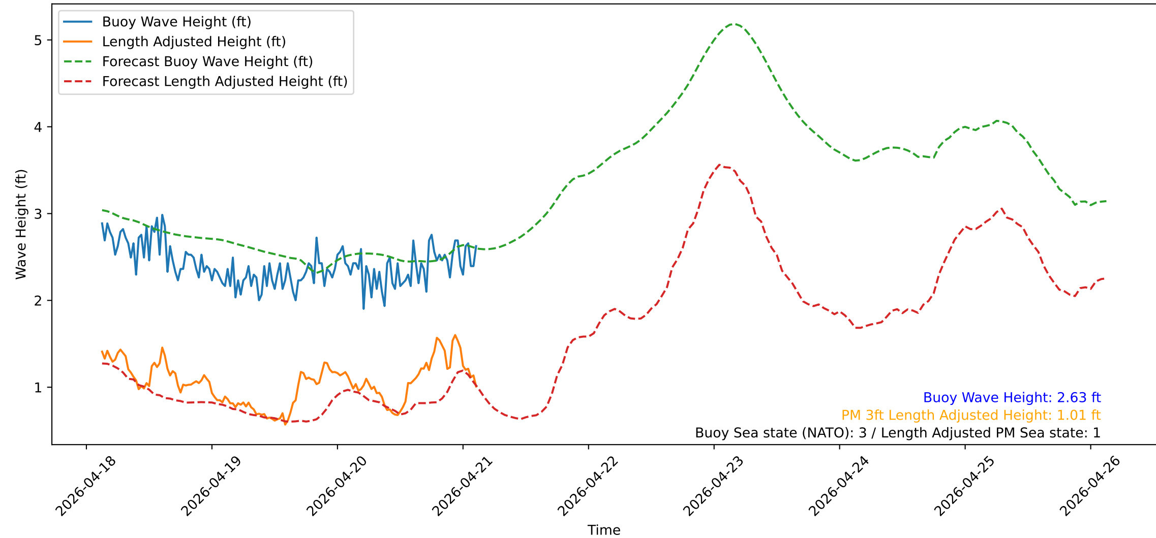
Wave Heights over Time for Oceanside Harbor at 2026-04-21 03:00:31
