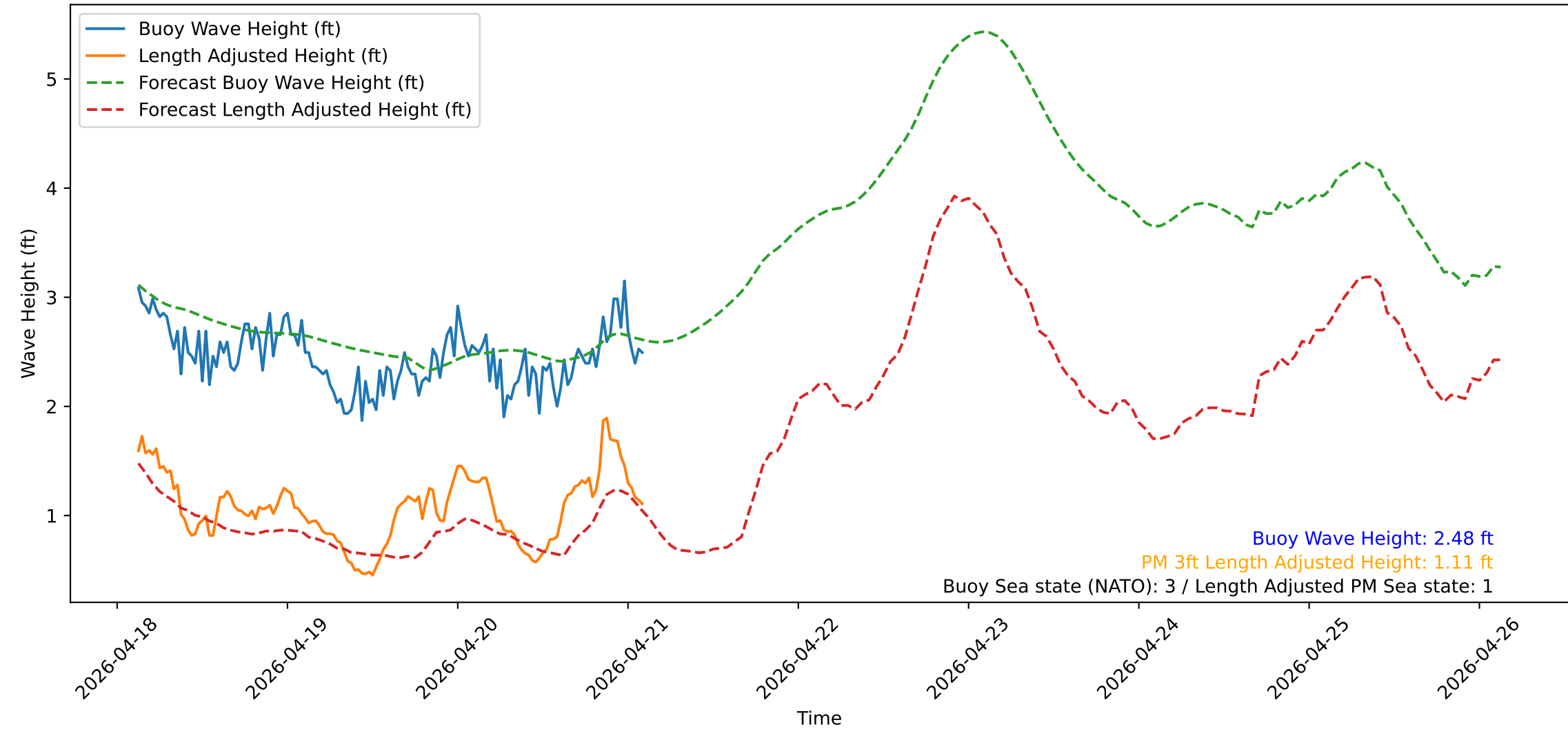
Wave Heights over Time for Green Beach at 2026-04-21 03:01:12
