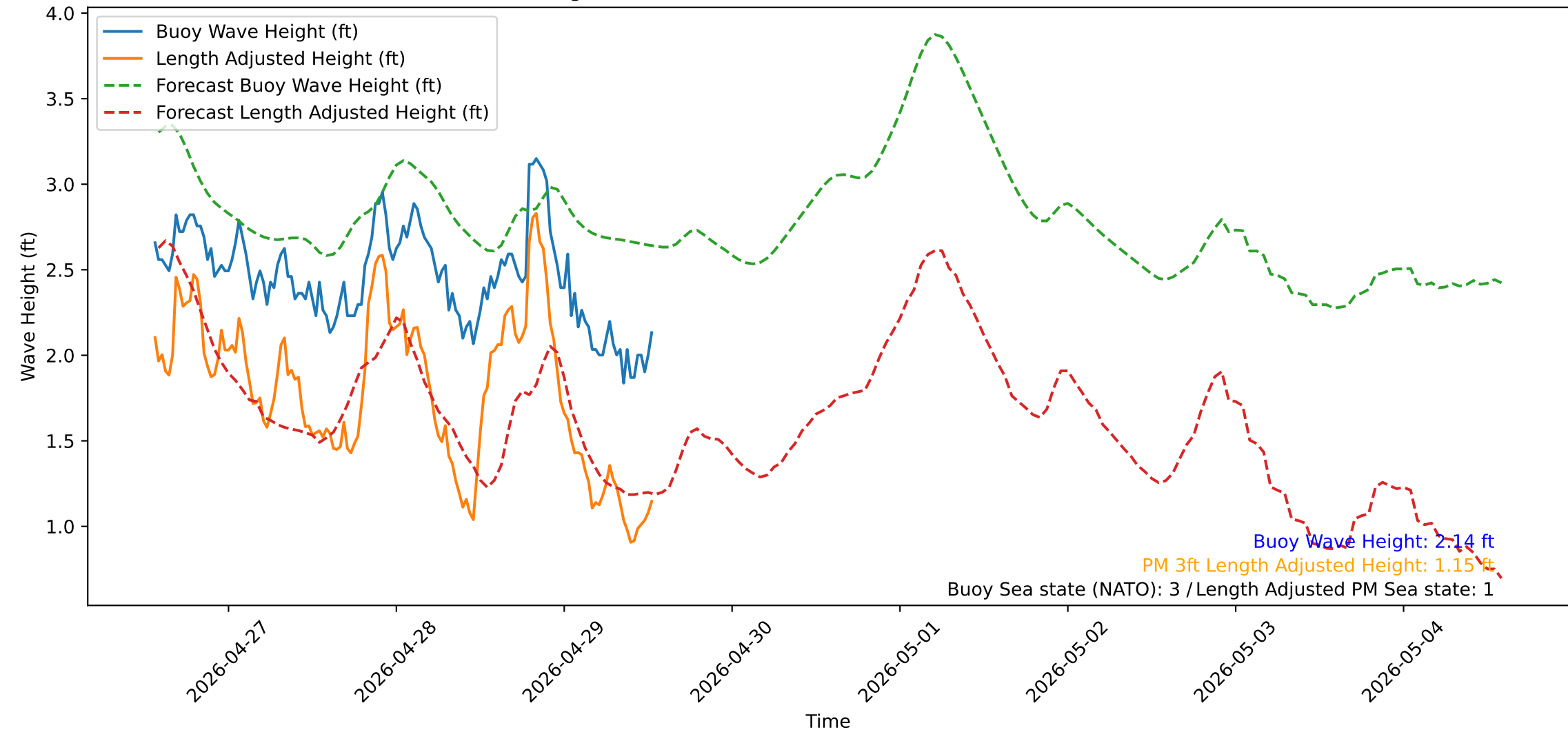
Wave Heights over Time for Green Beach at 2026-04-29 13:31:13
