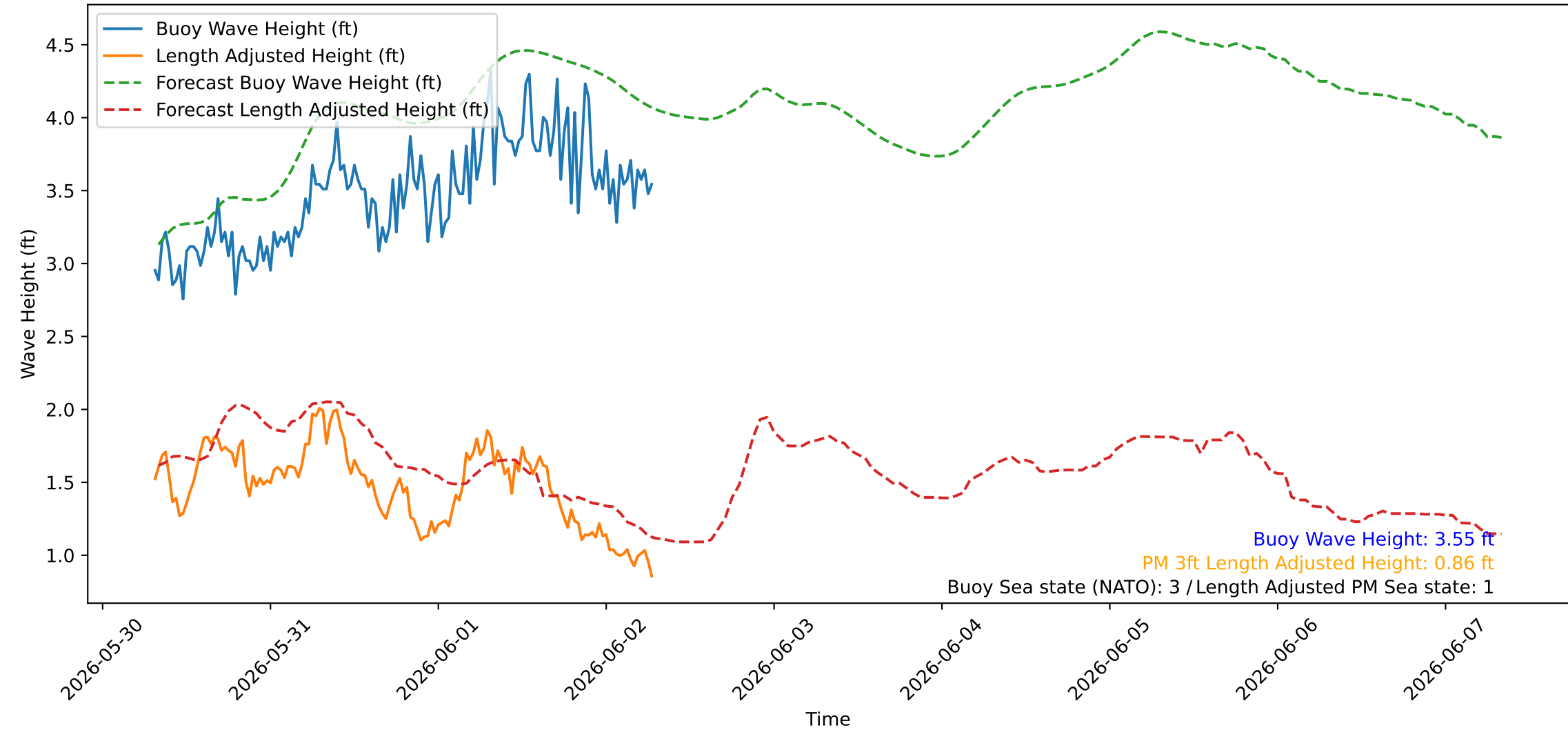
Wave Heights over Time for Green Beach at 2026-06-02 07:31:08
