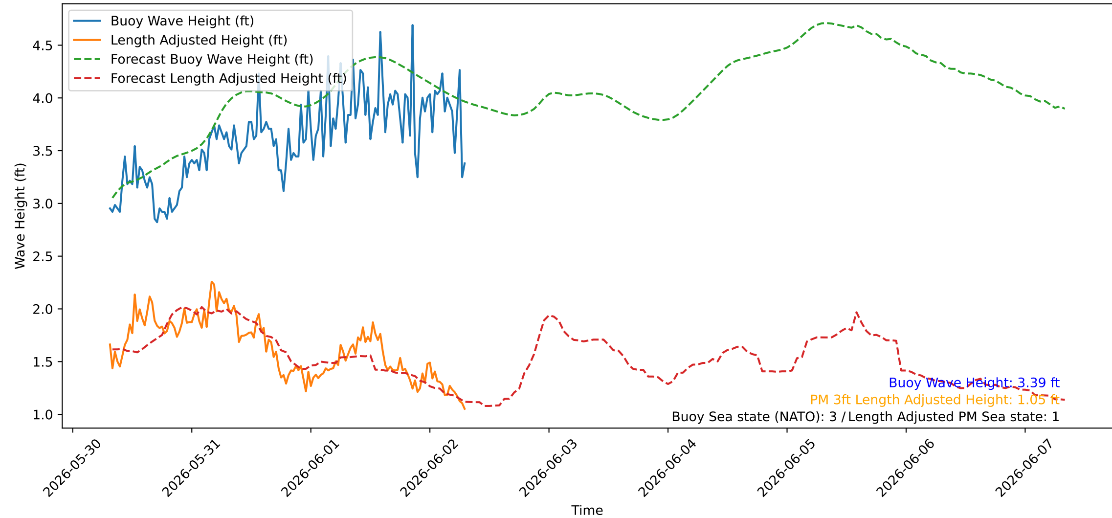
Wave Heights over Time for Oceanside Harbor at 2026-06-02 07:30:27
