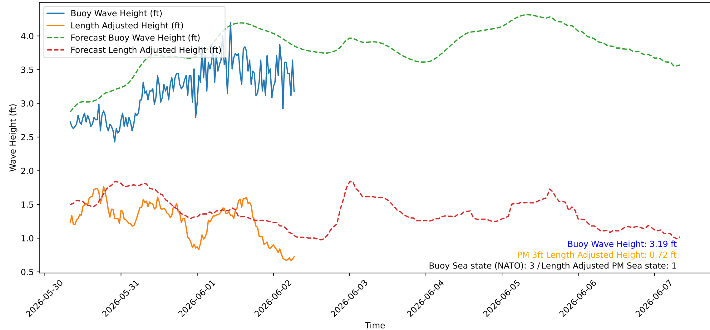
Wave Heights over Time for Red Beach at 2026-06-02 07:30:46
