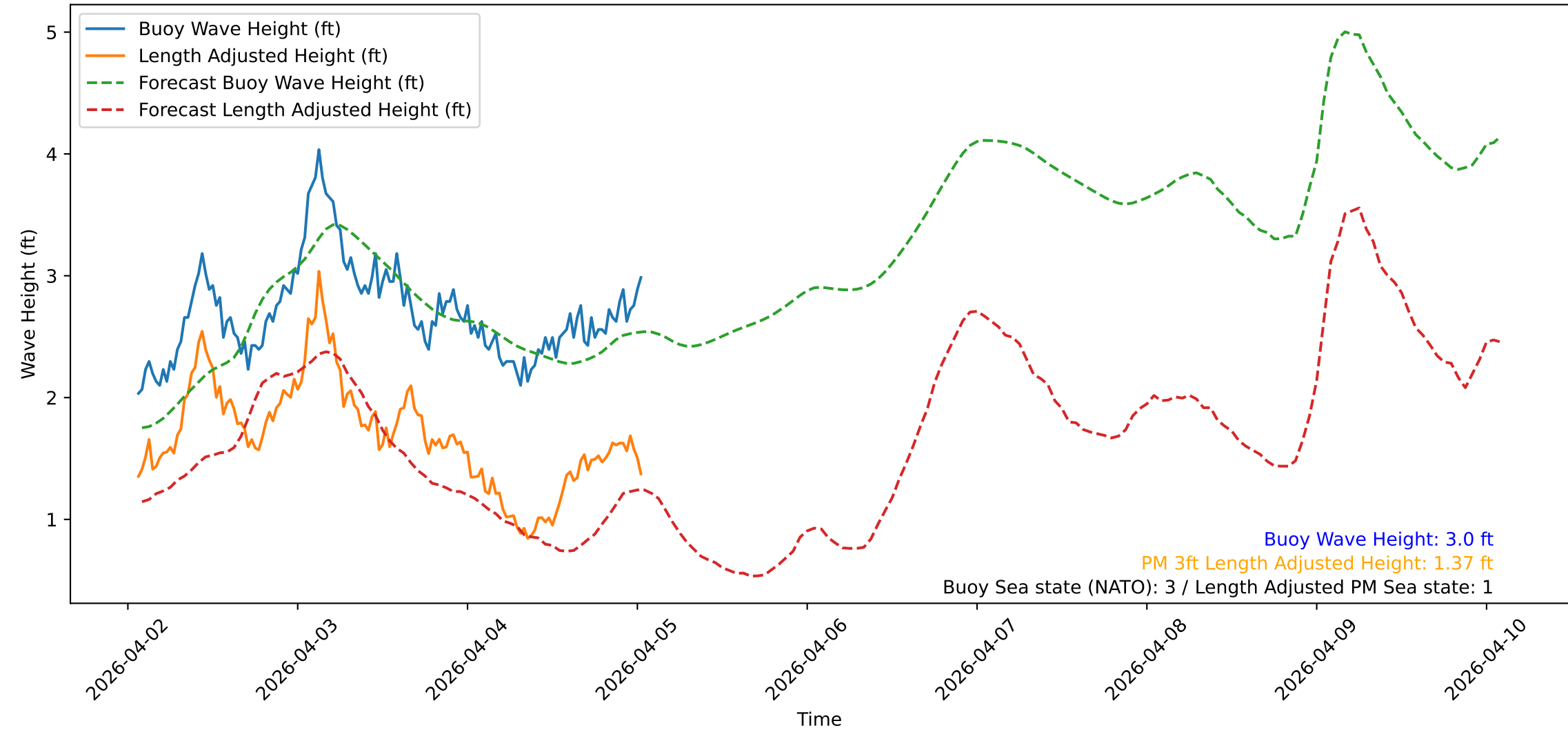
Wave Heights over Time for Oceanside Harbor at 2026-04-05 01:40:32
