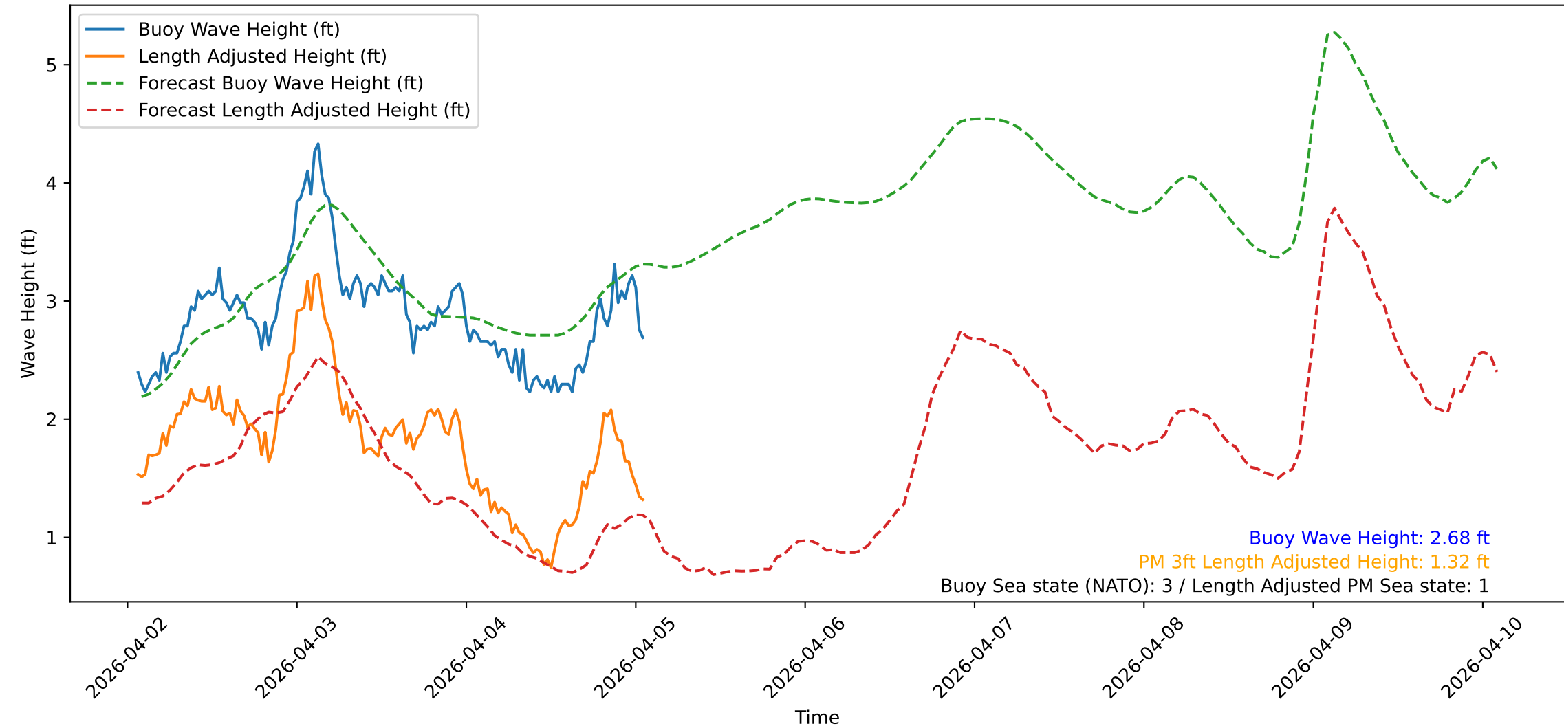
Wave Heights over Time for Green Beach at 2026-04-05 01:41:11
