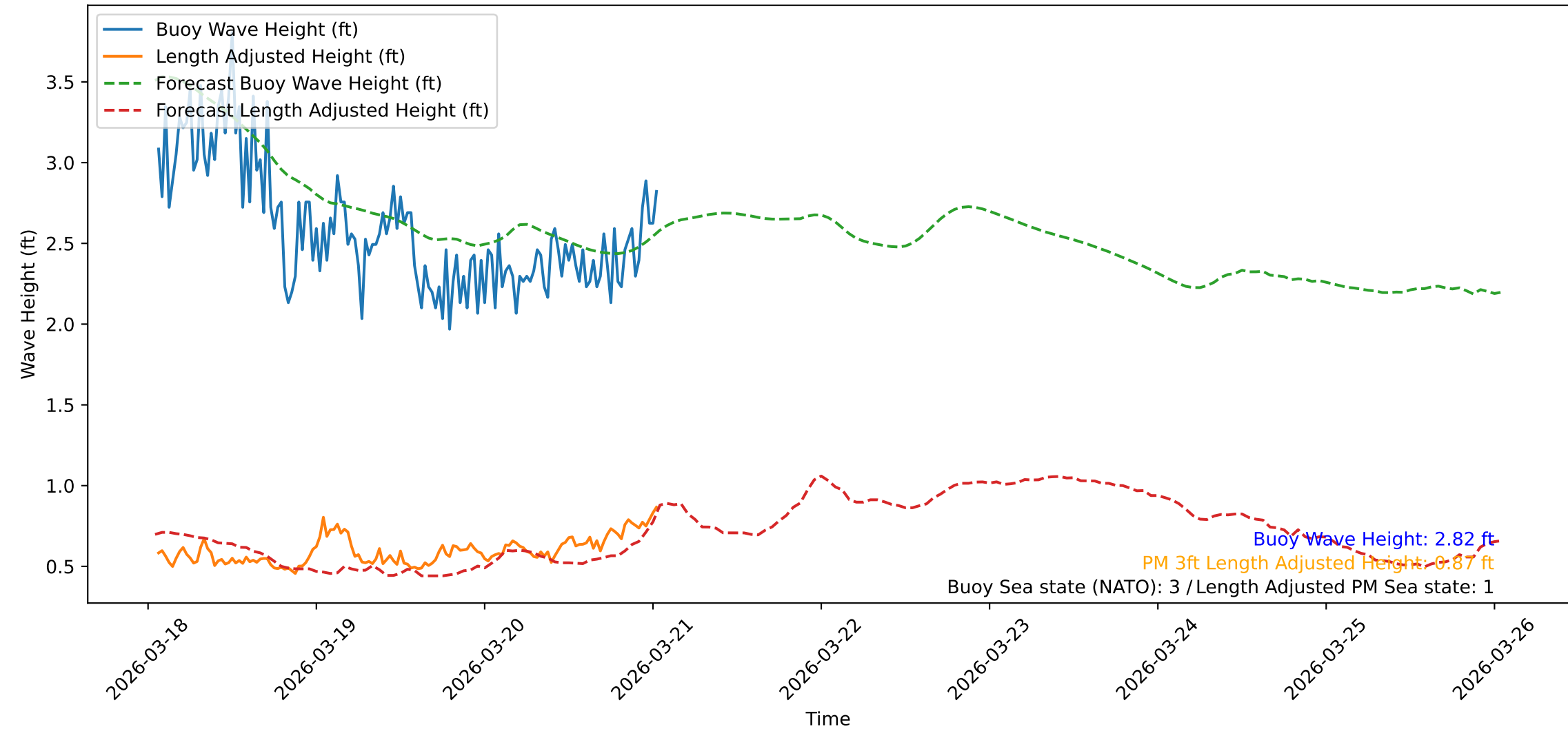
Wave Heights over Time for Oceanside Harbor at 2026-03-21 01:20:32
