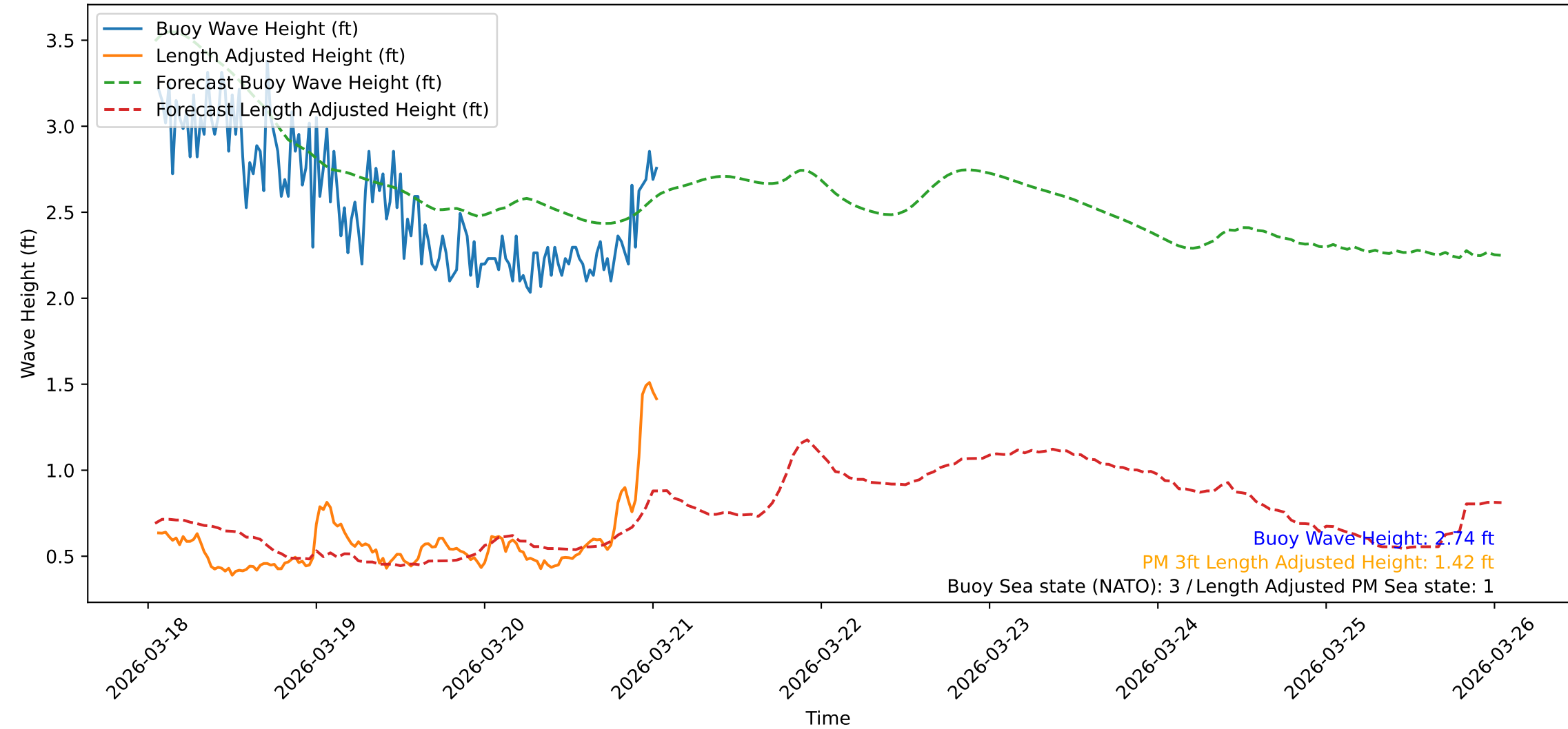
Wave Heights over Time for Green Beach at 2026-03-21 01:21:11
