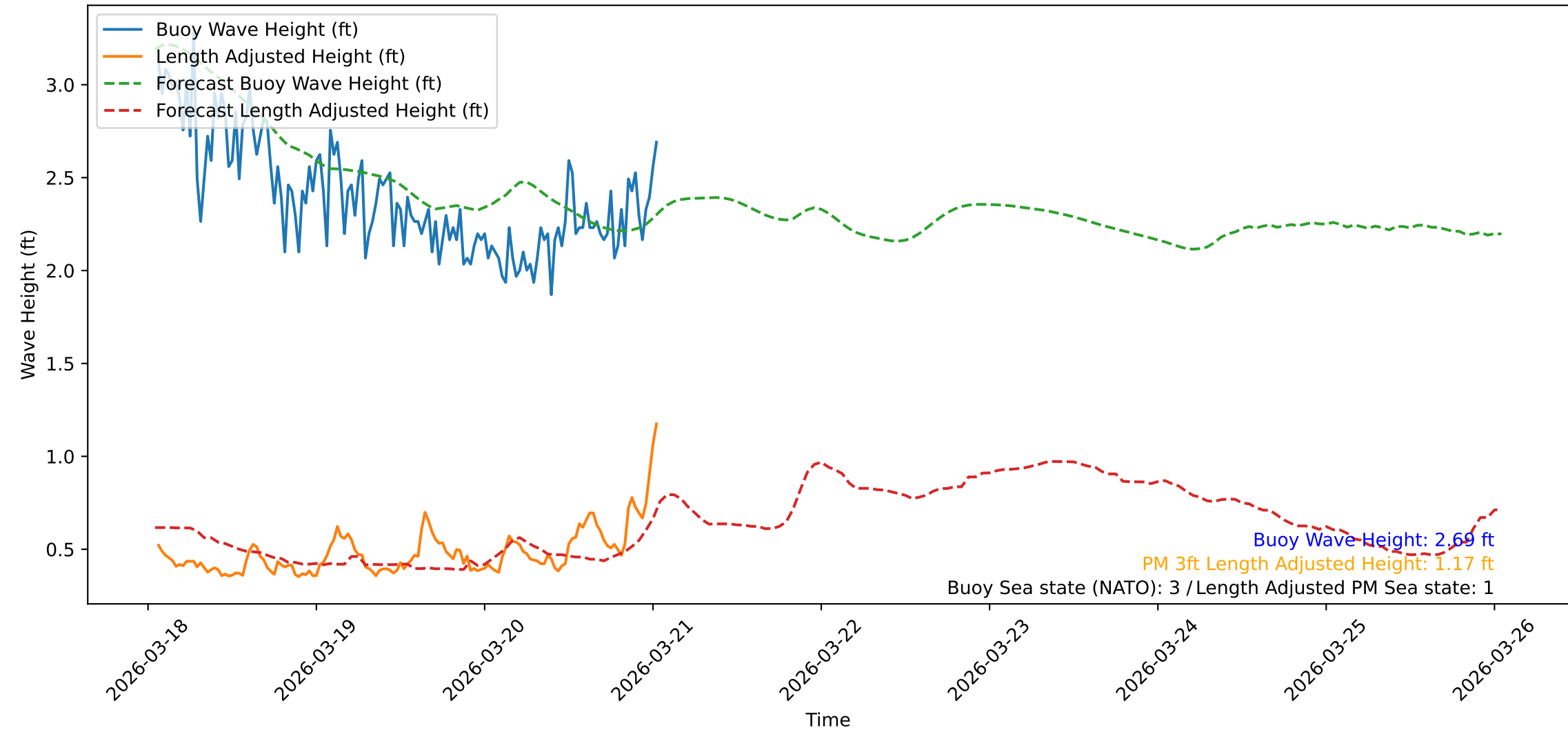
Wave Heights over Time for Red Beach at 2026-03-21 01:20:48
