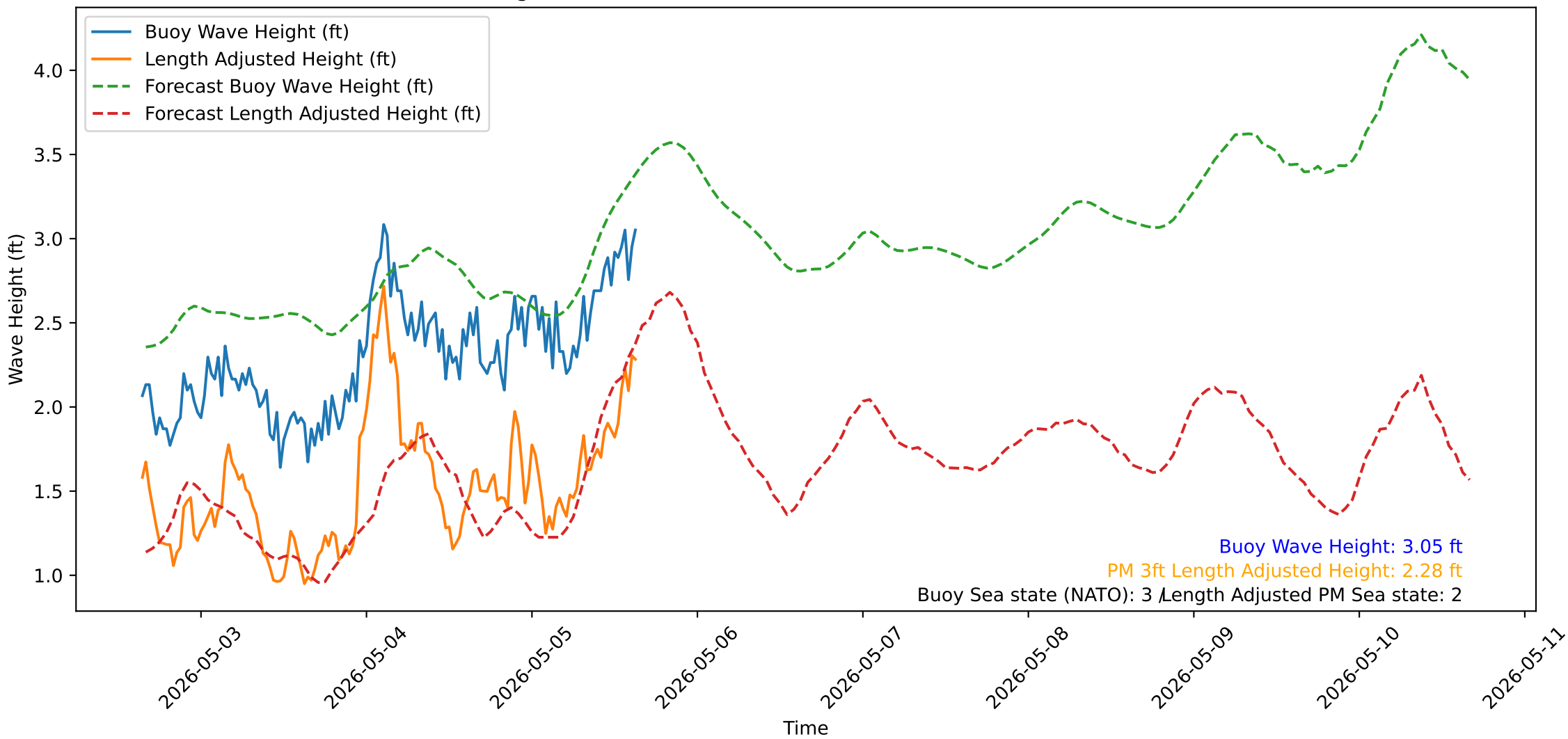
Wave Heights over Time for Oceanside Harbor at 2026-05-05 15:30:31
