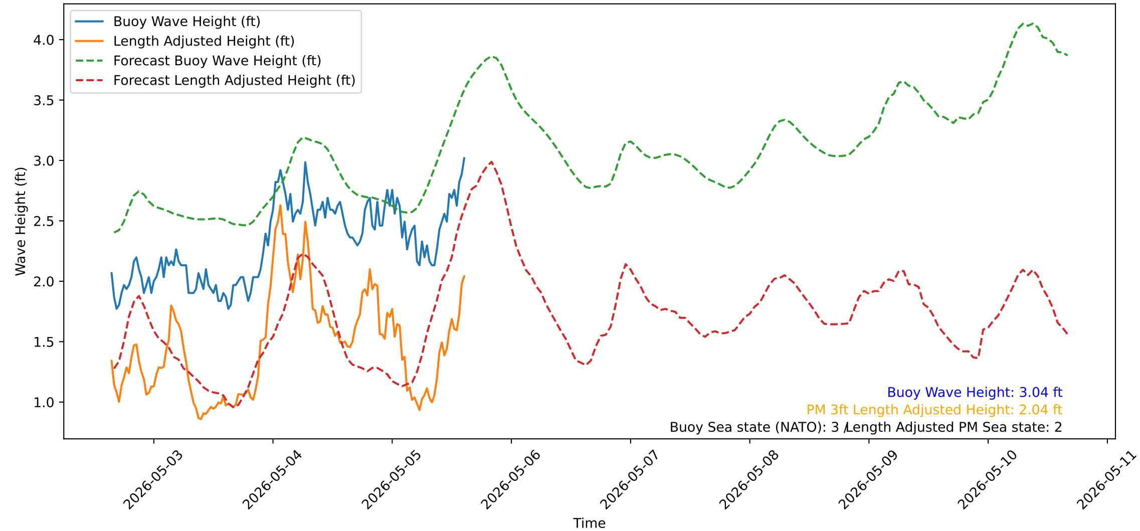
Wave Heights over Time for Green Beach at 2026-05-05 15:31:12
