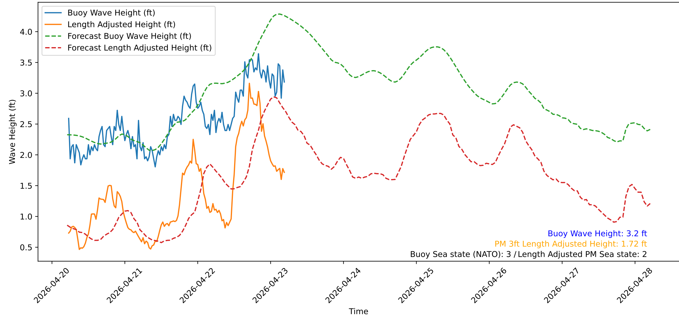
Wave Heights over Time for Red Beach at 2026-04-23 05:20:51
