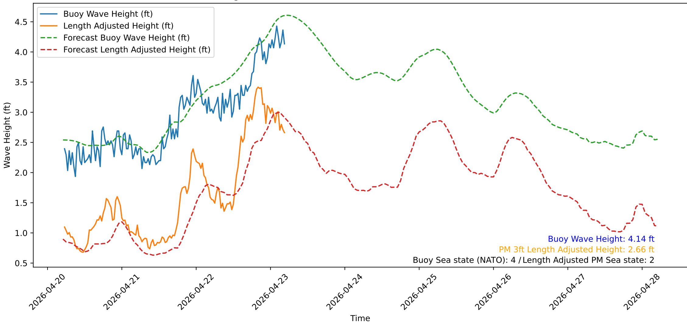
Wave Heights over Time for Oceanside Harbor at 2026-04-23 05:20:31
