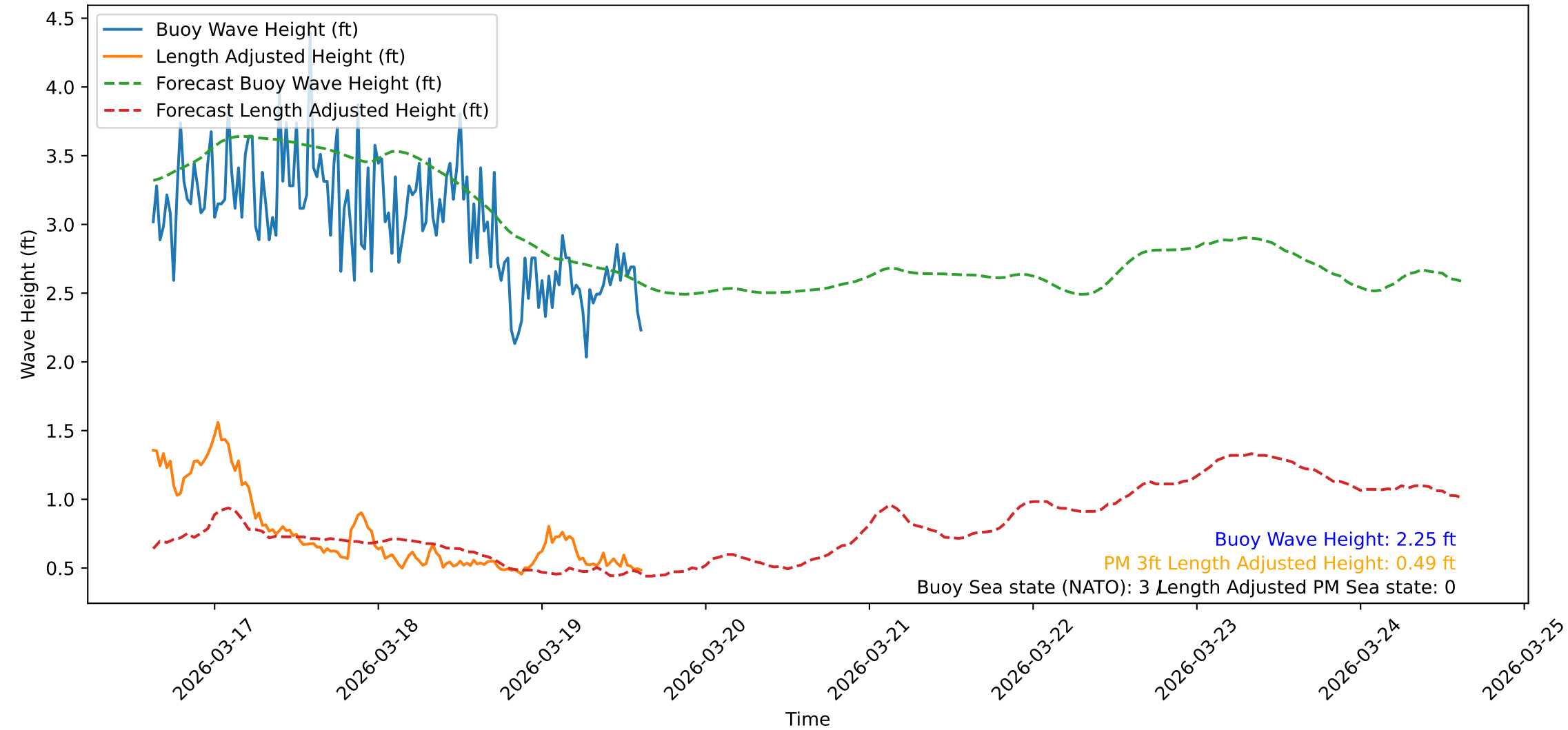
Wave Heights over Time for Oceanside Harbor at 2026-03-19 15:00:31
