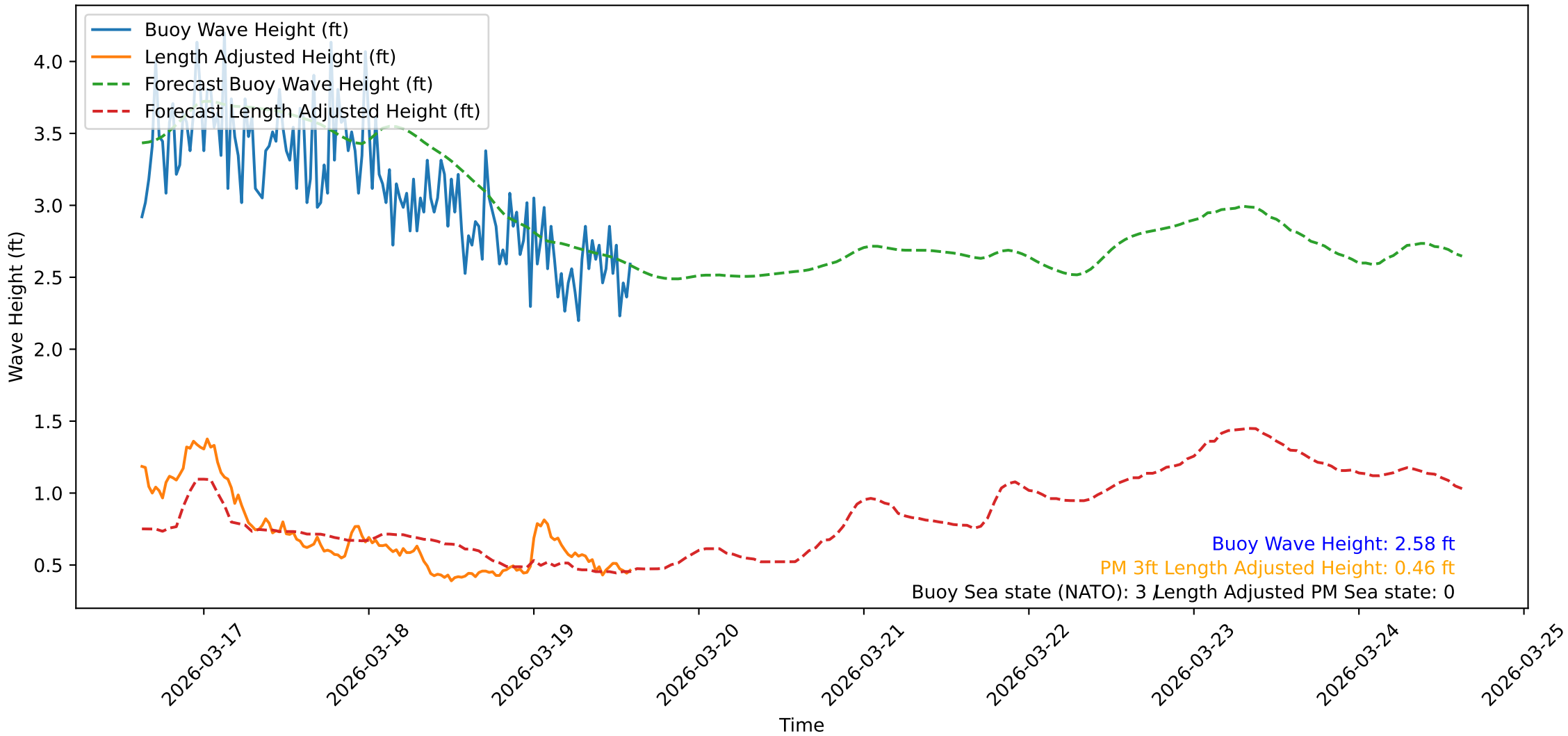
Wave Heights over Time for Green Beach at 2026-03-19 15:01:10
