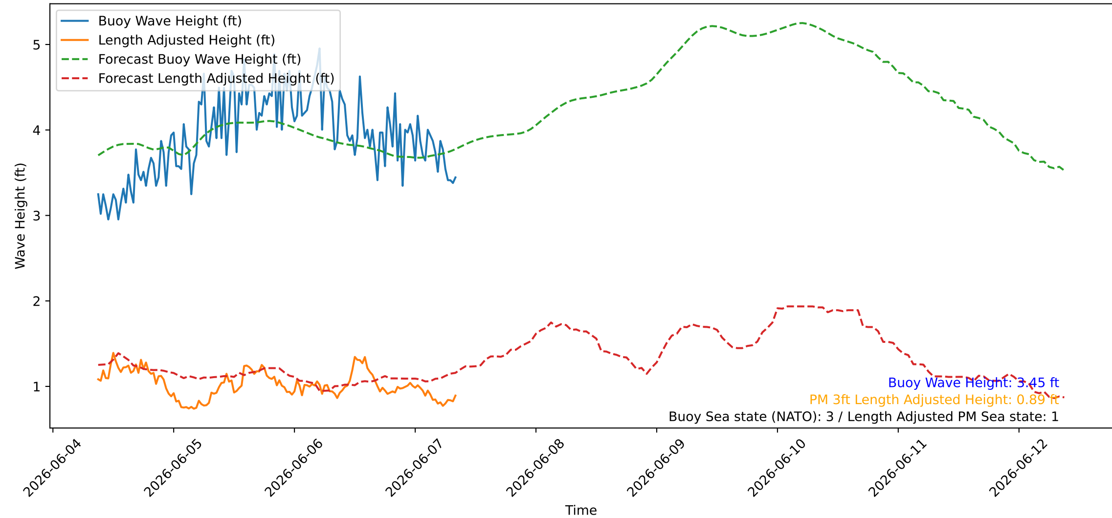
Wave Heights over Time for Red Beach at 2026-06-07 08:40:45
