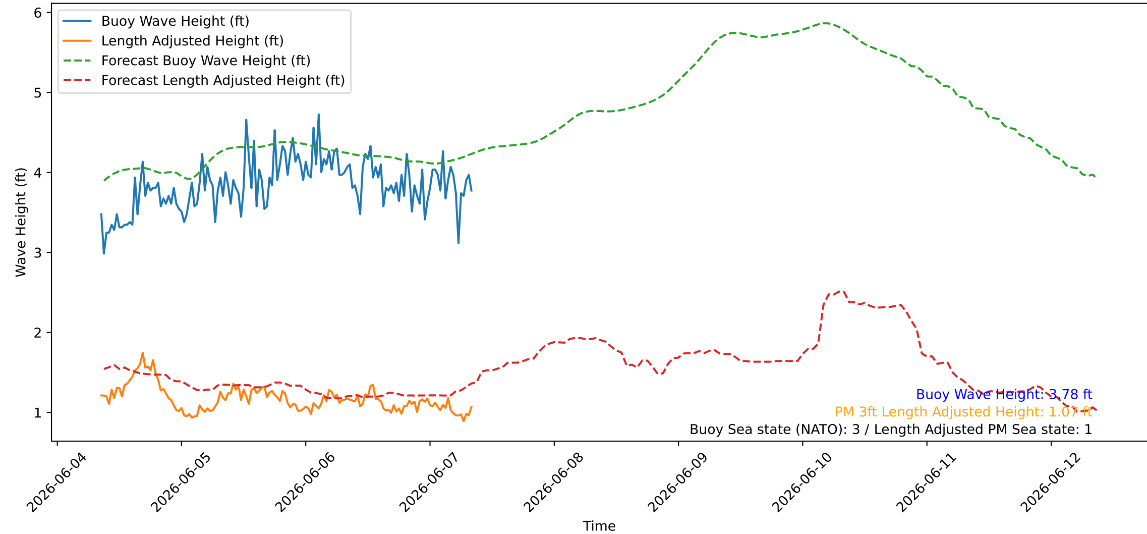
Wave Heights over Time for Green Beach at 2026-06-07 08:41:08
