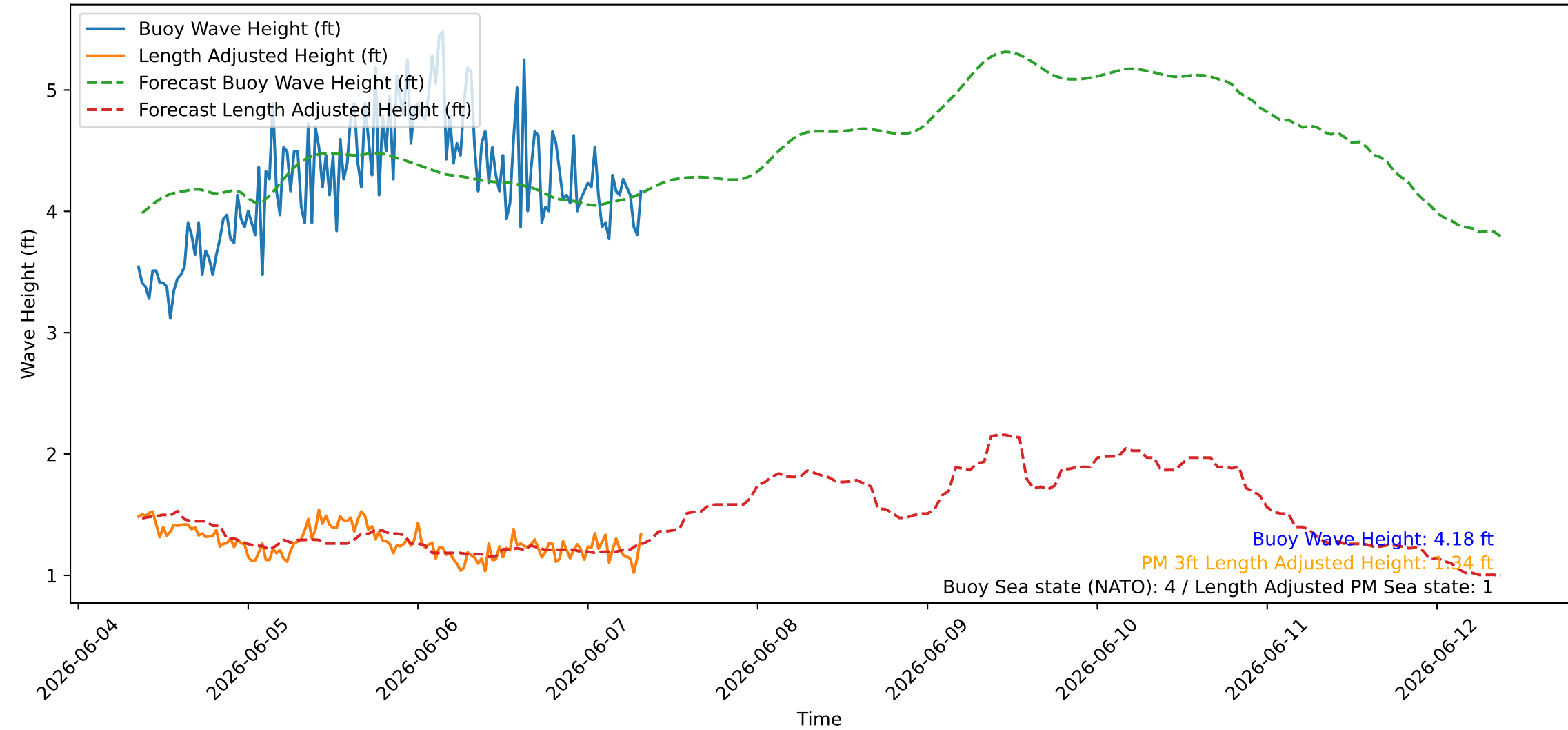
Wave Heights over Time for Oceanside Harbor at 2026-06-07 08:40:26
