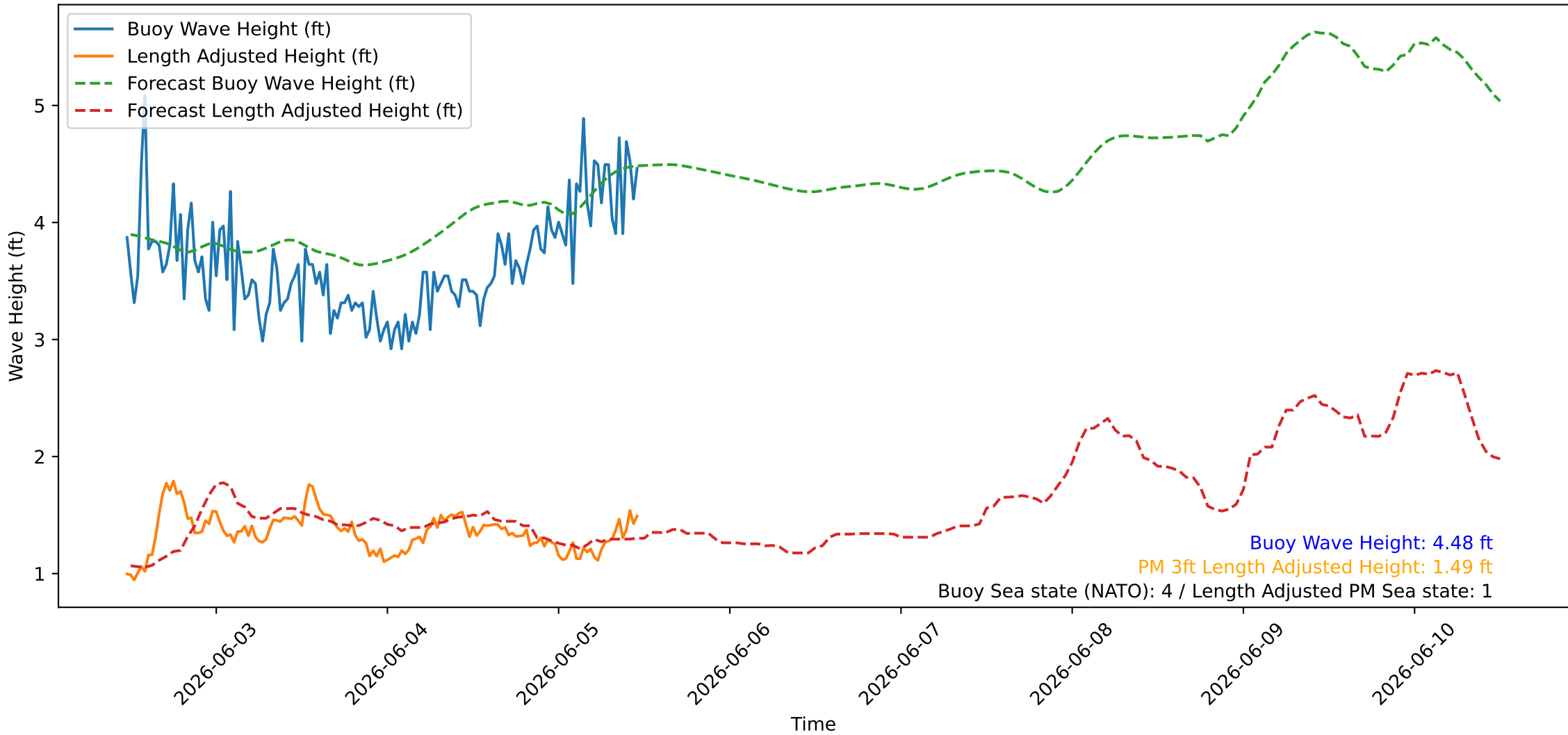
Wave Heights over Time for Oceanside Harbor at 2026-06-05 11:40:26
