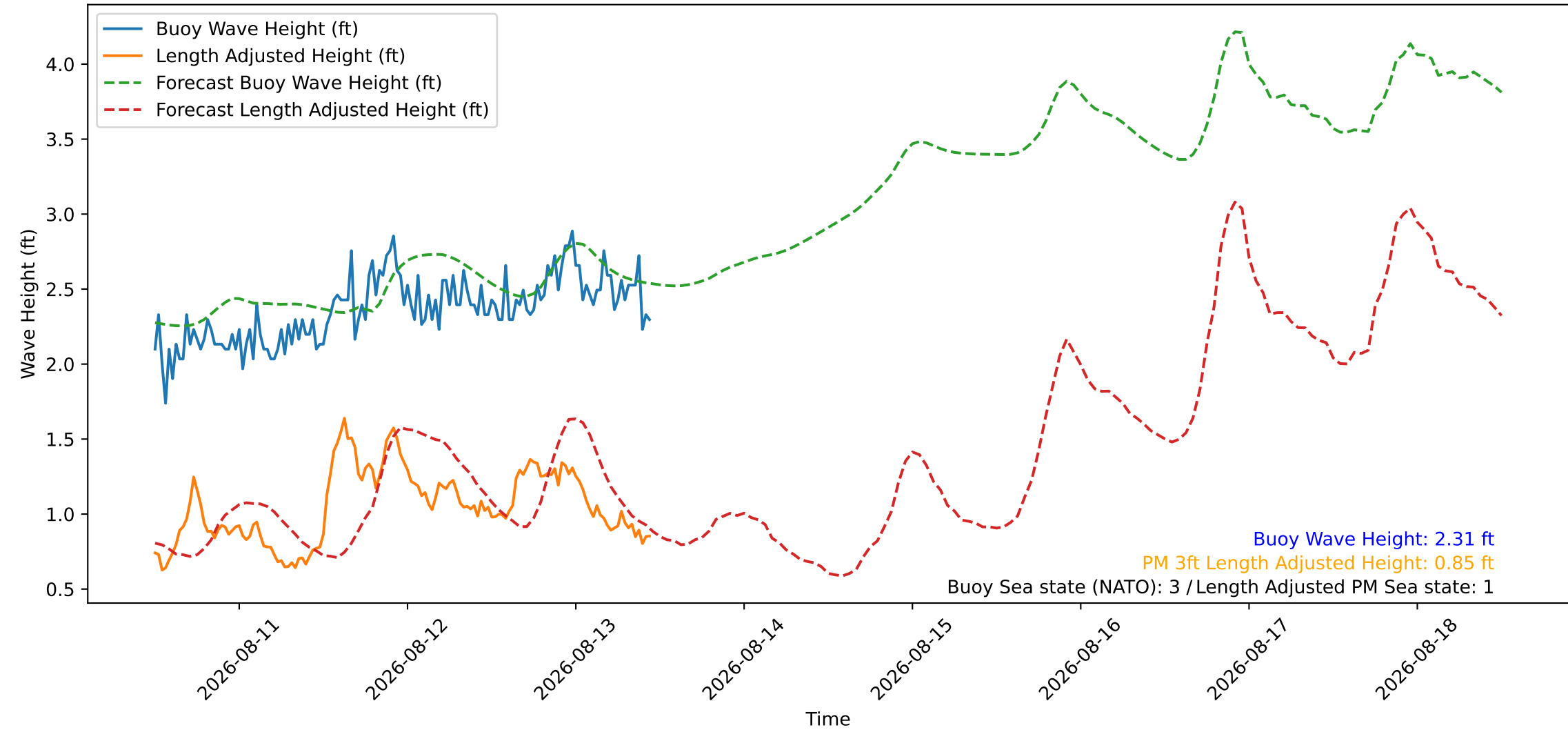
Wave Heights over Time for Red Beach at 2026-08-13 11:50:47
