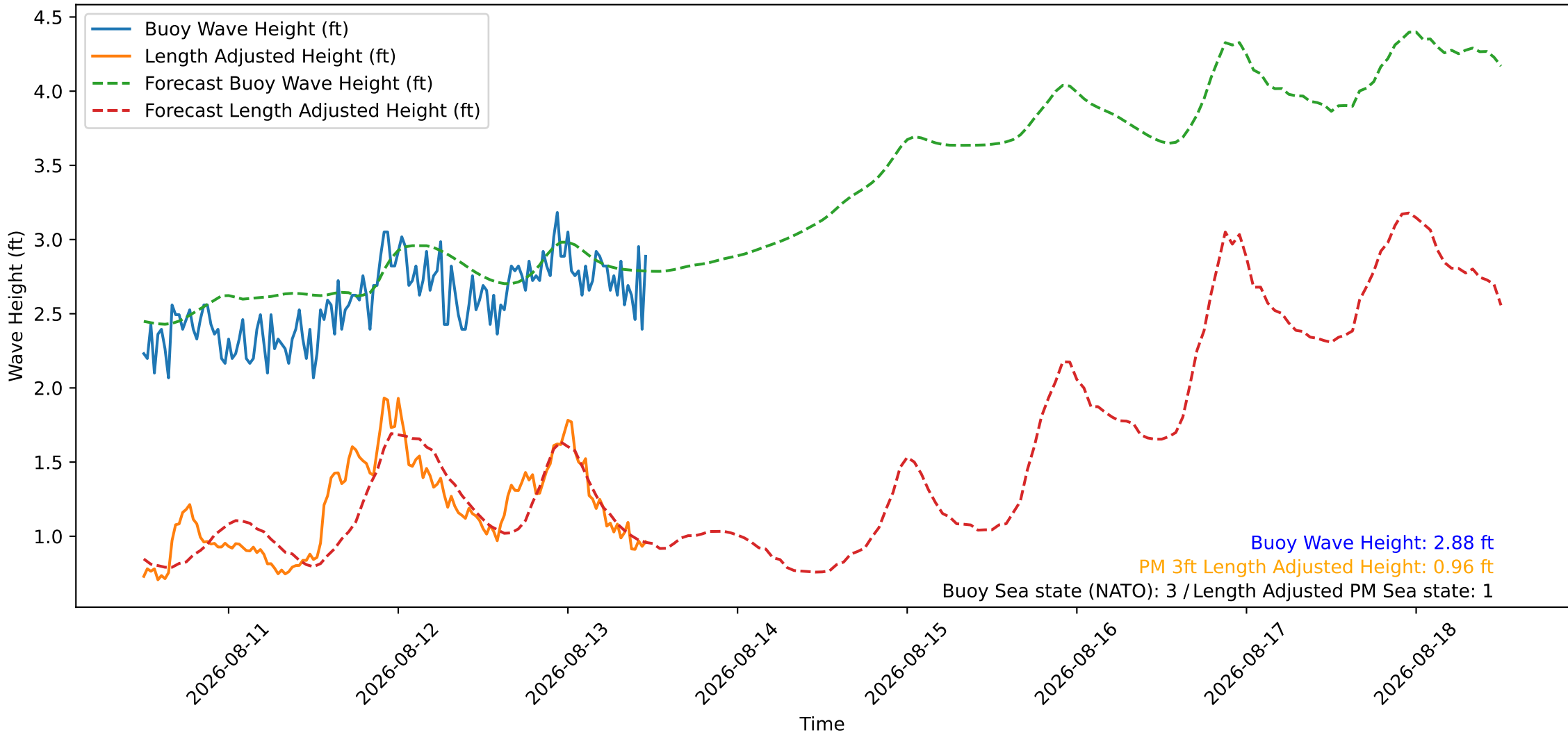
Wave Heights over Time for Oceanside Harbor at 2026-08-13 11:50:26
