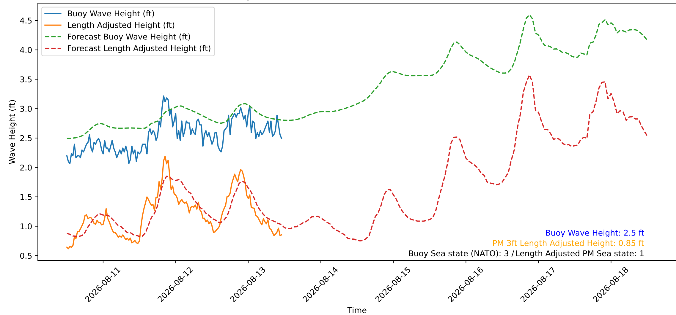
Wave Heights over Time for Green Beach at 2026-08-13 11:51:09
