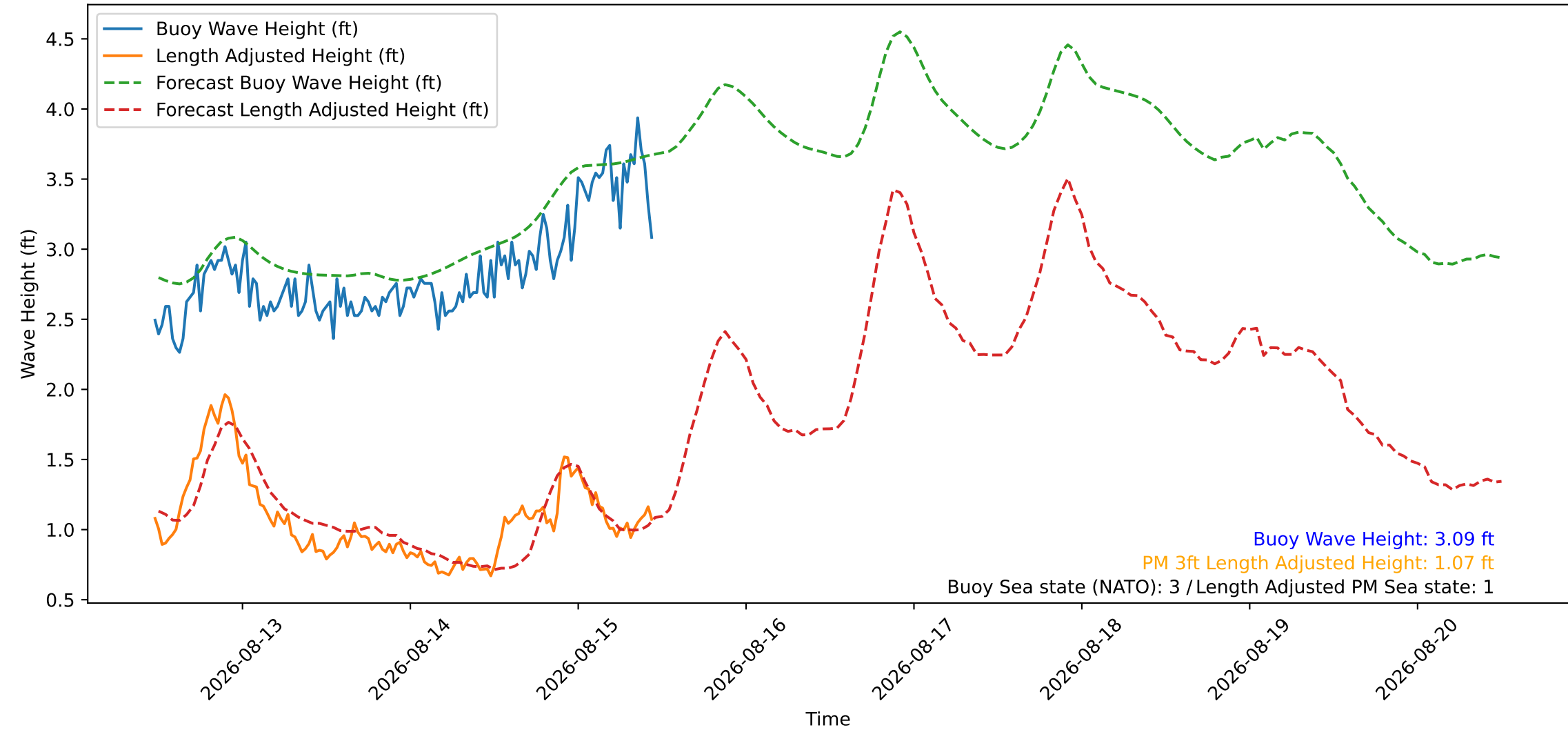
Wave Heights over Time for Green Beach at 2026-08-15 11:31:09
