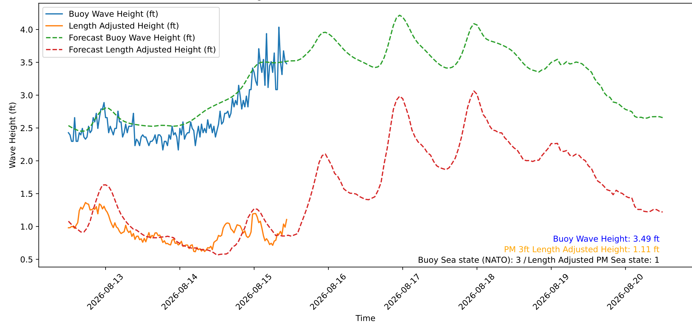
Wave Heights over Time for Red Beach at 2026-08-15 11:30:46
