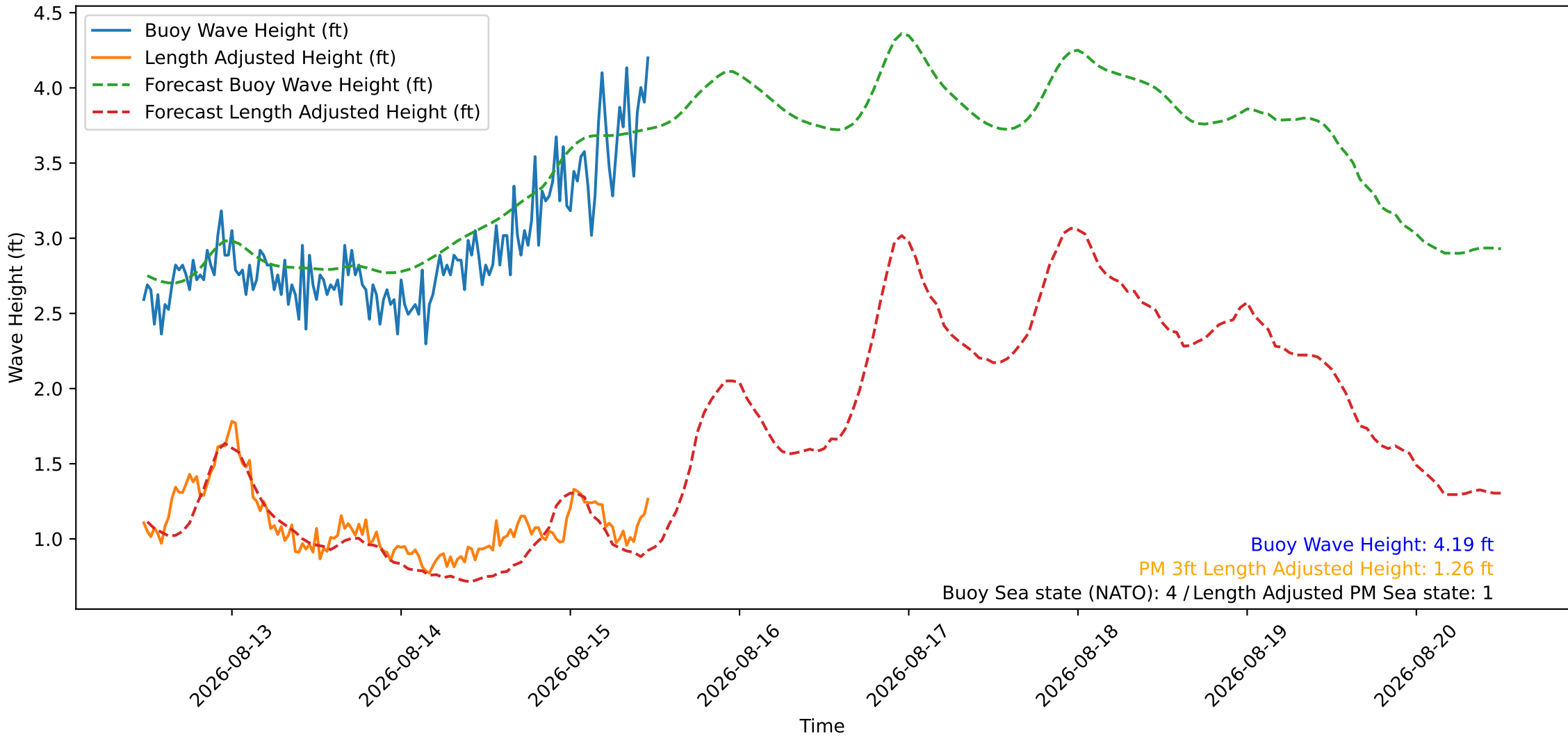
Wave Heights over Time for Oceanside Harbor at 2026-08-15 11:30:27
