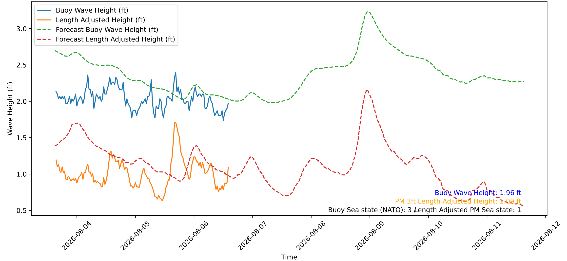
Wave Heights over Time for Red Beach at 2026-08-06 15:10:45
