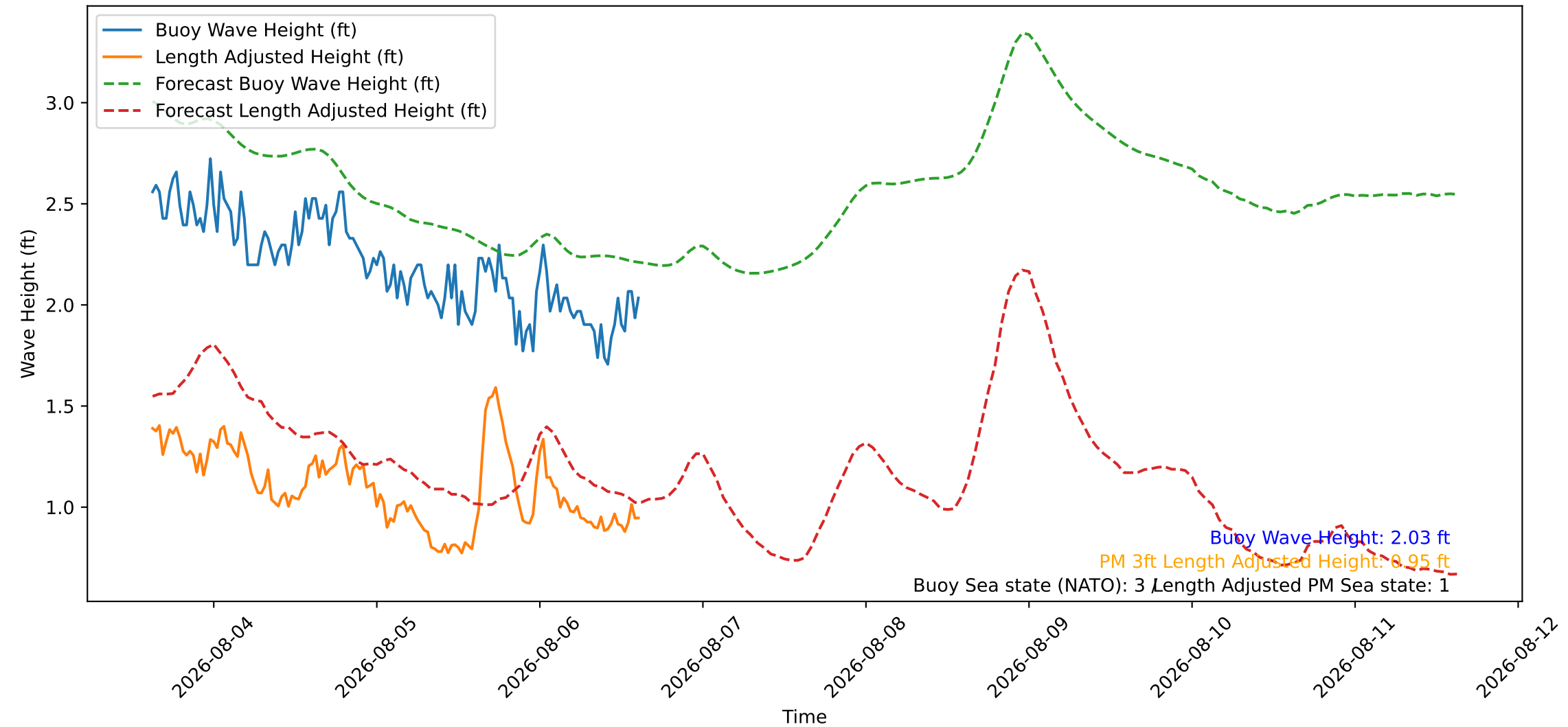
Wave Heights over Time for Oceanside Harbor at 2026-08-06 15:10:26
