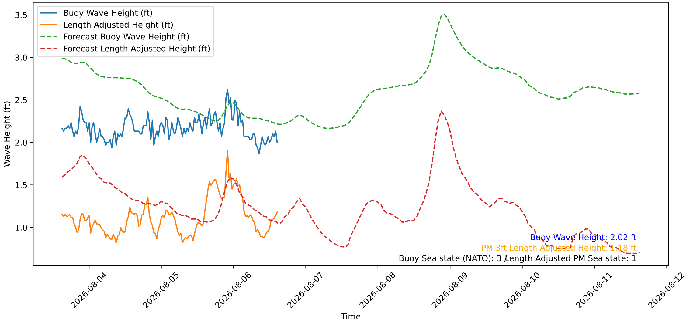
Wave Heights over Time for Green Beach at 2026-08-06 15:11:07
