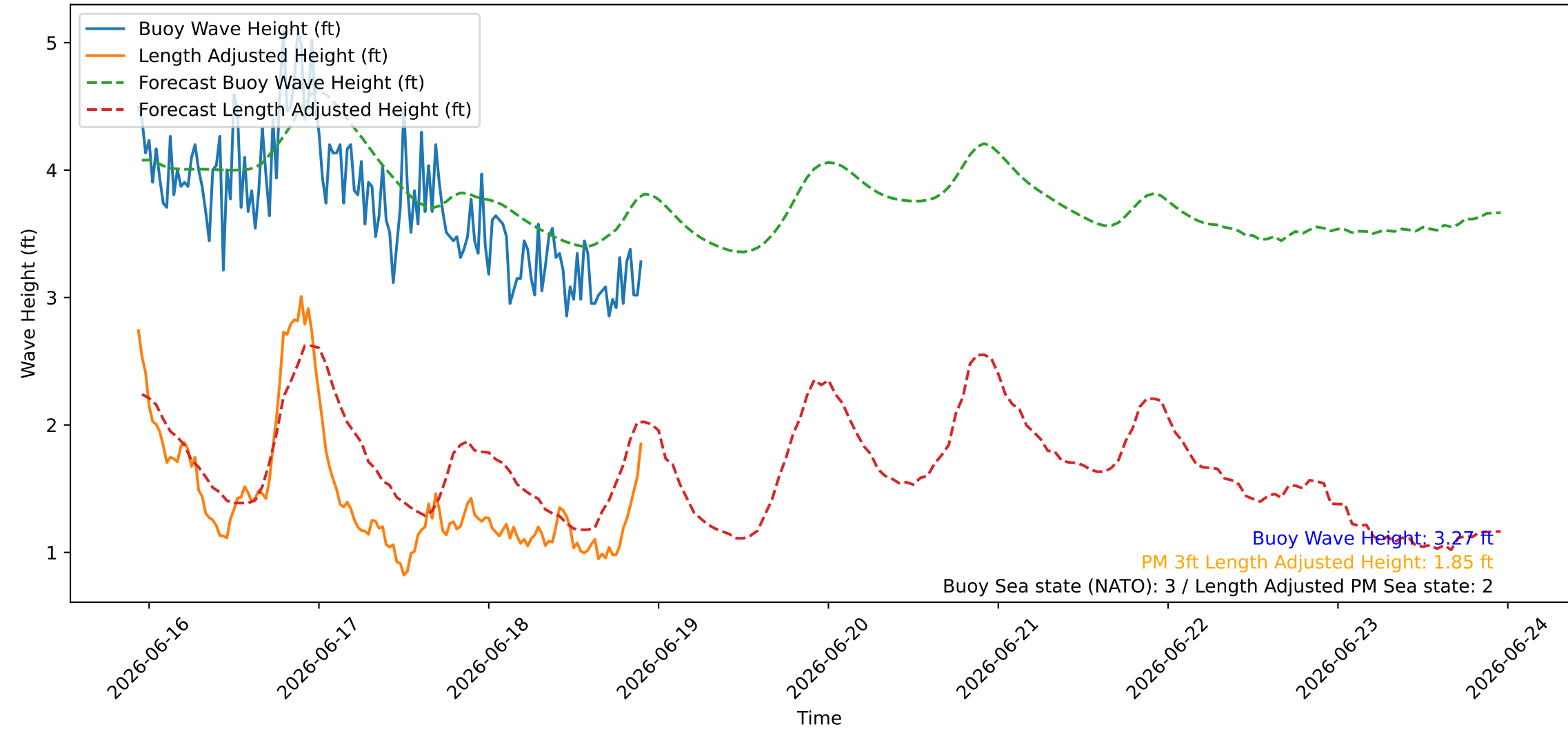
Wave Heights over Time for Green Beach at 2026-06-18 22:31:08
