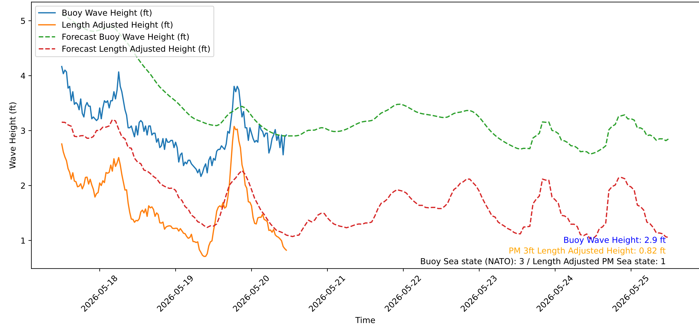
Wave Heights over Time for Green Beach at 2026-05-20 11:51:14
