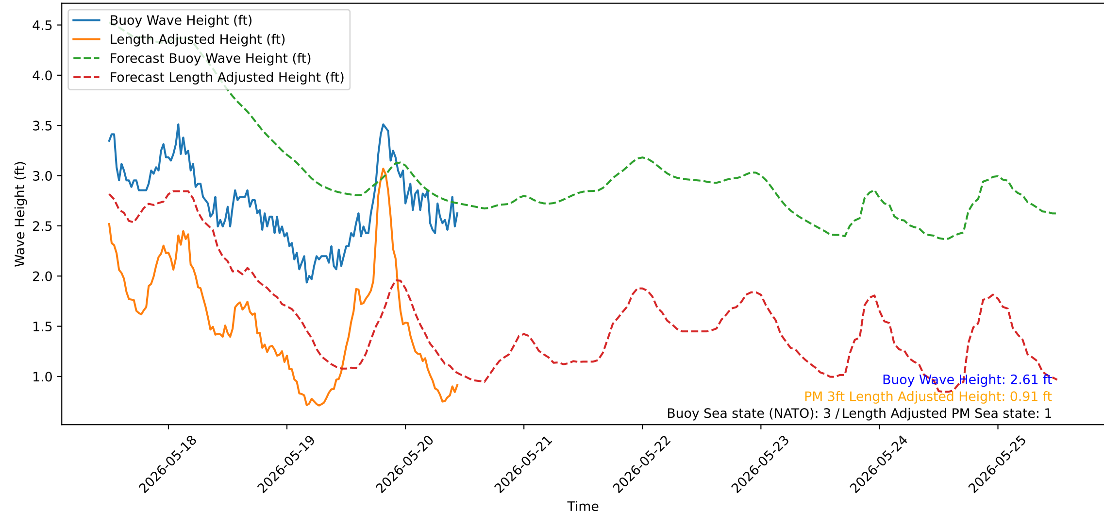
Wave Heights over Time for Red Beach at 2026-05-20 11:50:51
