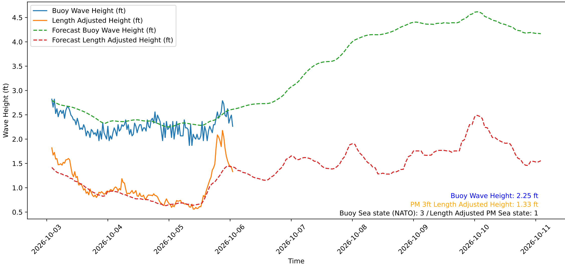
Wave Heights over Time for Oceanside Harbor at 2026-10-06 01:50:29
