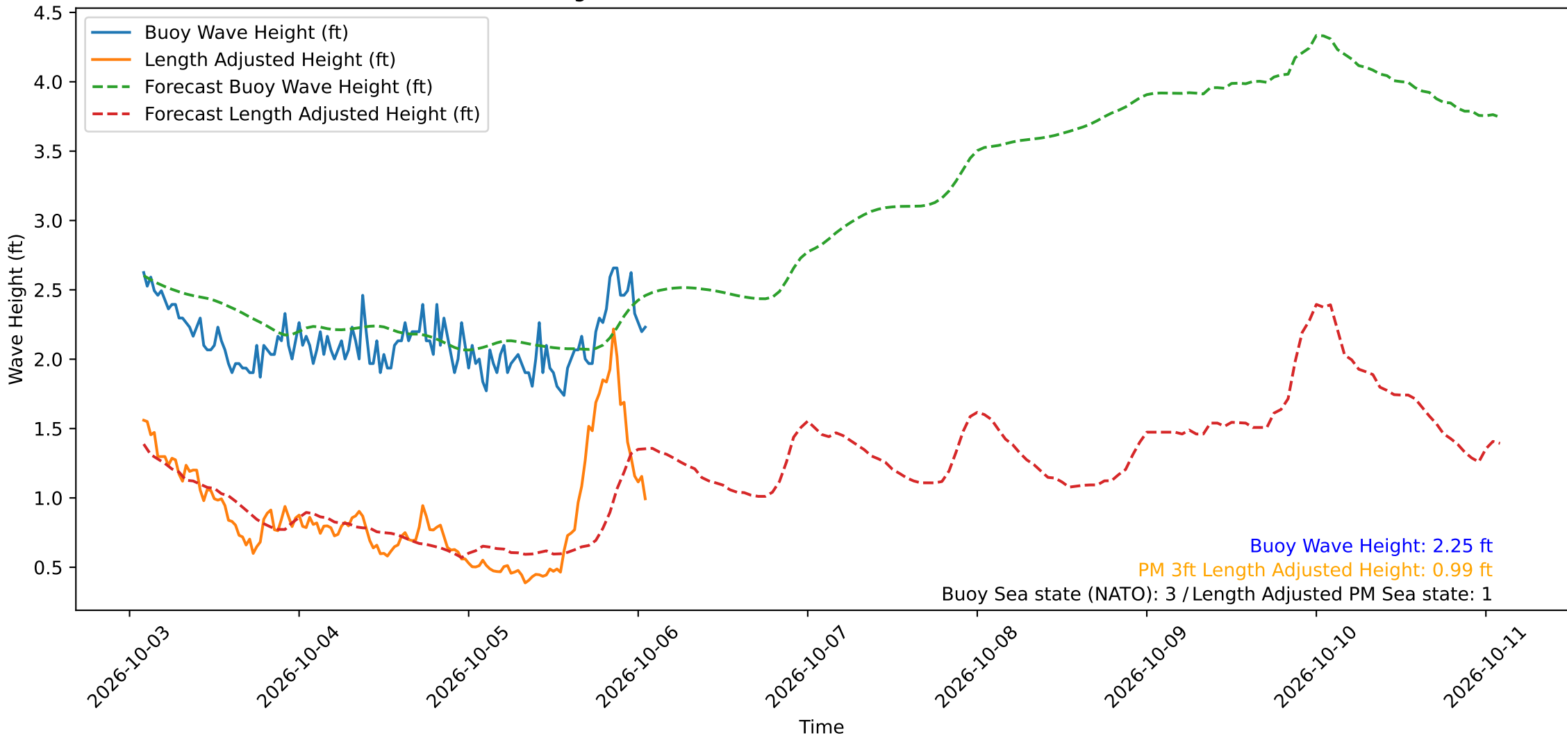
Wave Heights over Time for Red Beach at 2026-10-06 01:50:50
