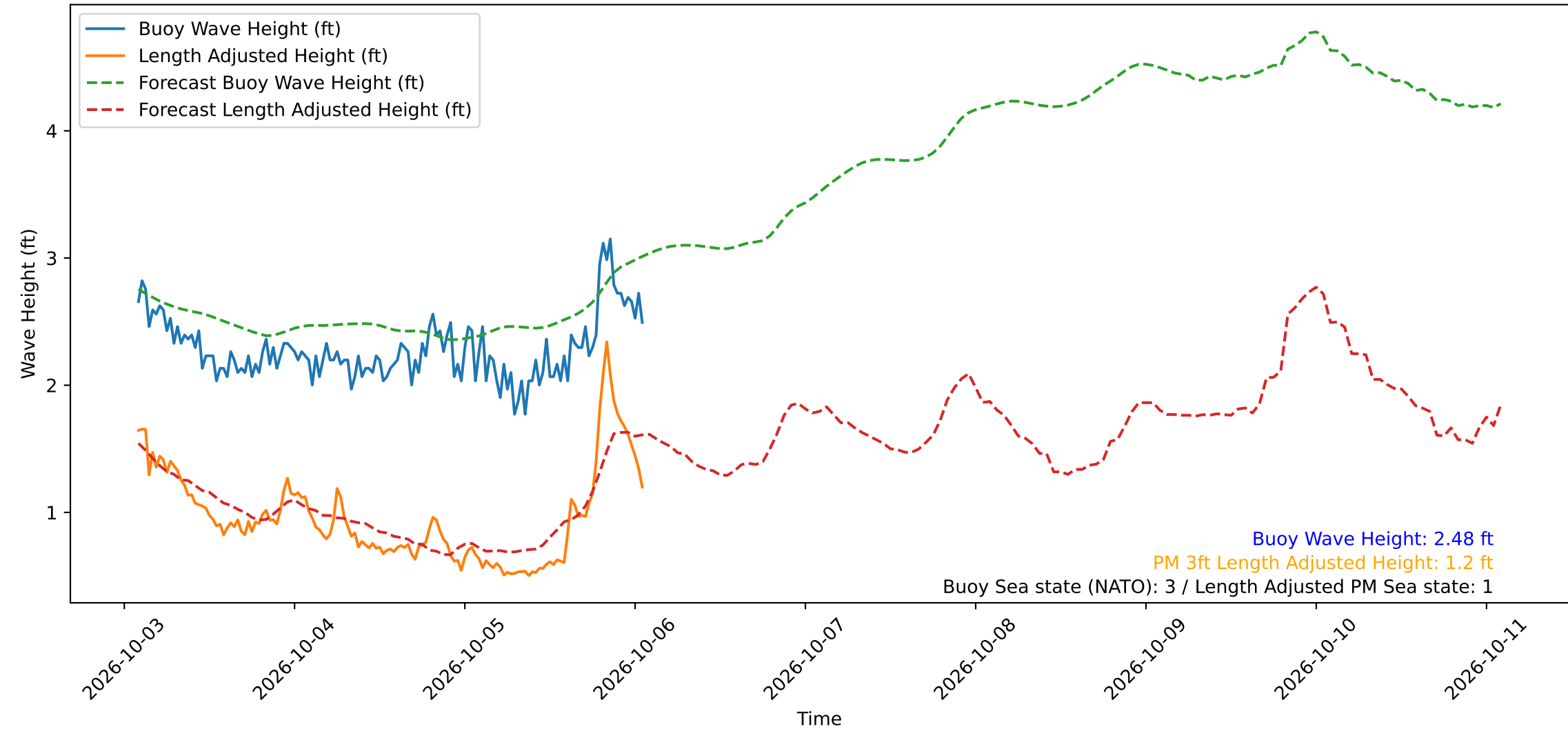
Wave Heights over Time for Green Beach at 2026-10-06 01:51:15
