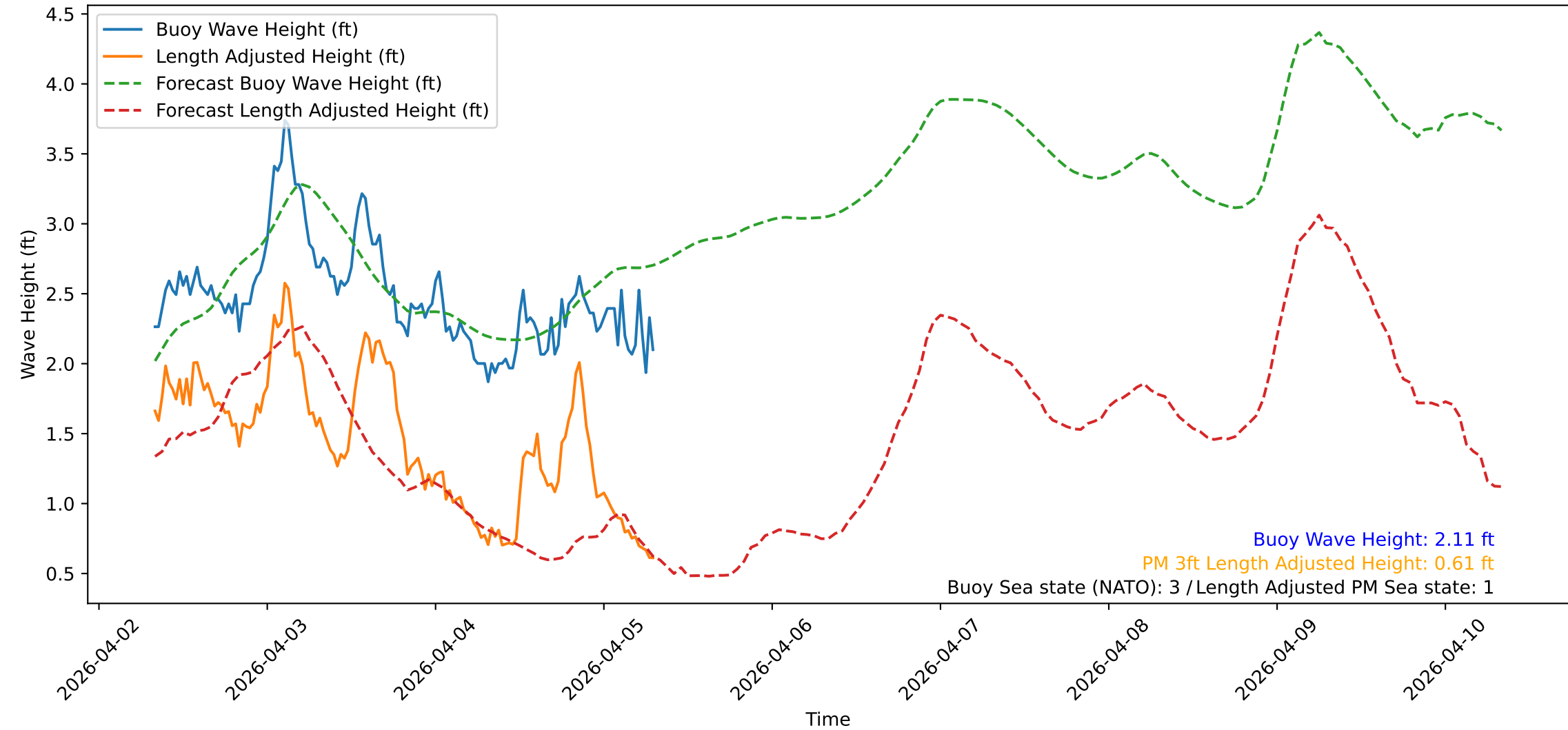
Wave Heights over Time for Red Beach at 2026-04-05 07:50:48
