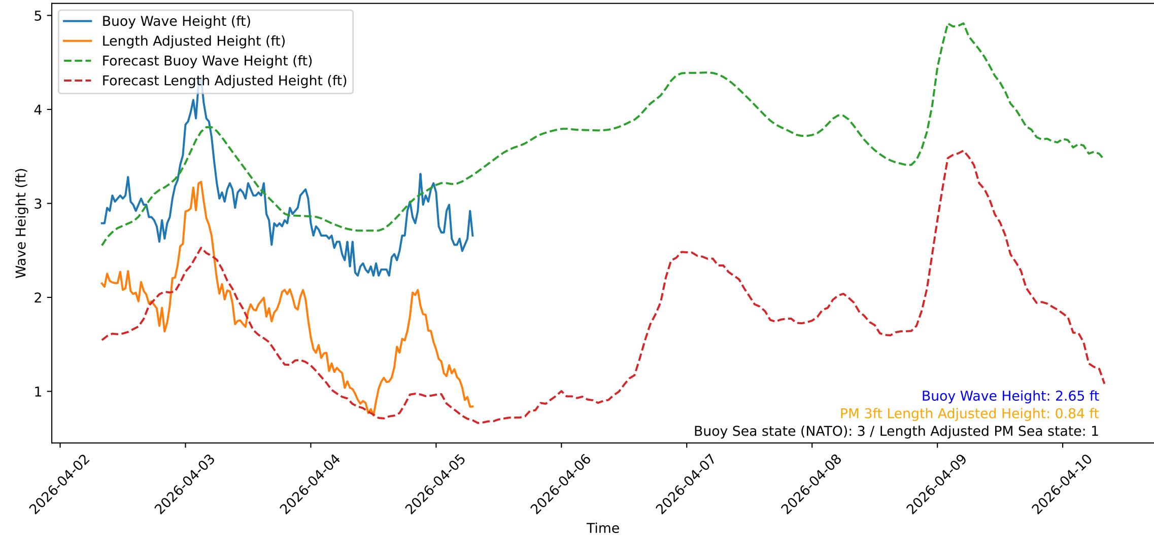
Wave Heights over Time for Green Beach at 2026-04-05 07:51:10
