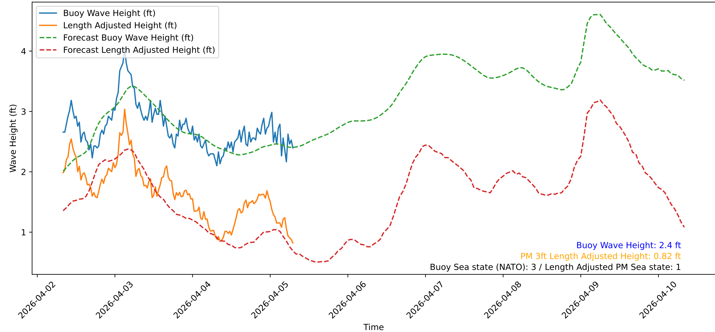
Wave Heights over Time for Oceanside Harbor at 2026-04-05 07:50:32
