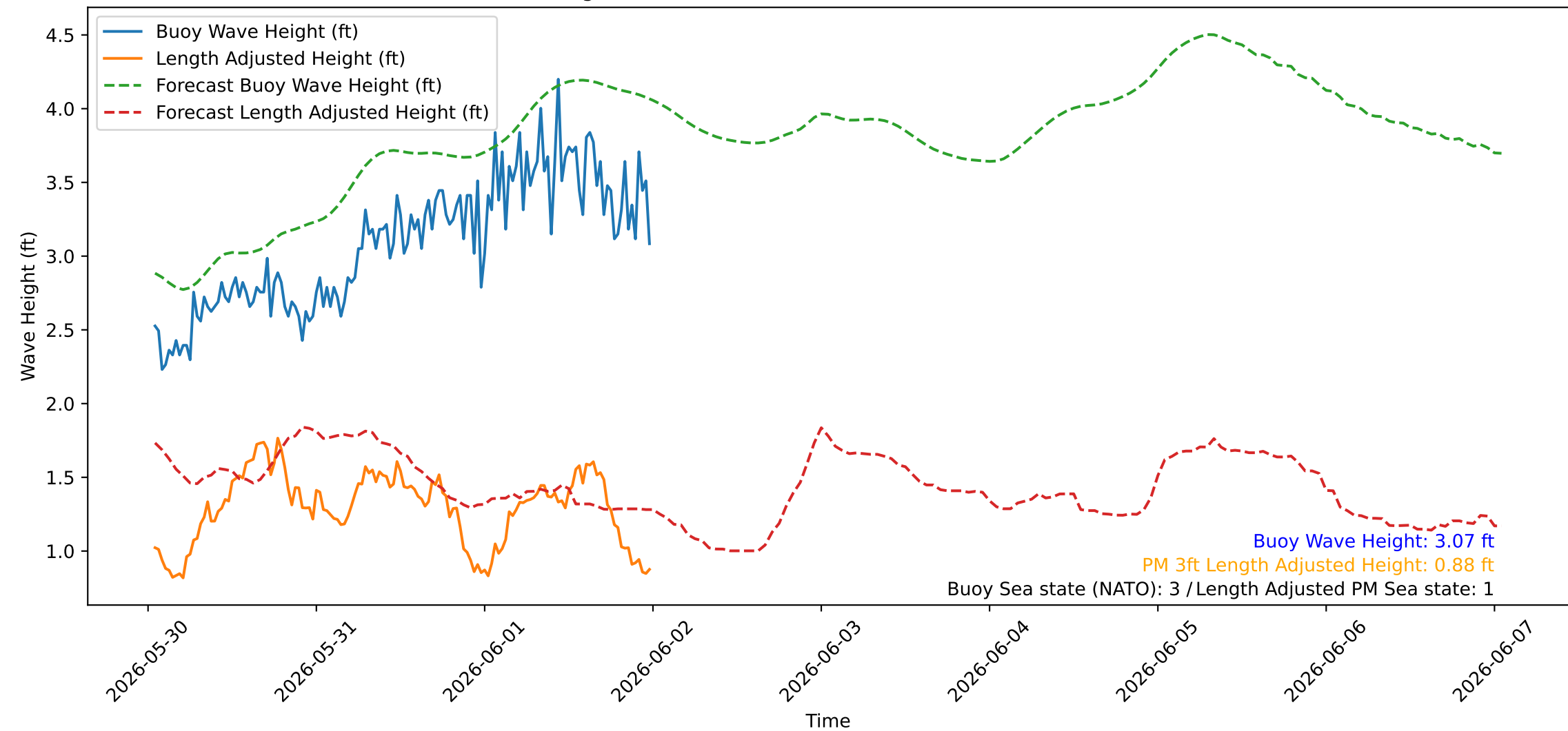
Wave Heights over Time for Red Beach at 2026-06-02 00:40:46
