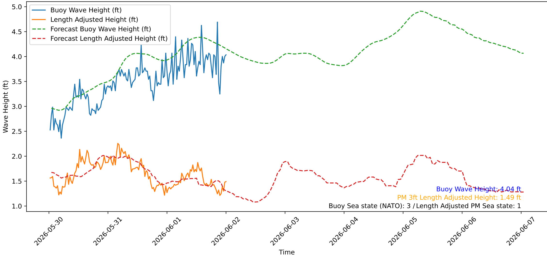
Wave Heights over Time for Oceanside Harbor at 2026-06-02 00:40:26
