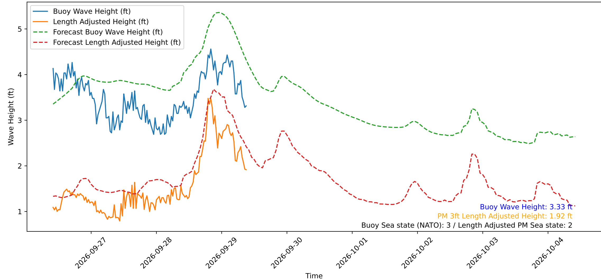
Wave Heights over Time for Green Beach at 2026-09-29 09:41:14
