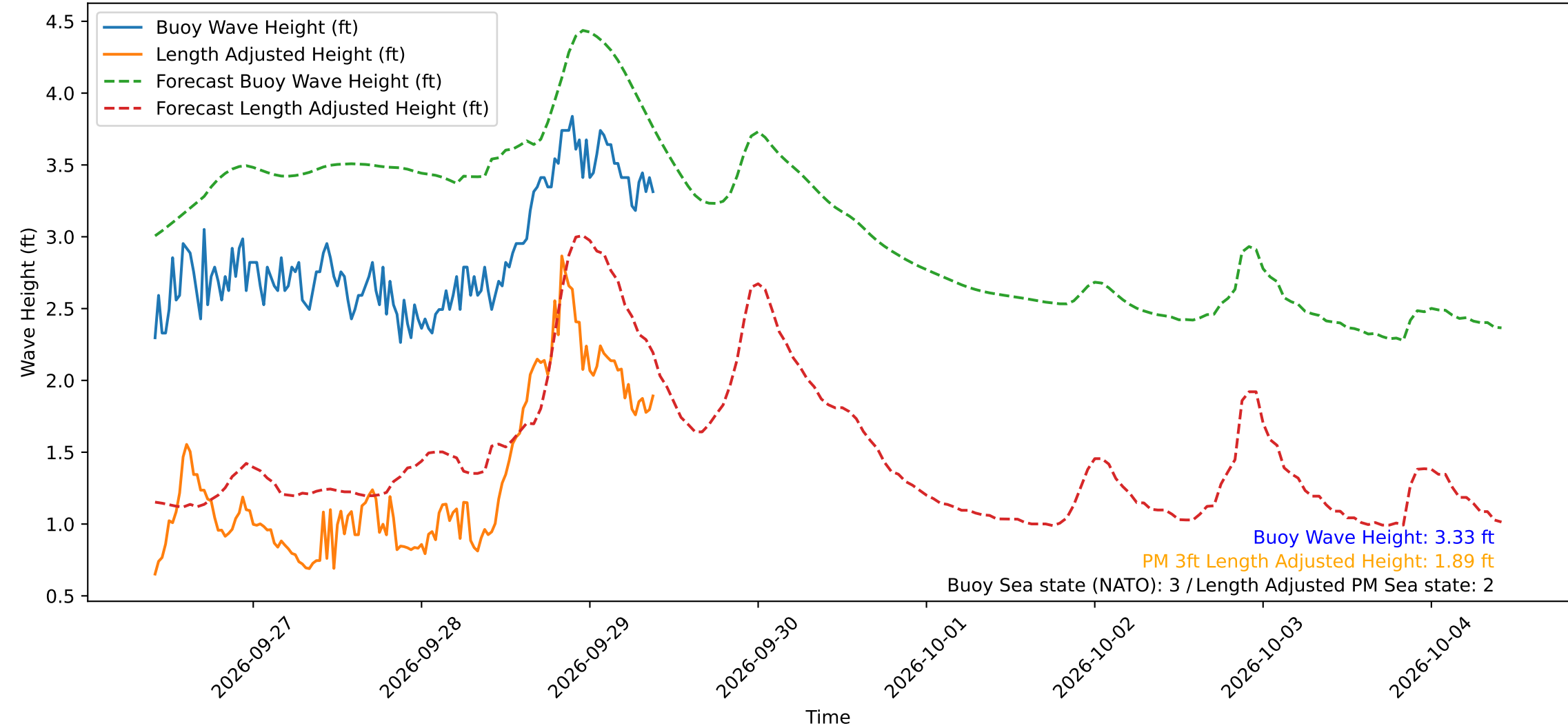
Wave Heights over Time for Red Beach at 2026-09-29 09:40:50
