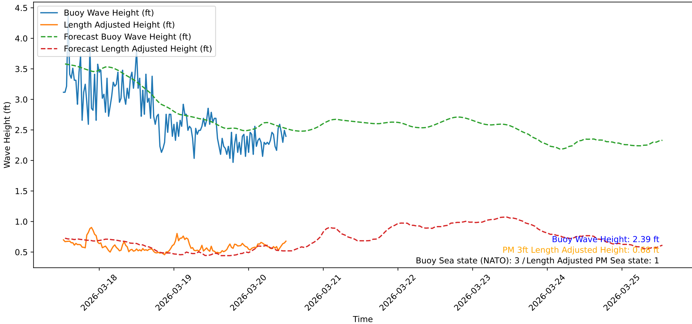
Wave Heights over Time for Oceanside Harbor at 2026-03-20 12:30:32
