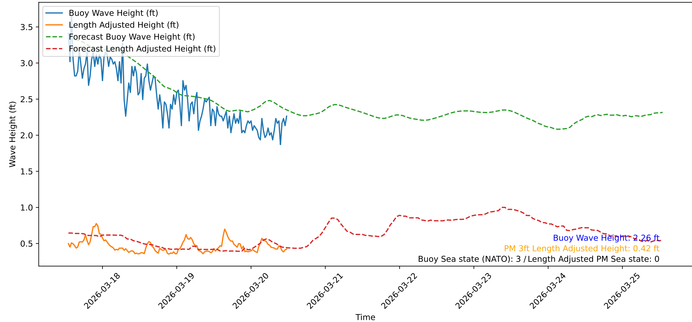
Wave Heights over Time for Red Beach at 2026-03-20 12:30:48
