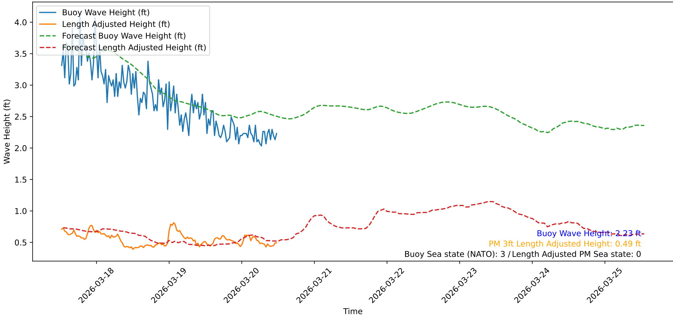
Wave Heights over Time for Green Beach at 2026-03-20 12:31:10
