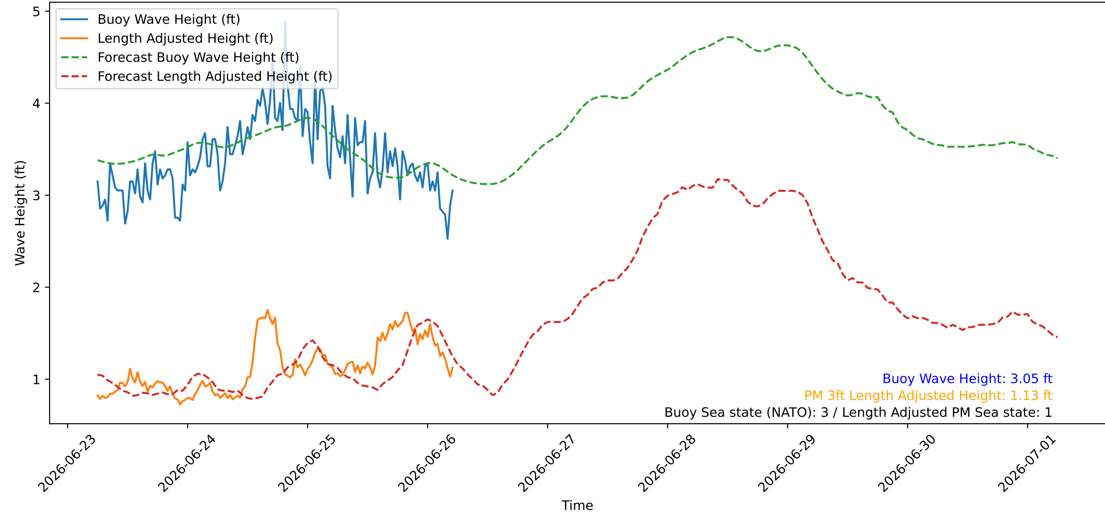
Wave Heights over Time for Oceanside Harbor at 2026-06-26 06:10:26
