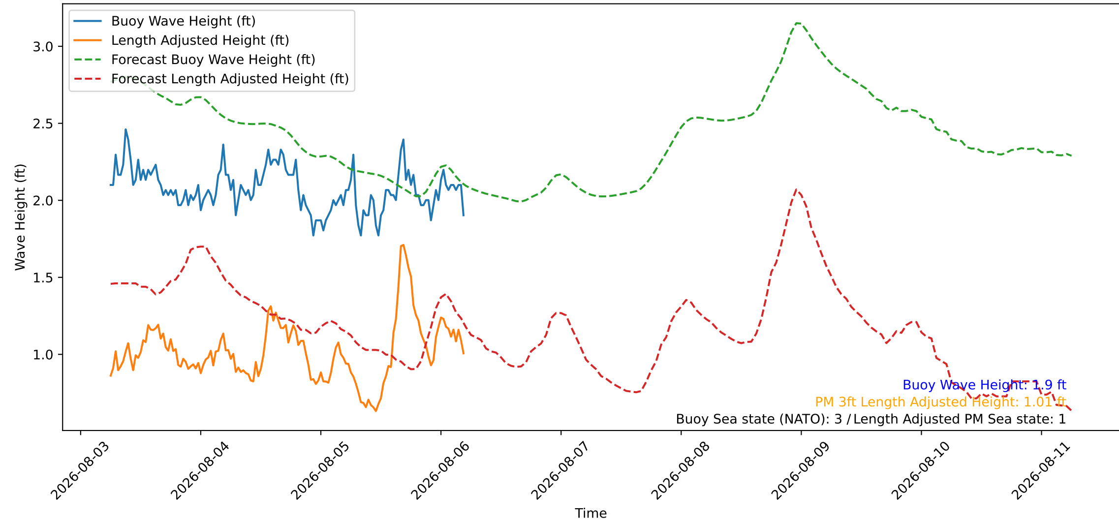
Wave Heights over Time for Red Beach at 2026-08-06 05:30:45
