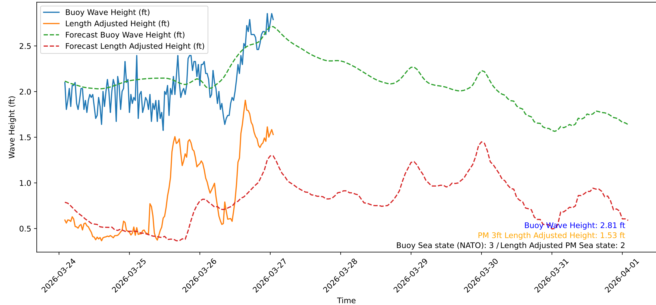
Wave Heights over Time for Red Beach at 2026-03-27 01:40:47
