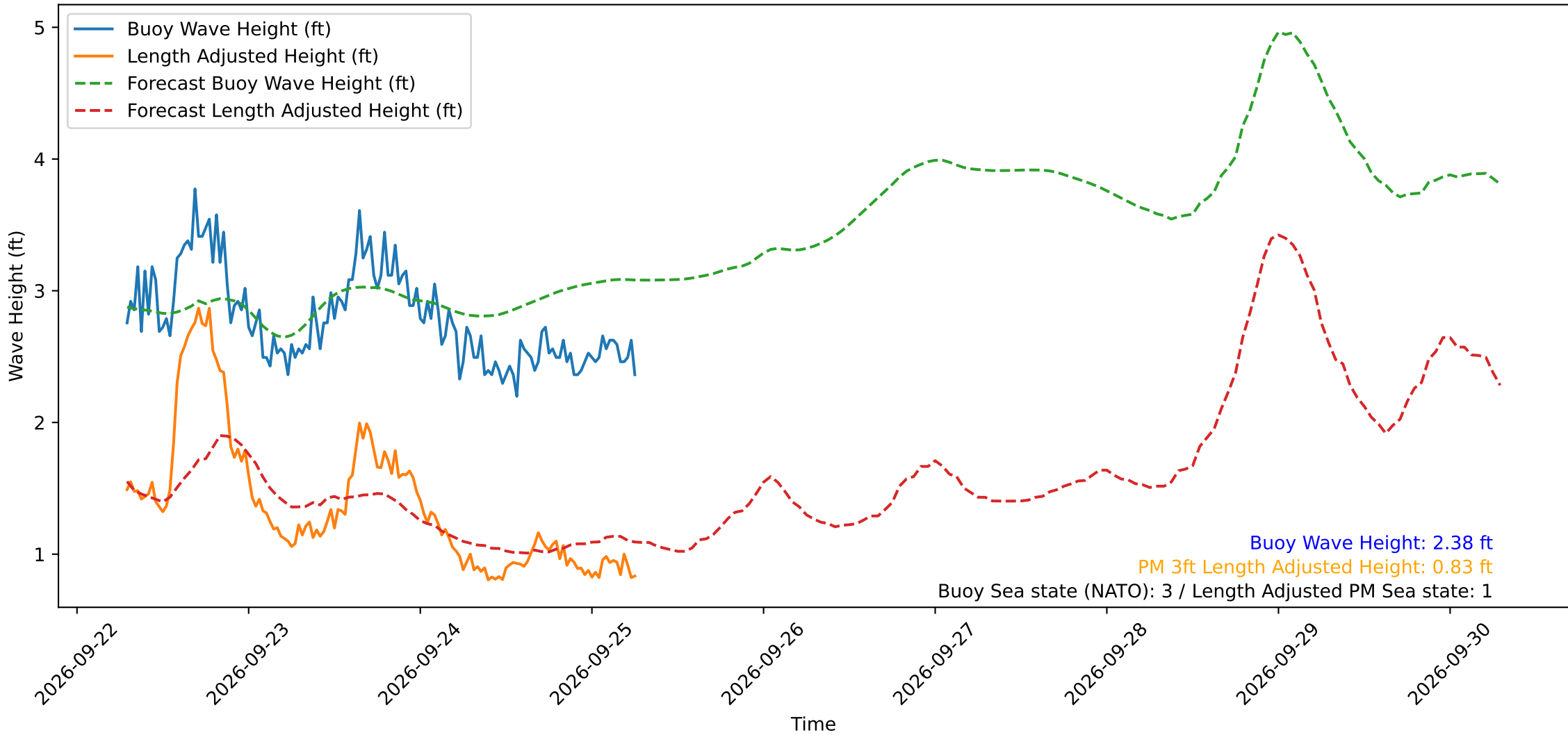
Wave Heights over Time for Oceanside Harbor at 2026-09-25 07:00:29
