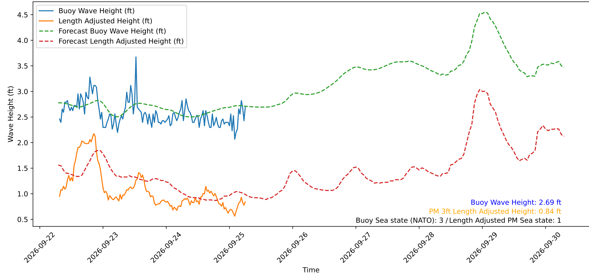
Wave Heights over Time for Red Beach at 2026-09-25 07:00:48
