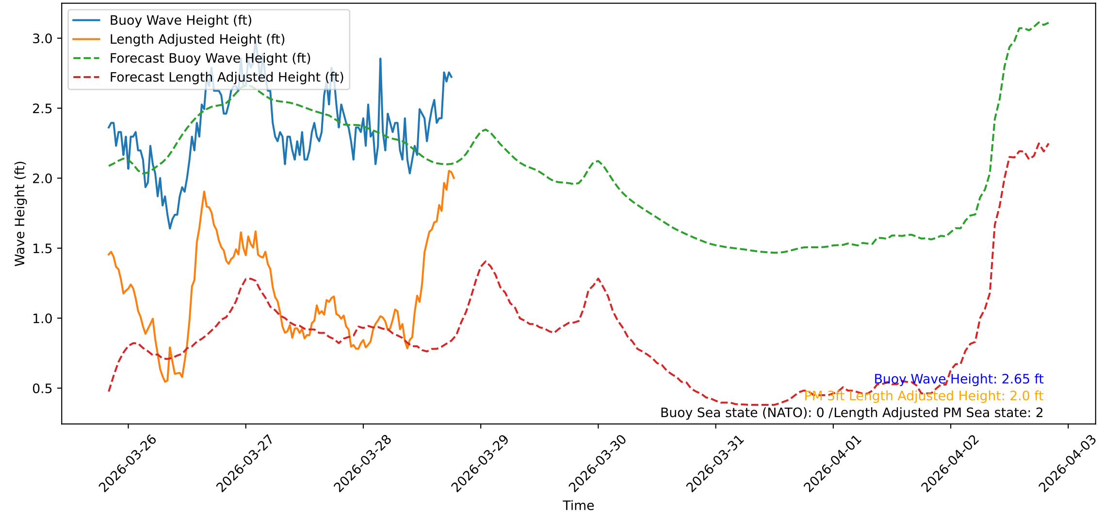
Wave Heights over Time for Red Beach at 2026-03-28 19:30:46
