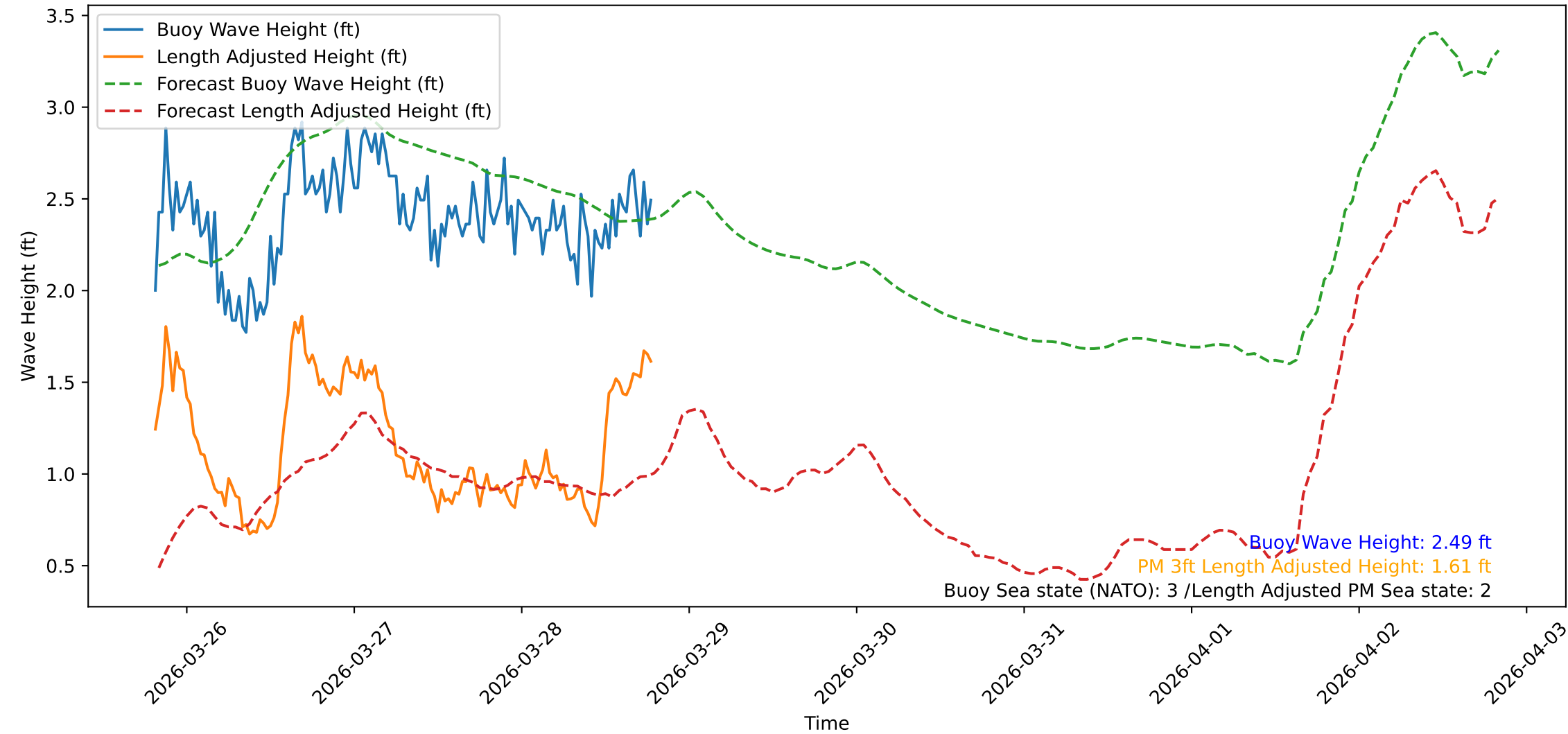
Wave Heights over Time for Oceanside Harbor at 2026-03-28 19:30:30
