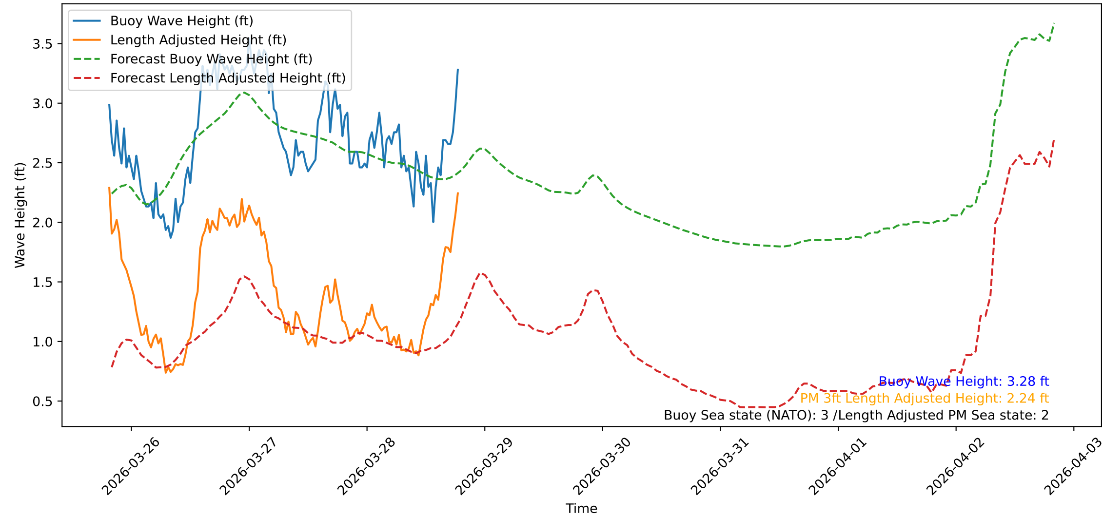
Wave Heights over Time for Green Beach at 2026-03-28 19:31:08
