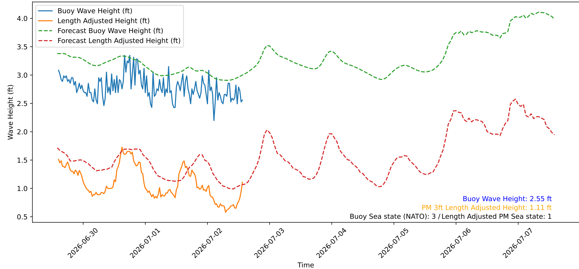
Wave Heights over Time for Red Beach at 2026-07-02 14:10:46
