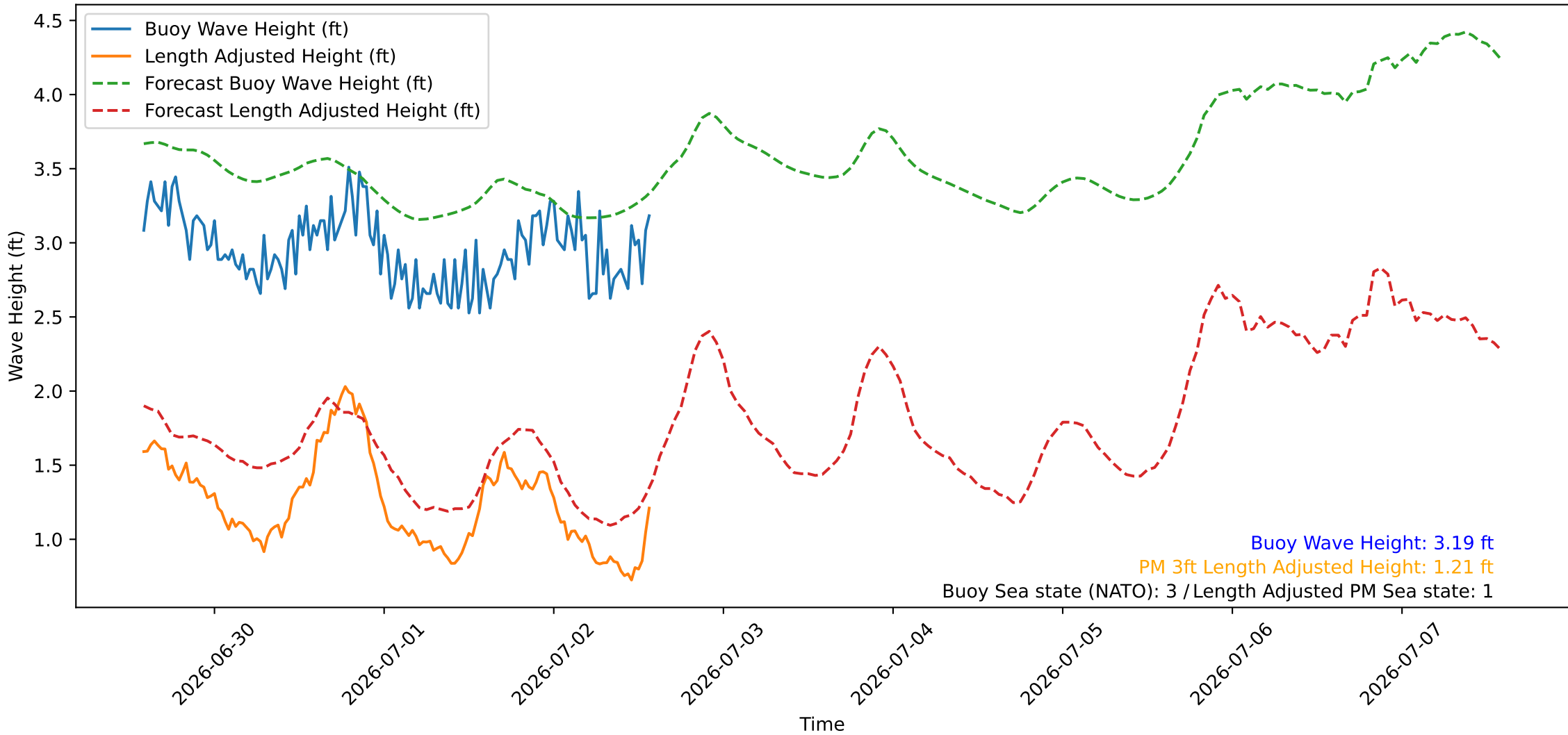
Wave Heights over Time for Green Beach at 2026-07-02 14:11:08
