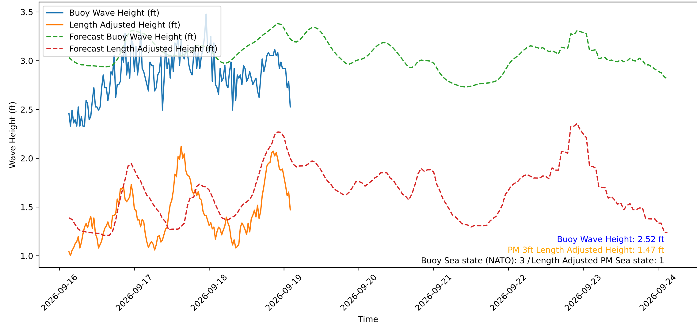
Wave Heights over Time for Green Beach at 2026-09-19 02:51:15
