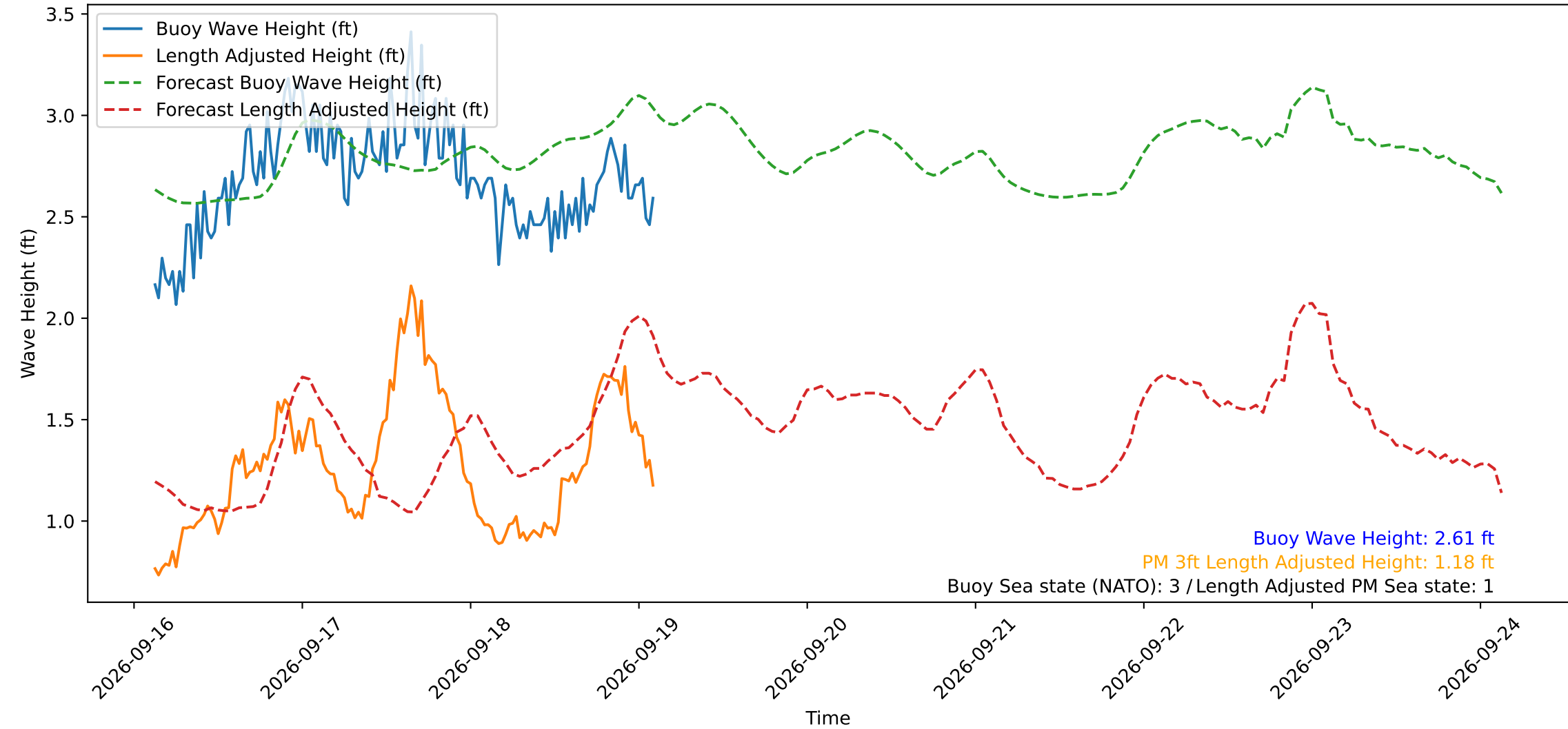
Wave Heights over Time for Red Beach at 2026-09-19 02:50:50
