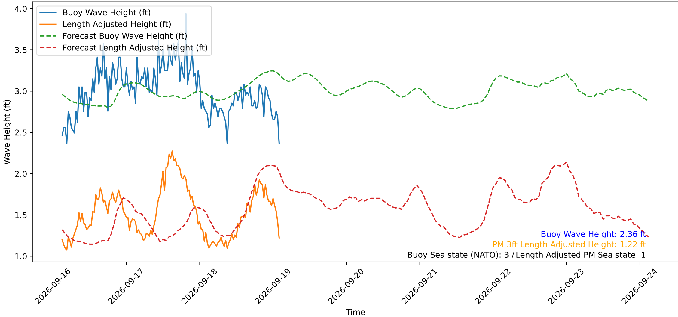
Wave Heights over Time for Oceanside Harbor at 2026-09-19 02:50:29
