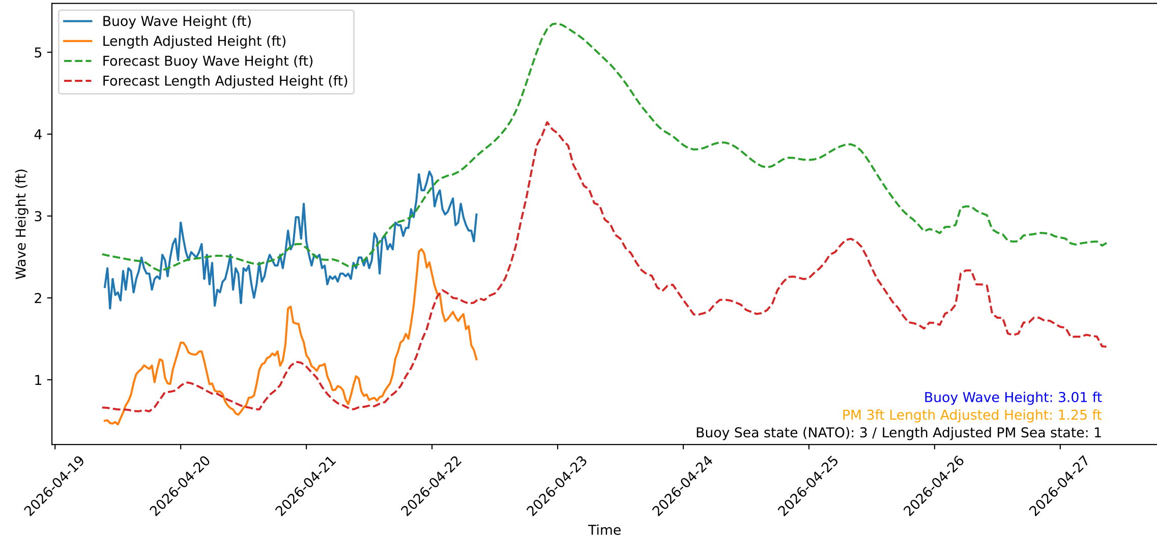
Wave Heights over Time for Green Beach at 2026-04-22 09:21:14
