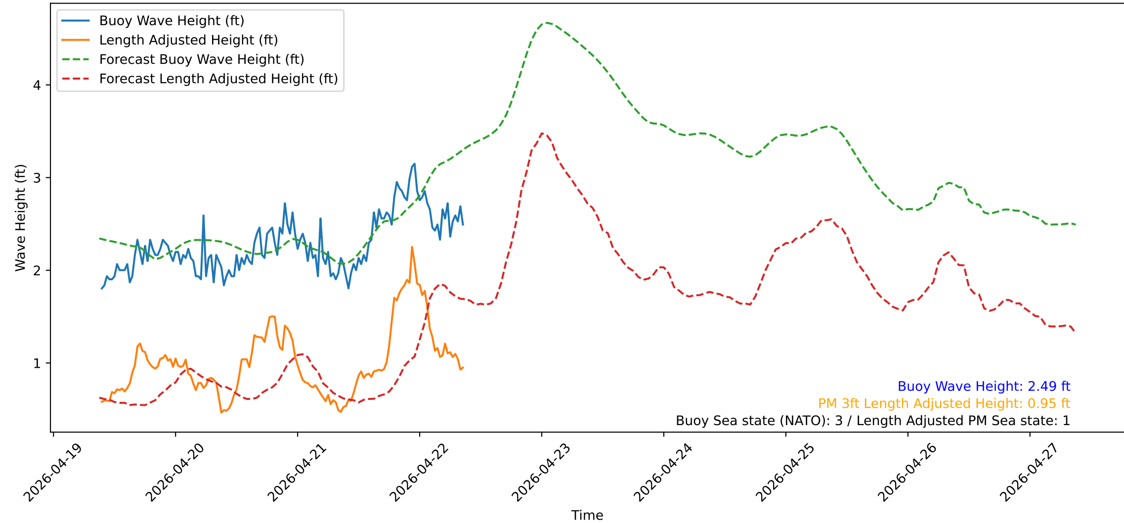
Wave Heights over Time for Red Beach at 2026-04-22 09:20:52
