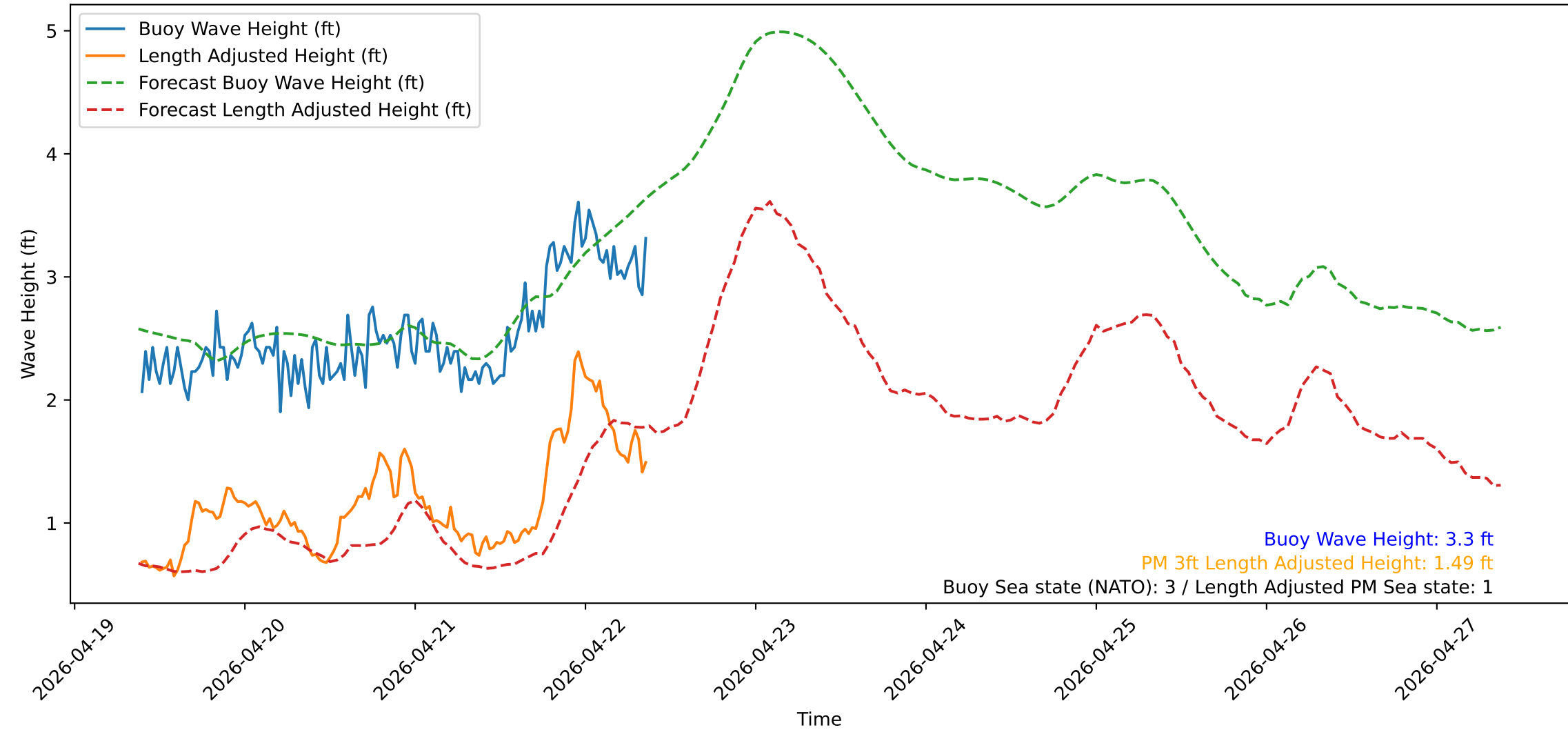
Wave Heights over Time for Oceanside Harbor at 2026-04-22 09:20:31
