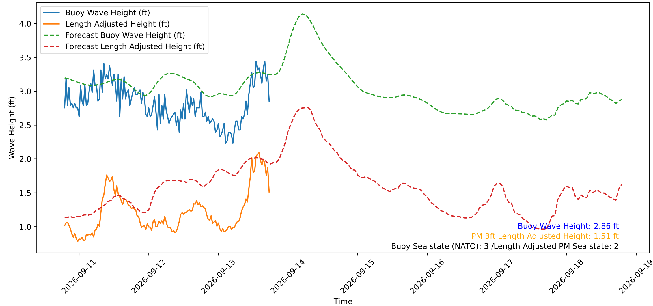
Wave Heights over Time for Red Beach at 2026-09-13 18:30:49
