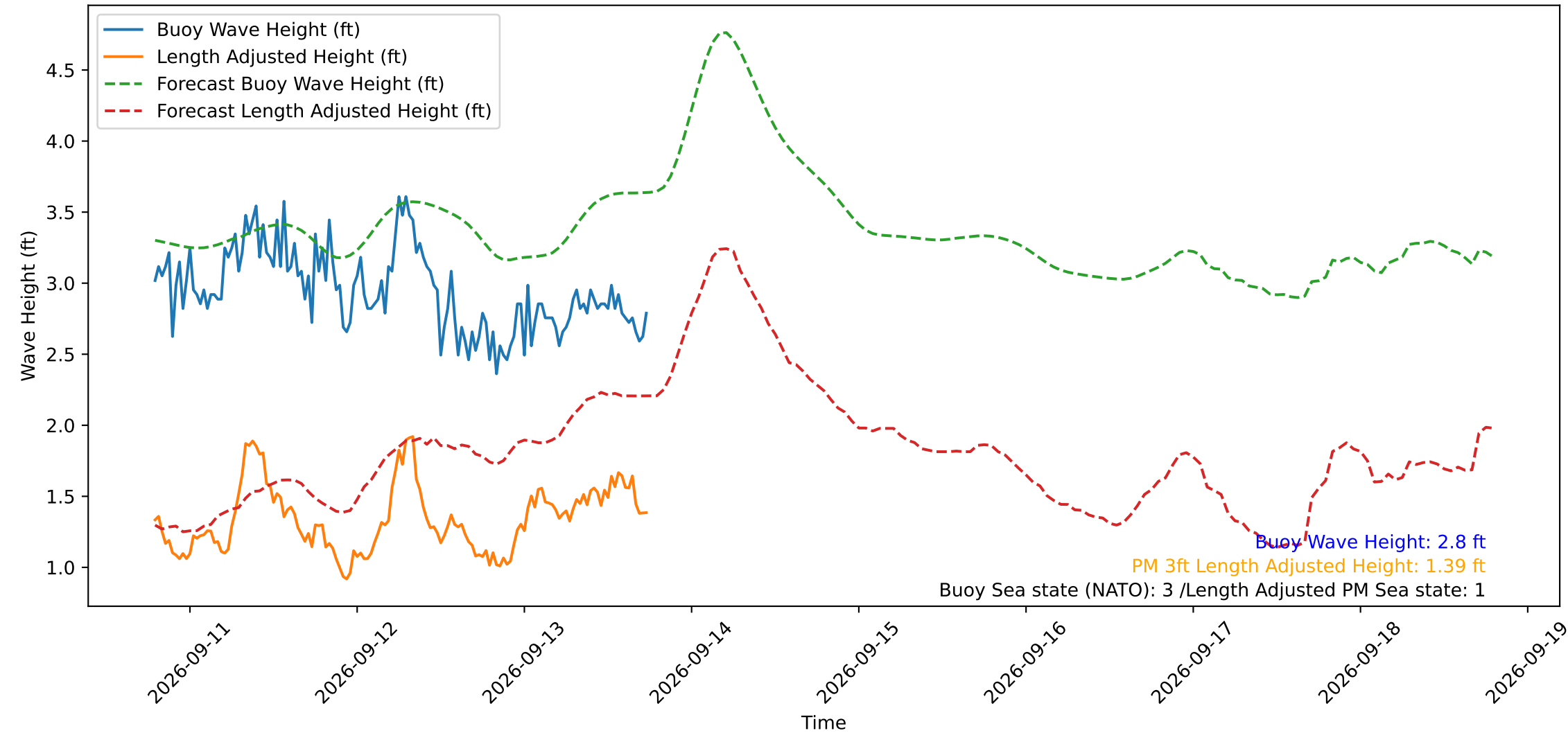
Wave Heights over Time for Green Beach at 2026-09-13 18:31:12
