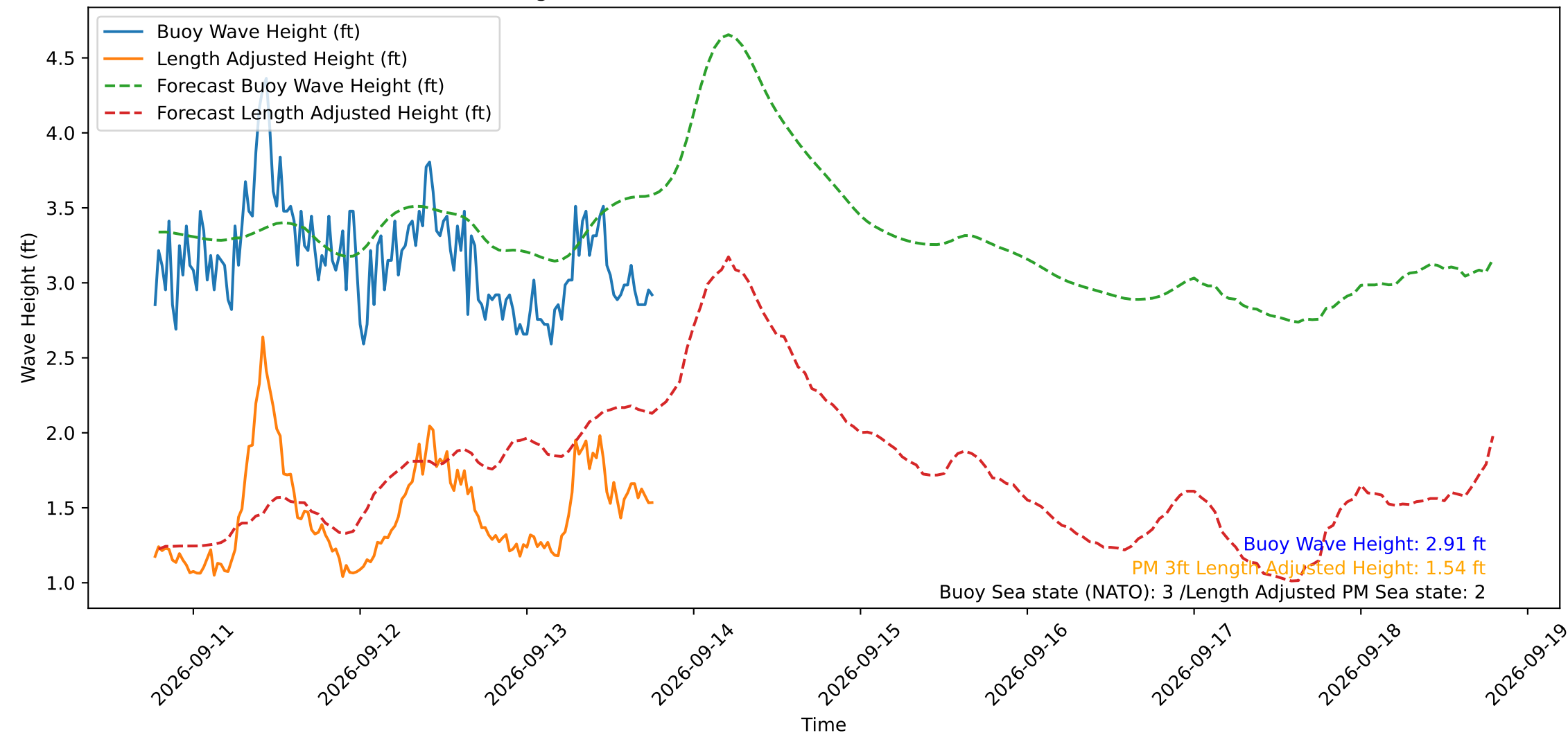
Wave Heights over Time for Oceanside Harbor at 2026-09-13 18:30:30
