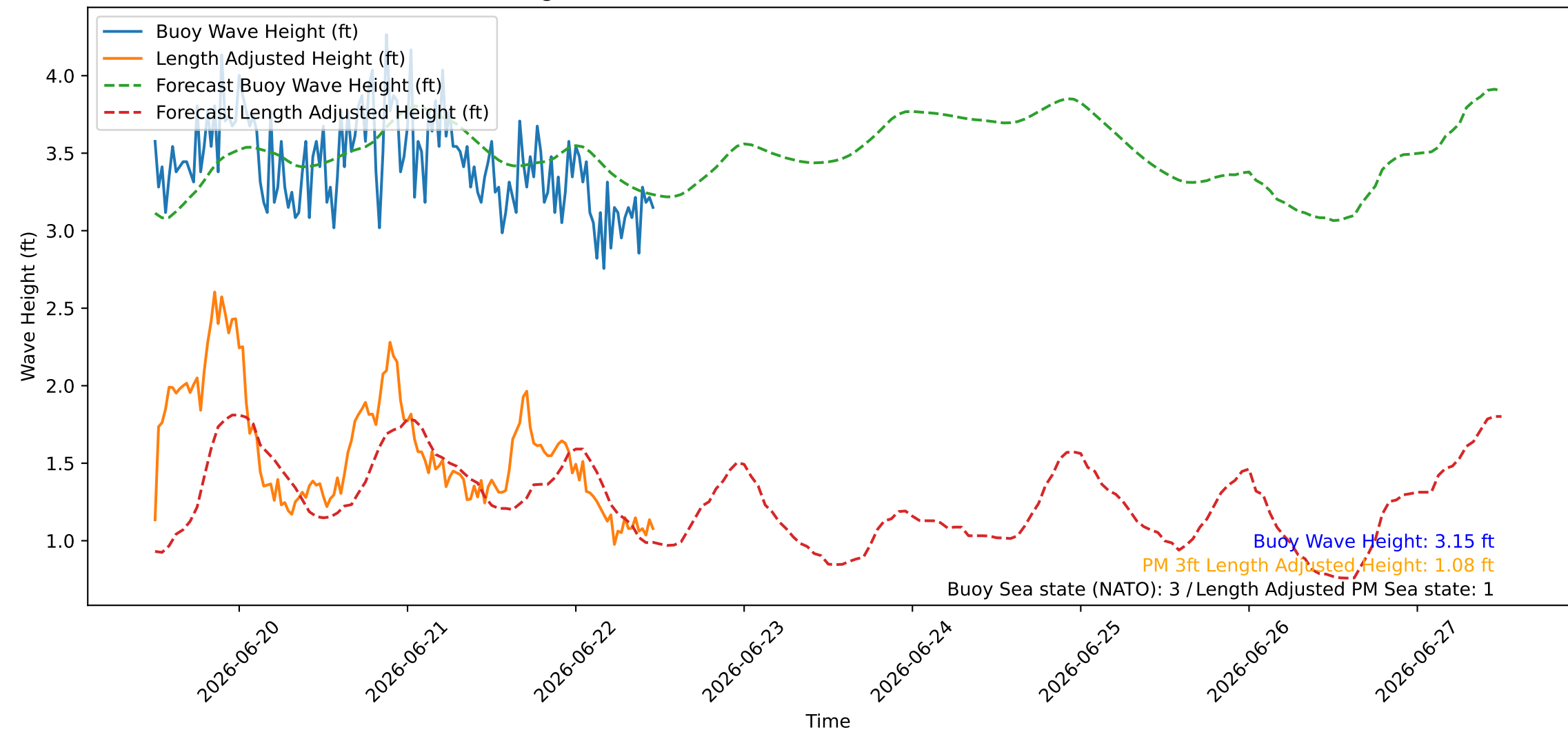
Wave Heights over Time for Oceanside Harbor at 2026-06-22 12:00:26
