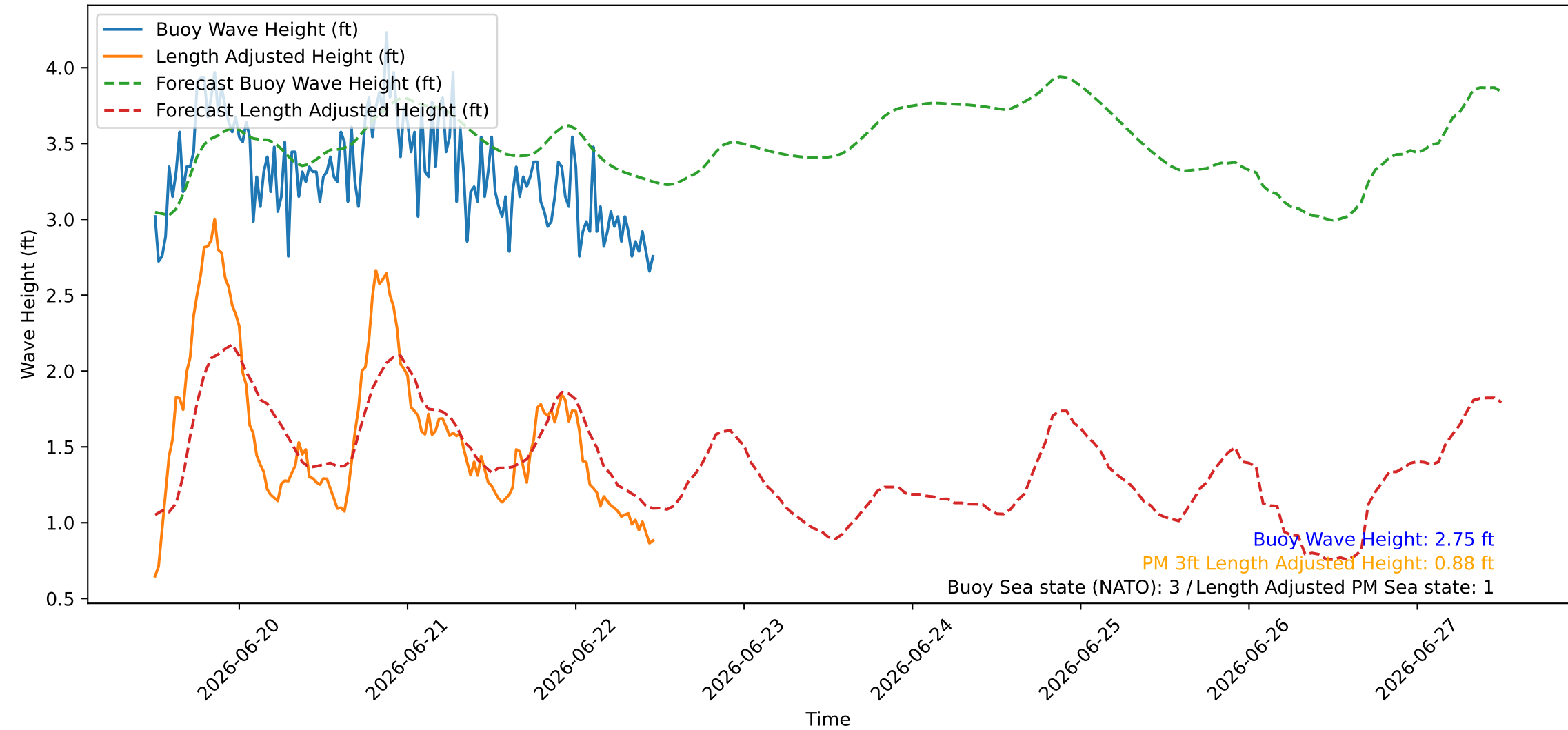
Wave Heights over Time for Green Beach at 2026-06-22 12:01:09
