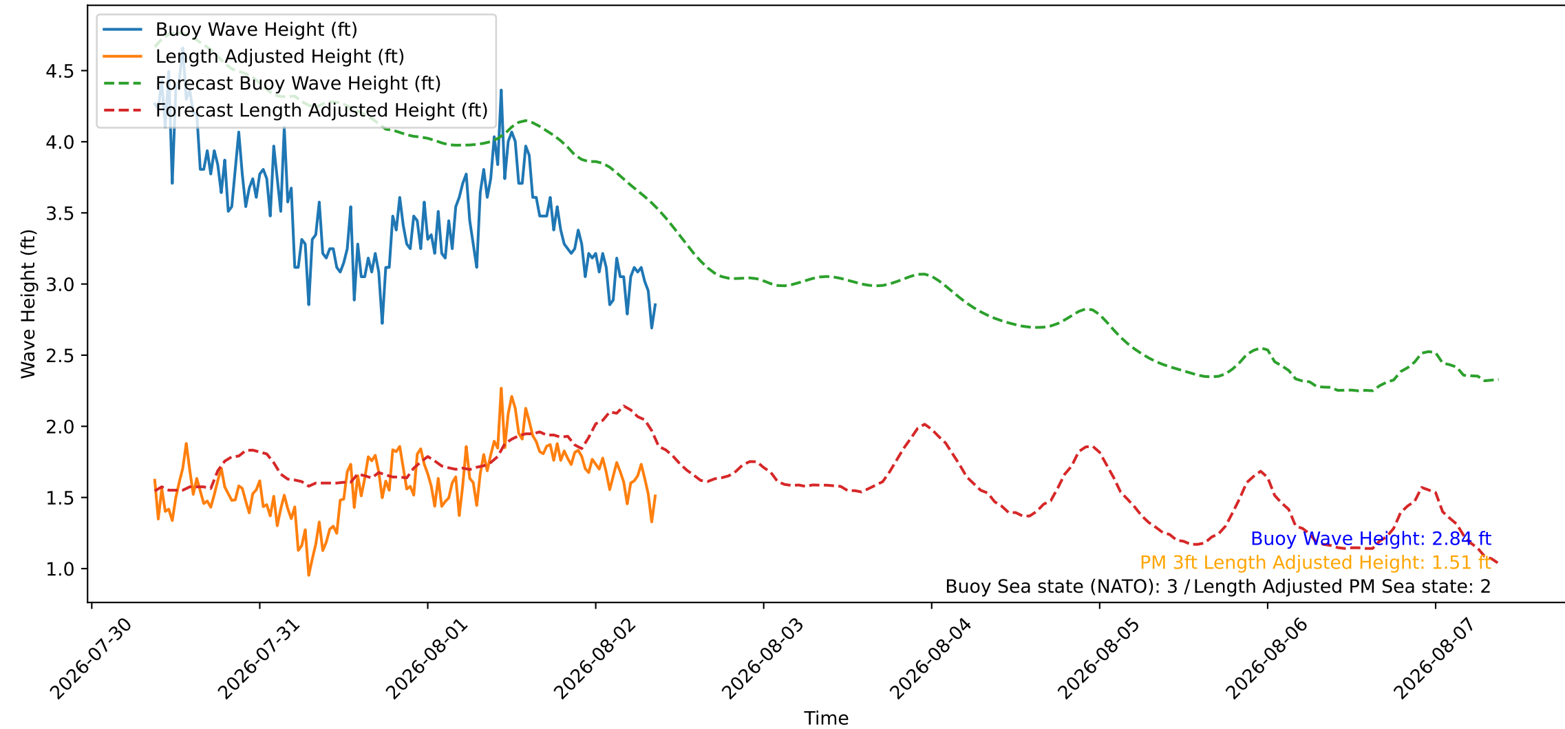
Wave Heights over Time for Oceanside Harbor at 2026-08-02 09:10:27
