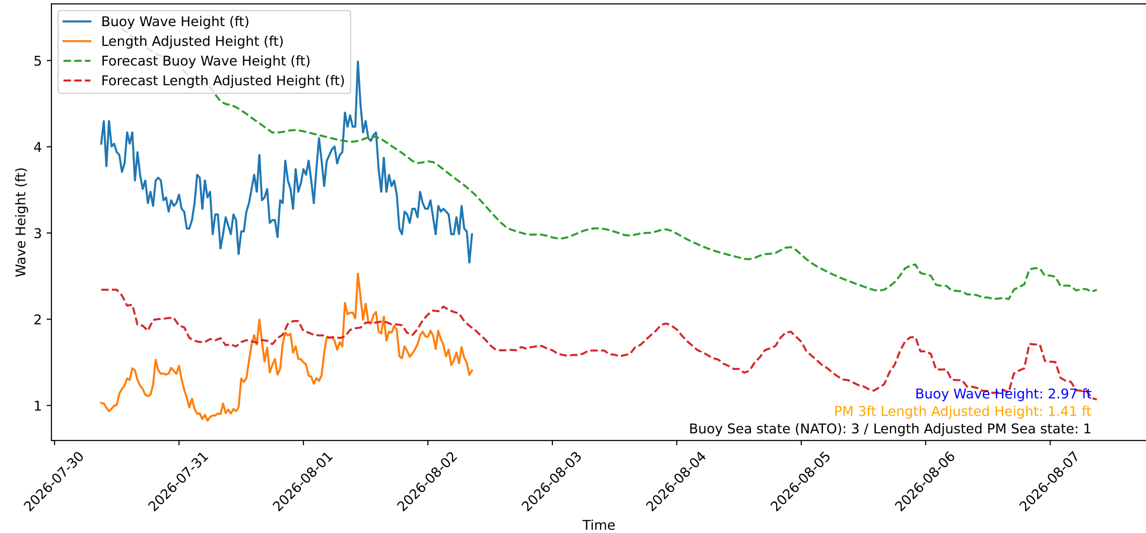
Wave Heights over Time for Green Beach at 2026-08-02 09:11:09
