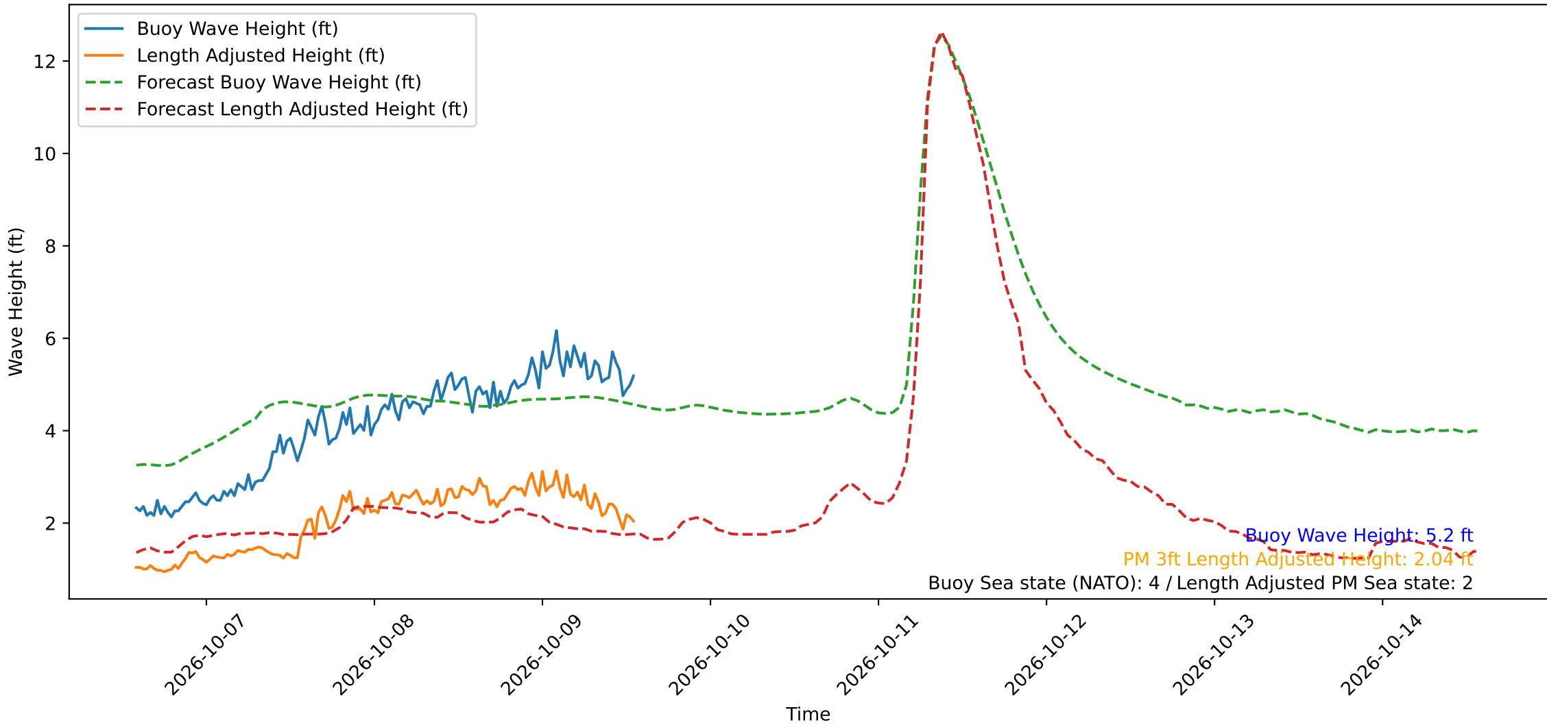
Wave Heights over Time for Green Beach at 2026-10-09 13:51:14
