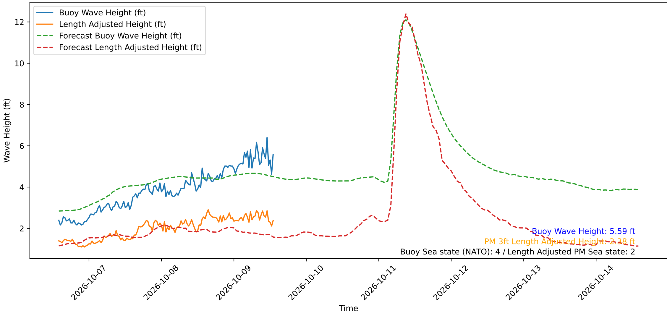
Wave Heights over Time for Oceanside Harbor at 2026-10-09 13:50:30
