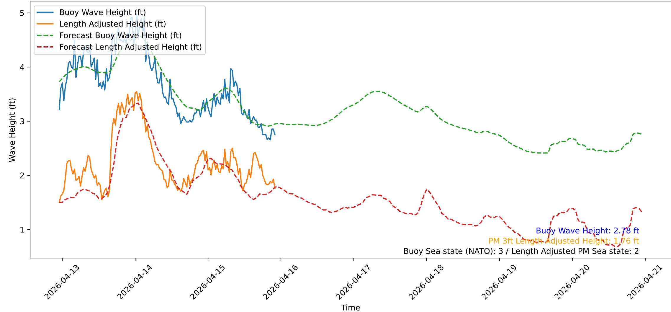
Wave Heights over Time for Green Beach at 2026-04-15 22:51:18
