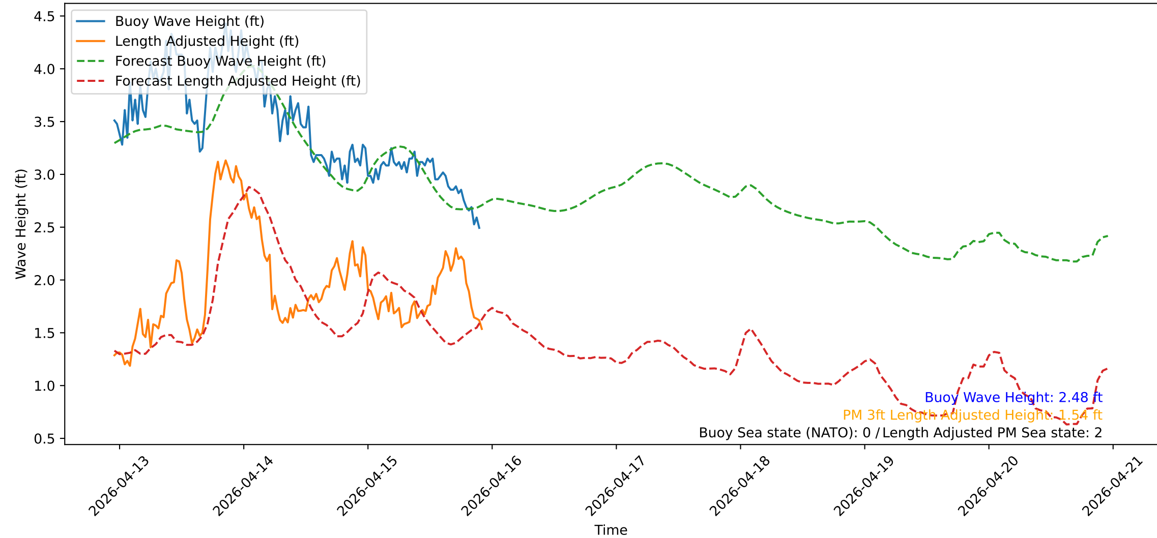
Wave Heights over Time for Red Beach at 2026-04-15 22:50:55
