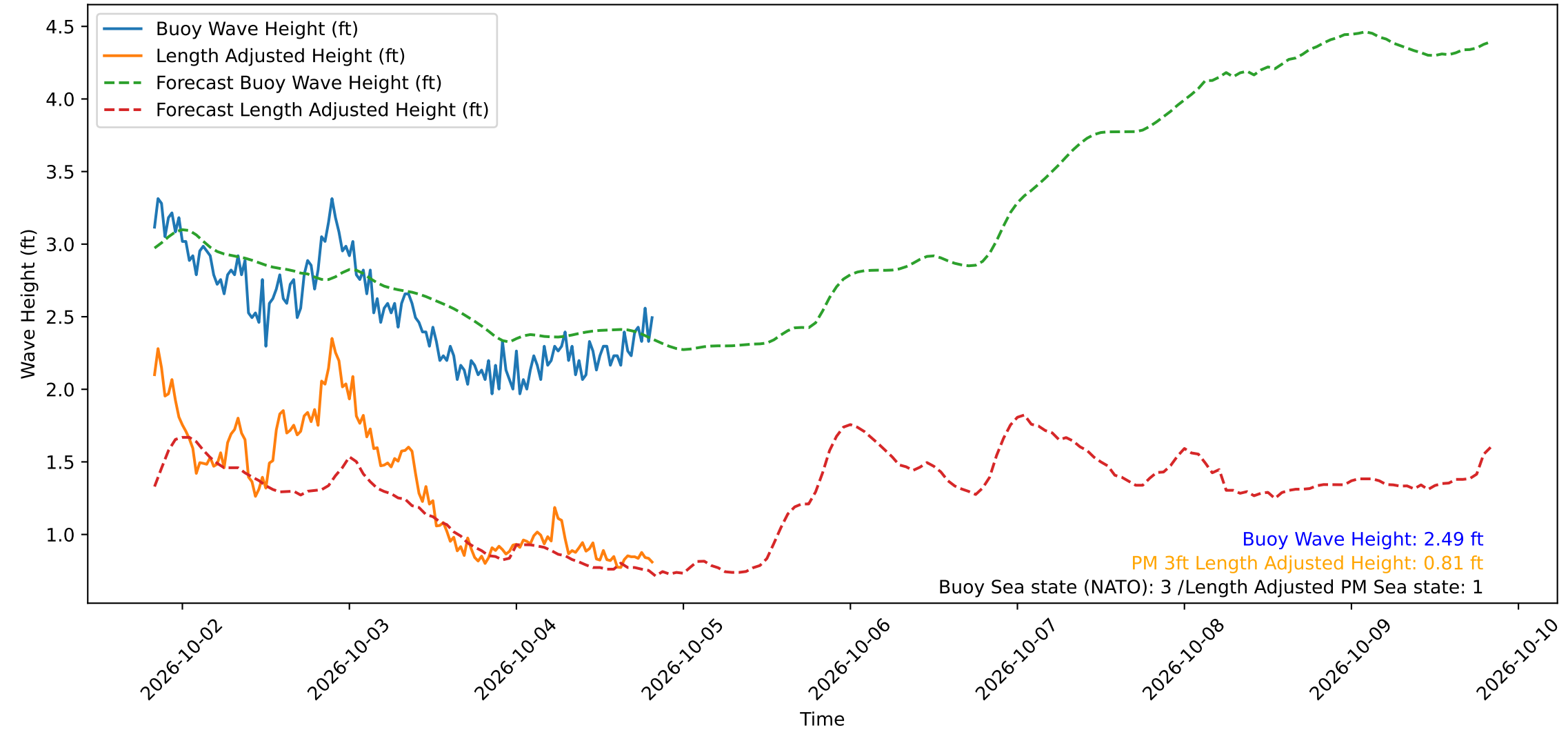
Wave Heights over Time for Oceanside Harbor at 2026-10-04 20:10:29
