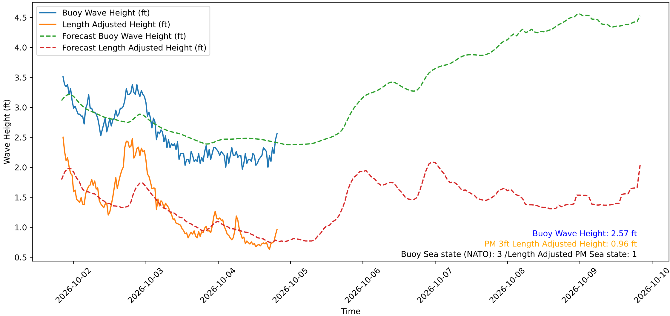
Wave Heights over Time for Green Beach at 2026-10-04 20:11:11
