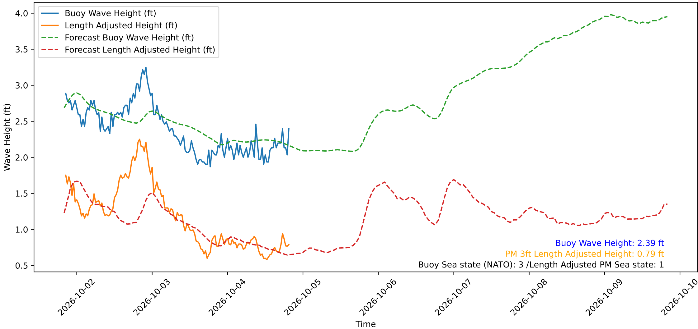
Wave Heights over Time for Red Beach at 2026-10-04 20:10:48
