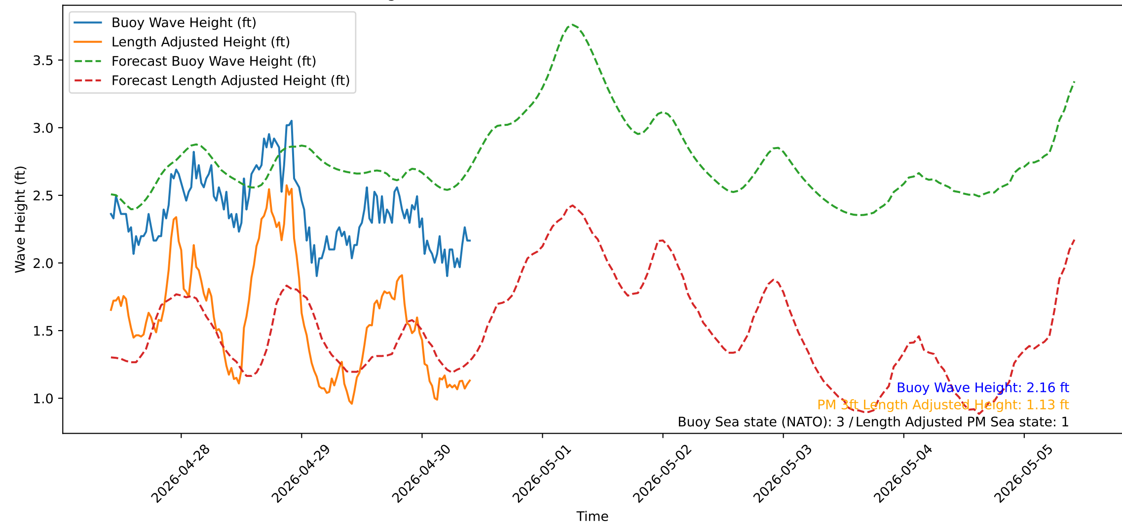
Wave Heights over Time for Oceanside Harbor at 2026-04-30 10:00:32
