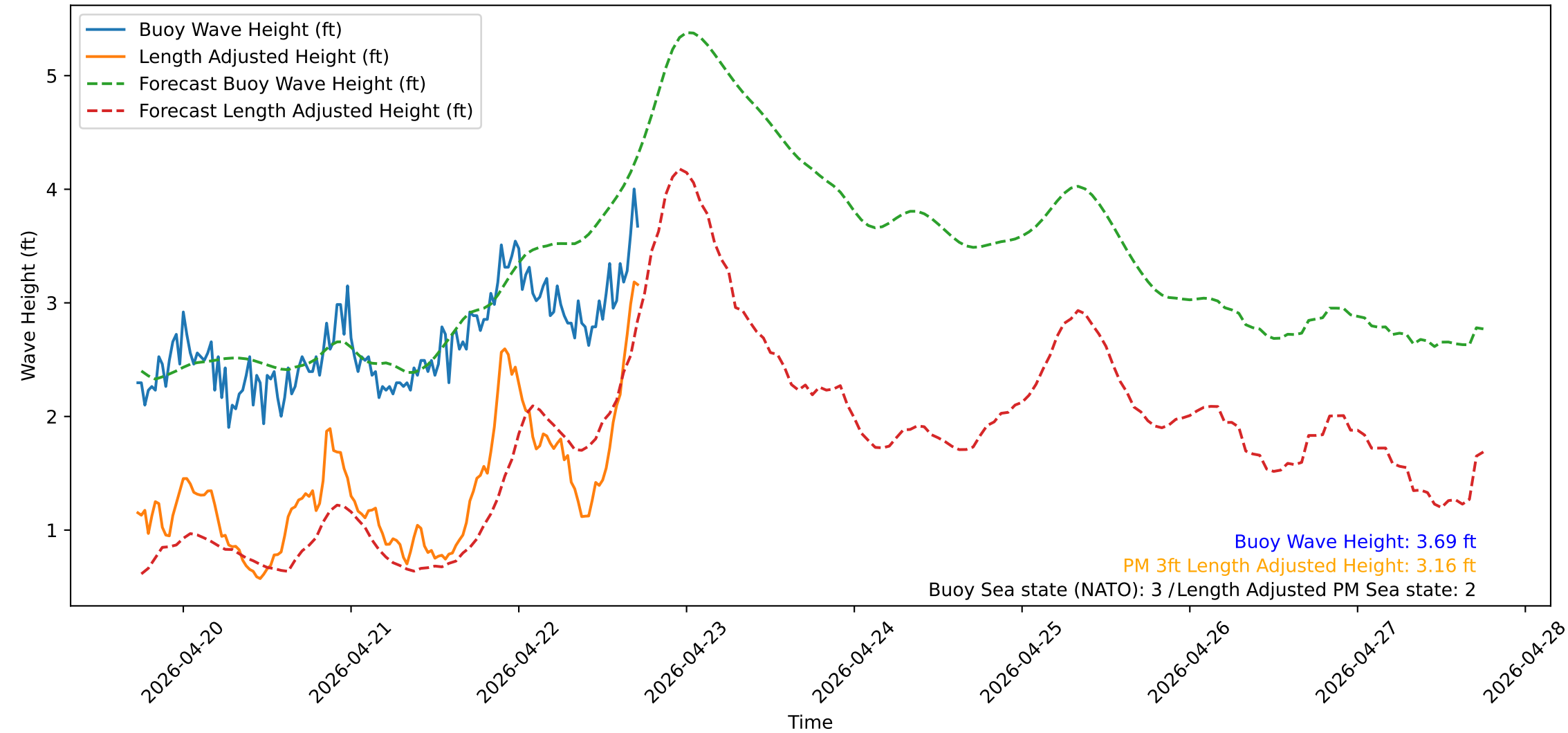
Wave Heights over Time for Green Beach at 2026-04-22 17:41:13
