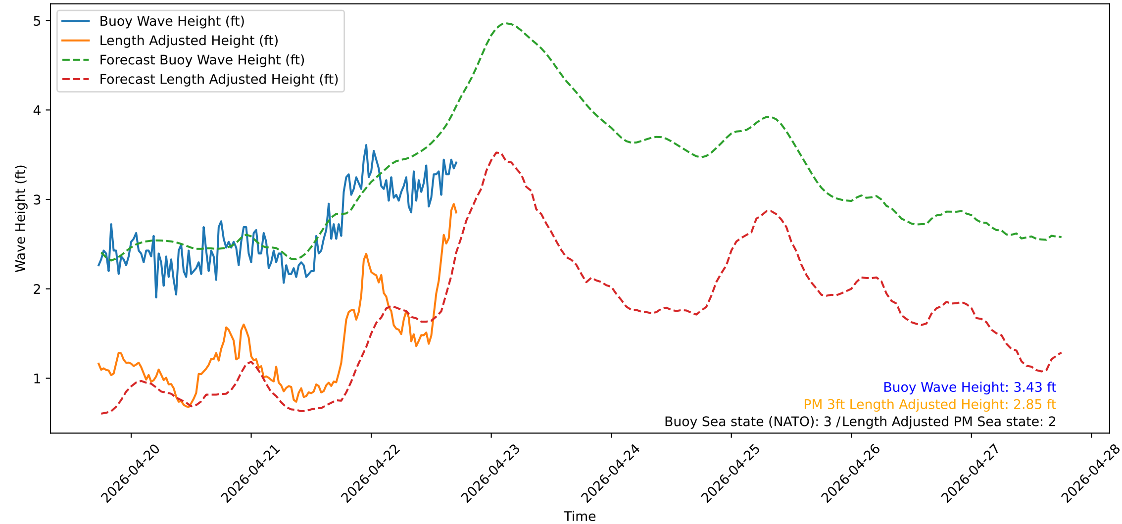
Wave Heights over Time for Oceanside Harbor at 2026-04-22 17:40:31
