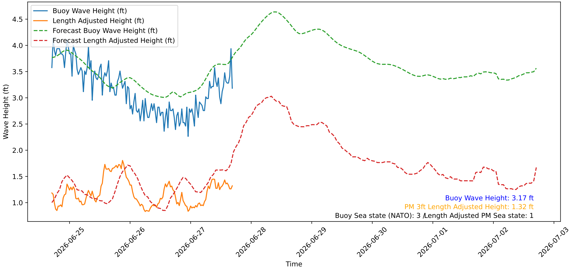
Wave Heights over Time for Green Beach at 2026-06-27 17:11:08
