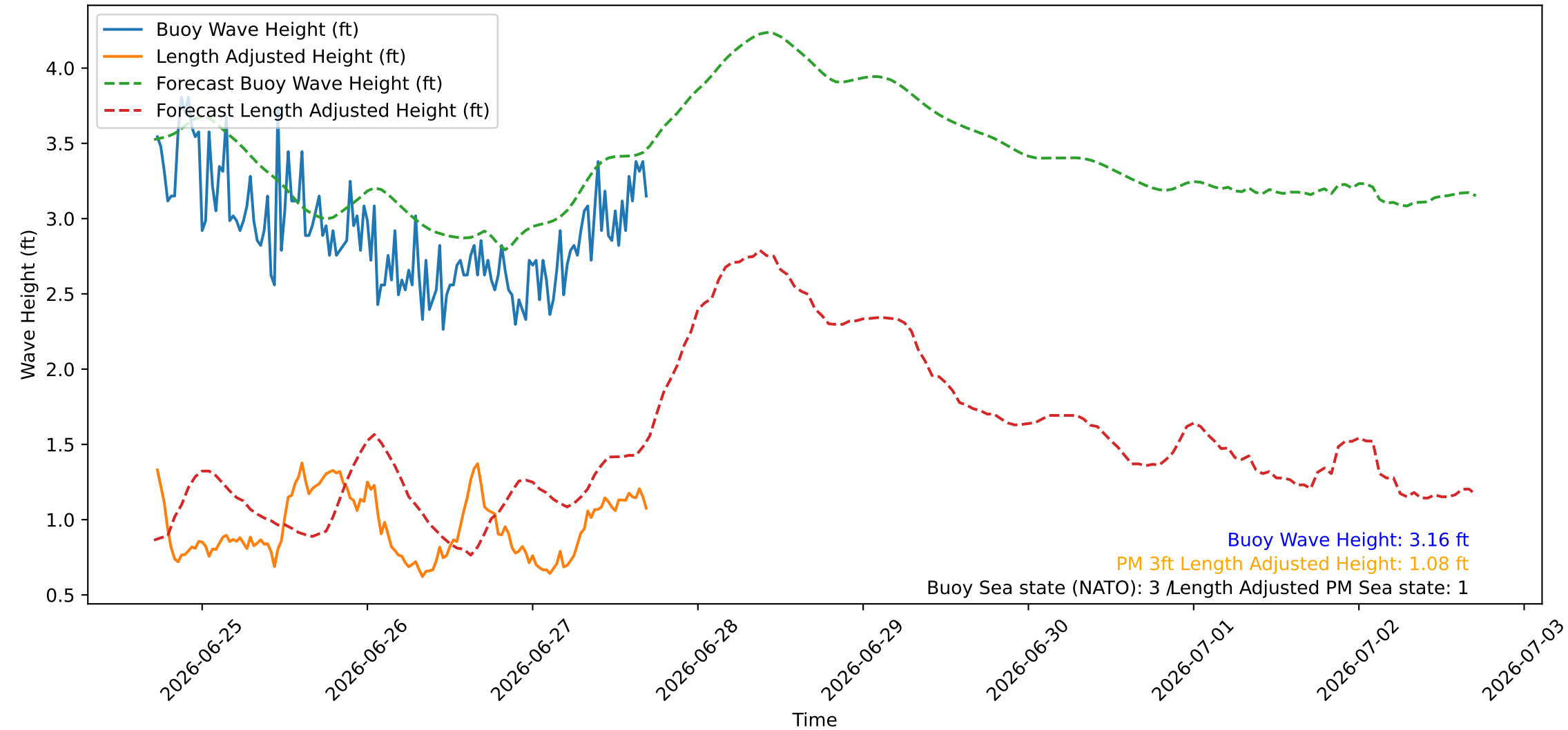
Wave Heights over Time for Red Beach at 2026-06-27 17:10:45
