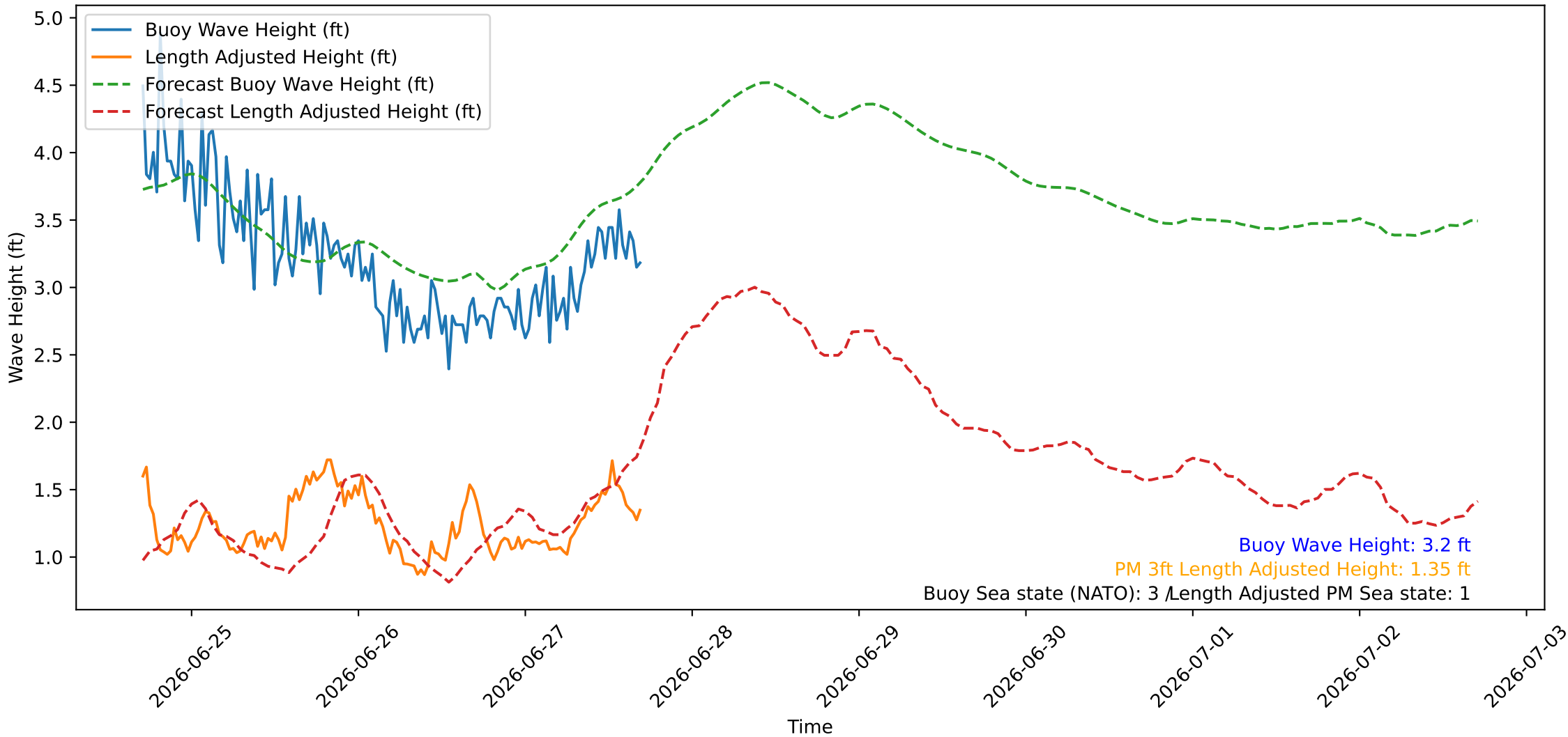
Wave Heights over Time for Oceanside Harbor at 2026-06-27 17:10:26
