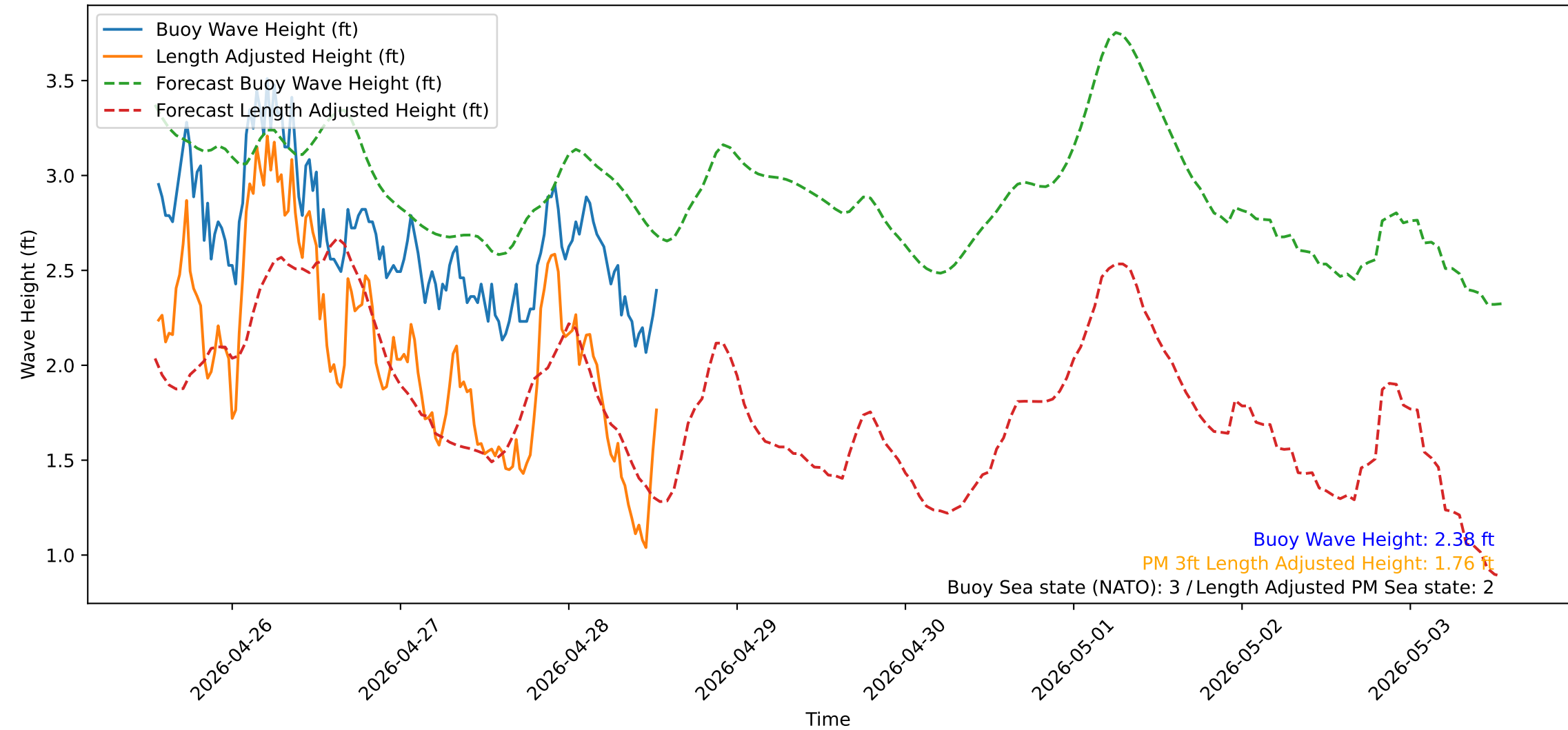
Wave Heights over Time for Green Beach at 2026-04-28 13:21:14
