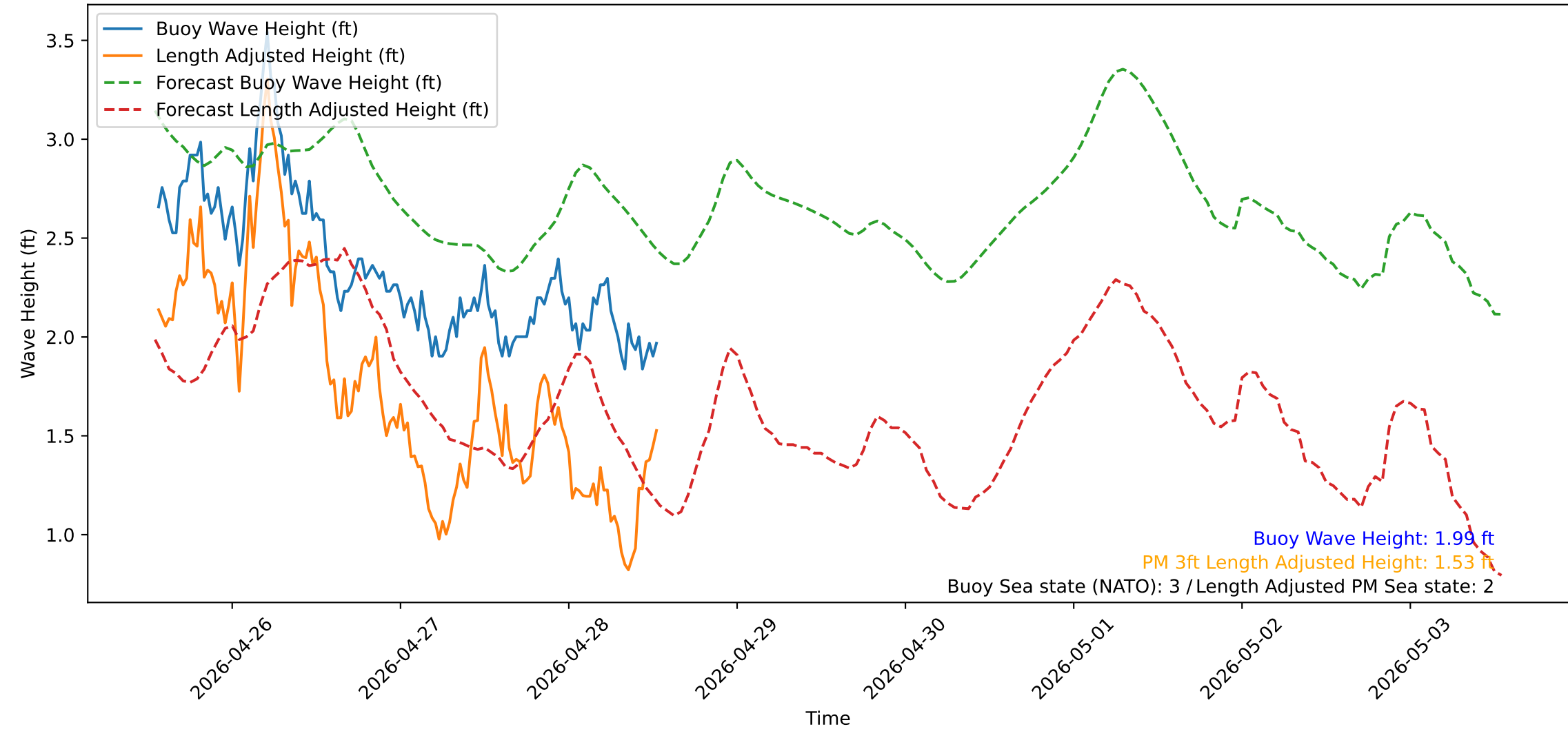
Wave Heights over Time for Red Beach at 2026-04-28 13:20:52
