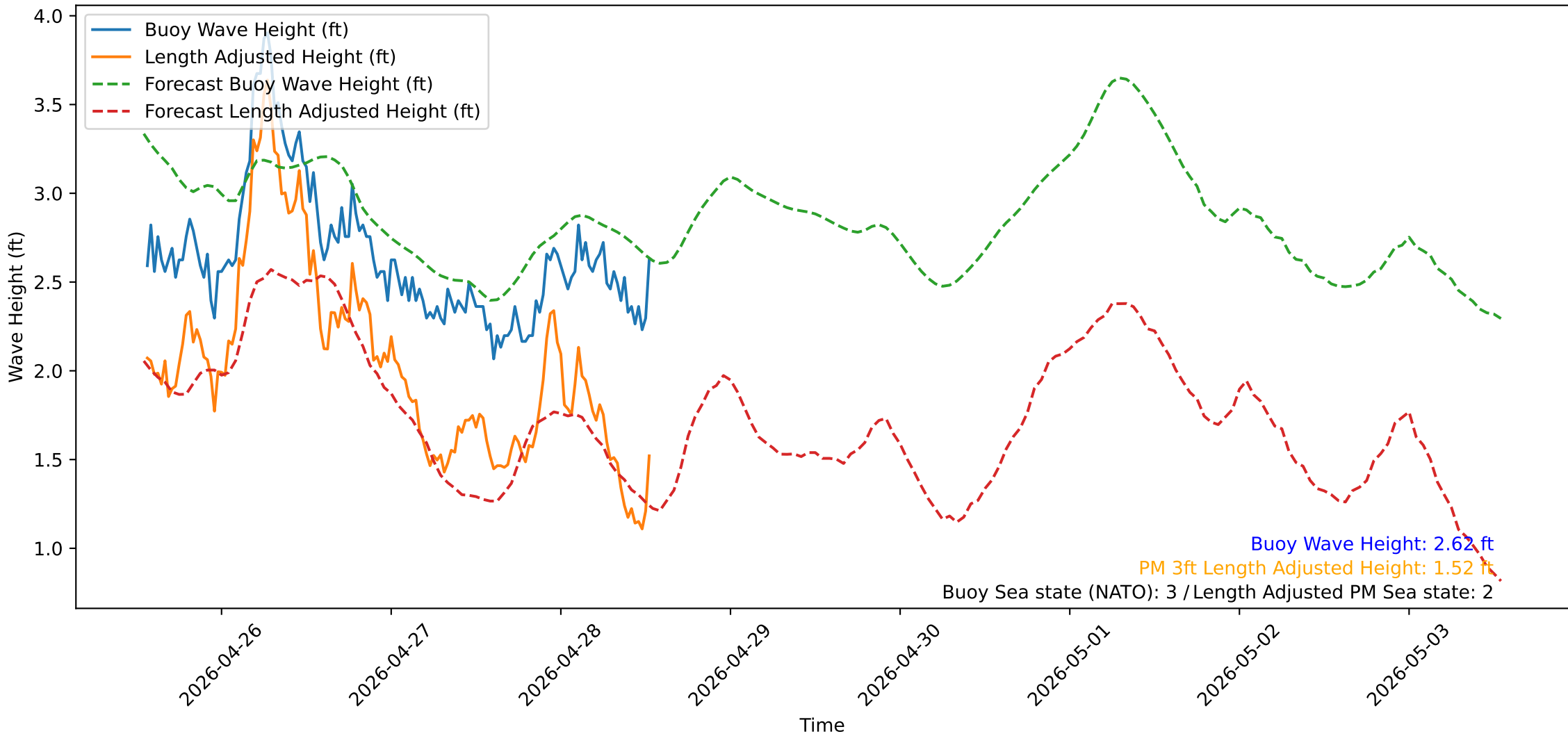
Wave Heights over Time for Oceanside Harbor at 2026-04-28 13:20:31
