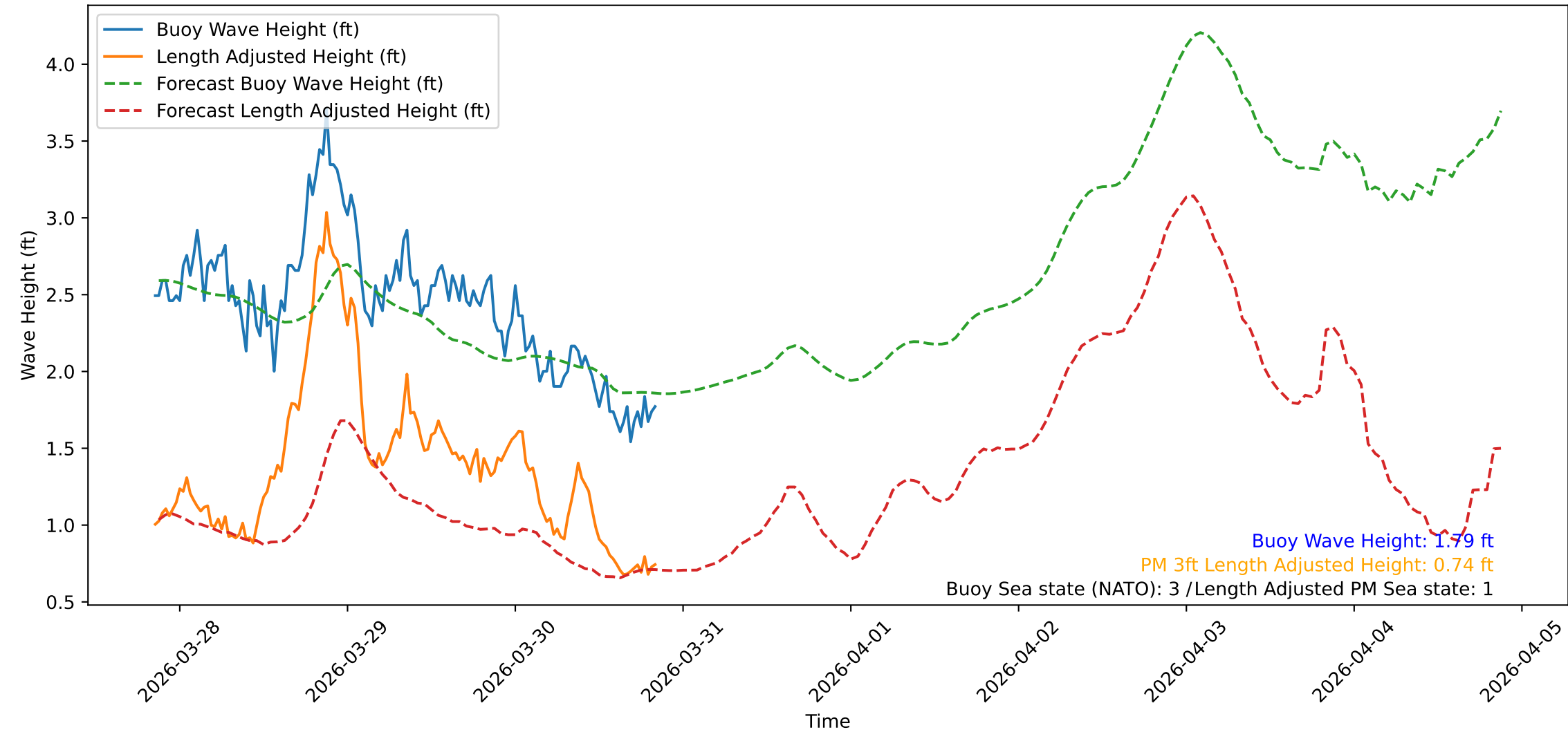
Wave Heights over Time for Green Beach at 2026-03-30 20:41:09
