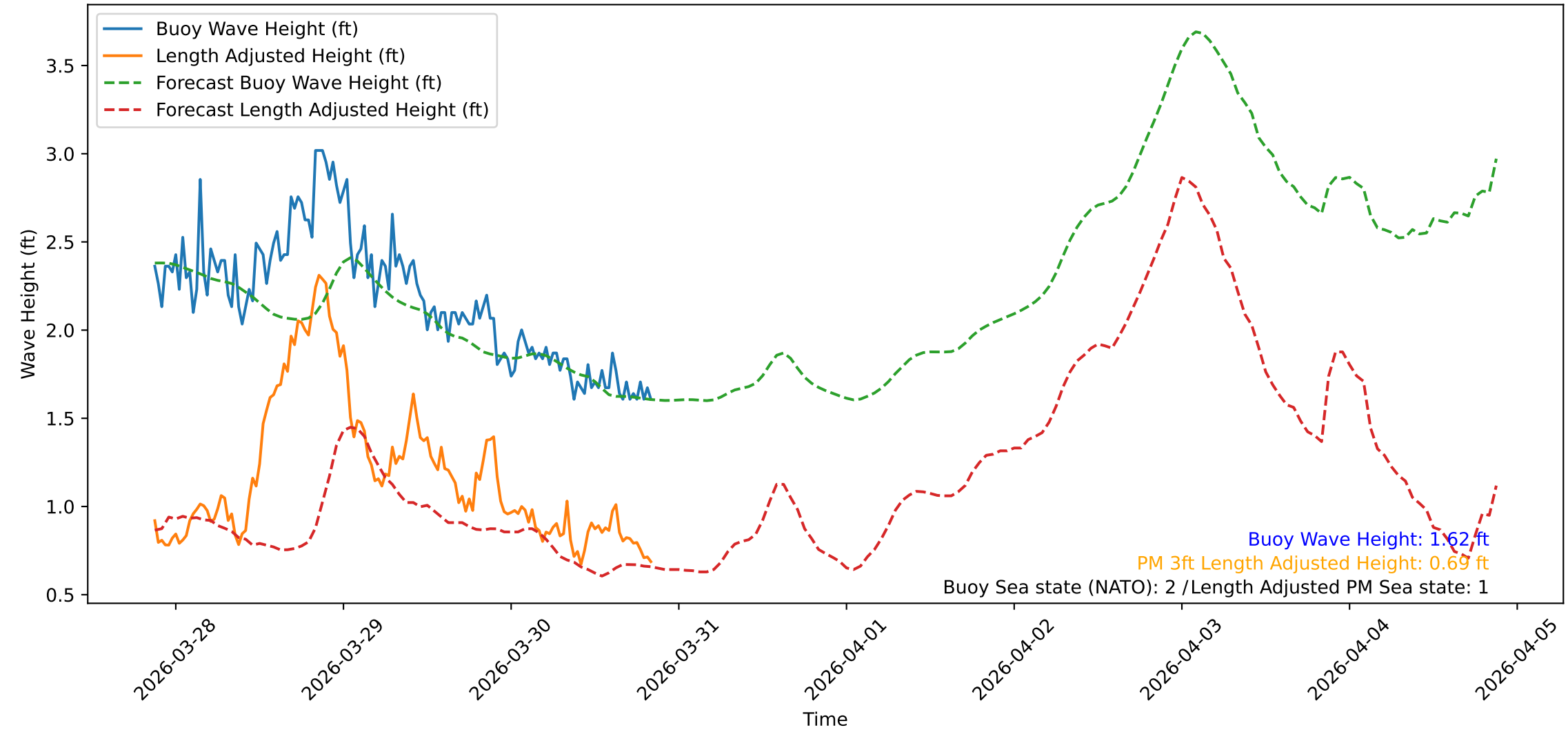
Wave Heights over Time for Red Beach at 2026-03-30 20:40:47
