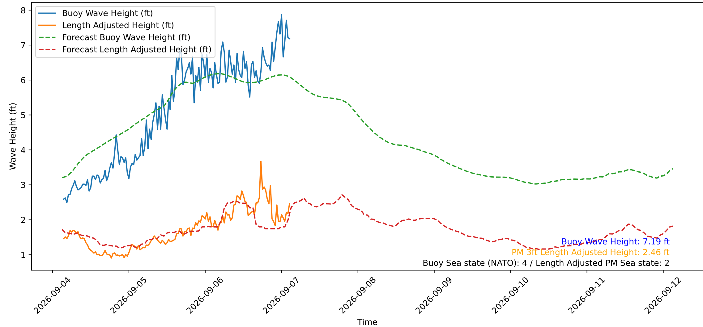
Wave Heights over Time for Green Beach at 2026-09-07 03:21:14
