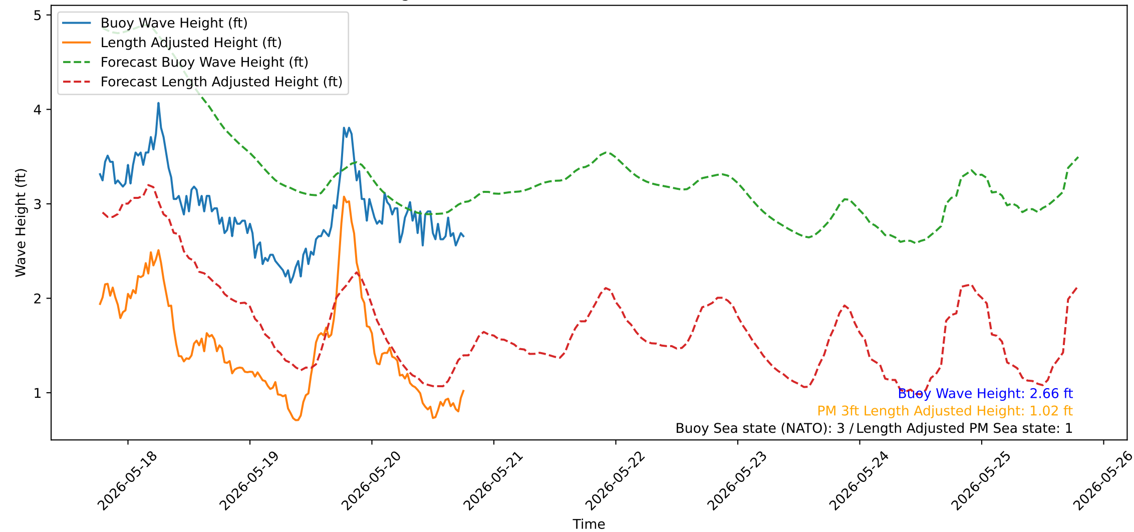
Wave Heights over Time for Green Beach at 2026-05-20 18:41:14
