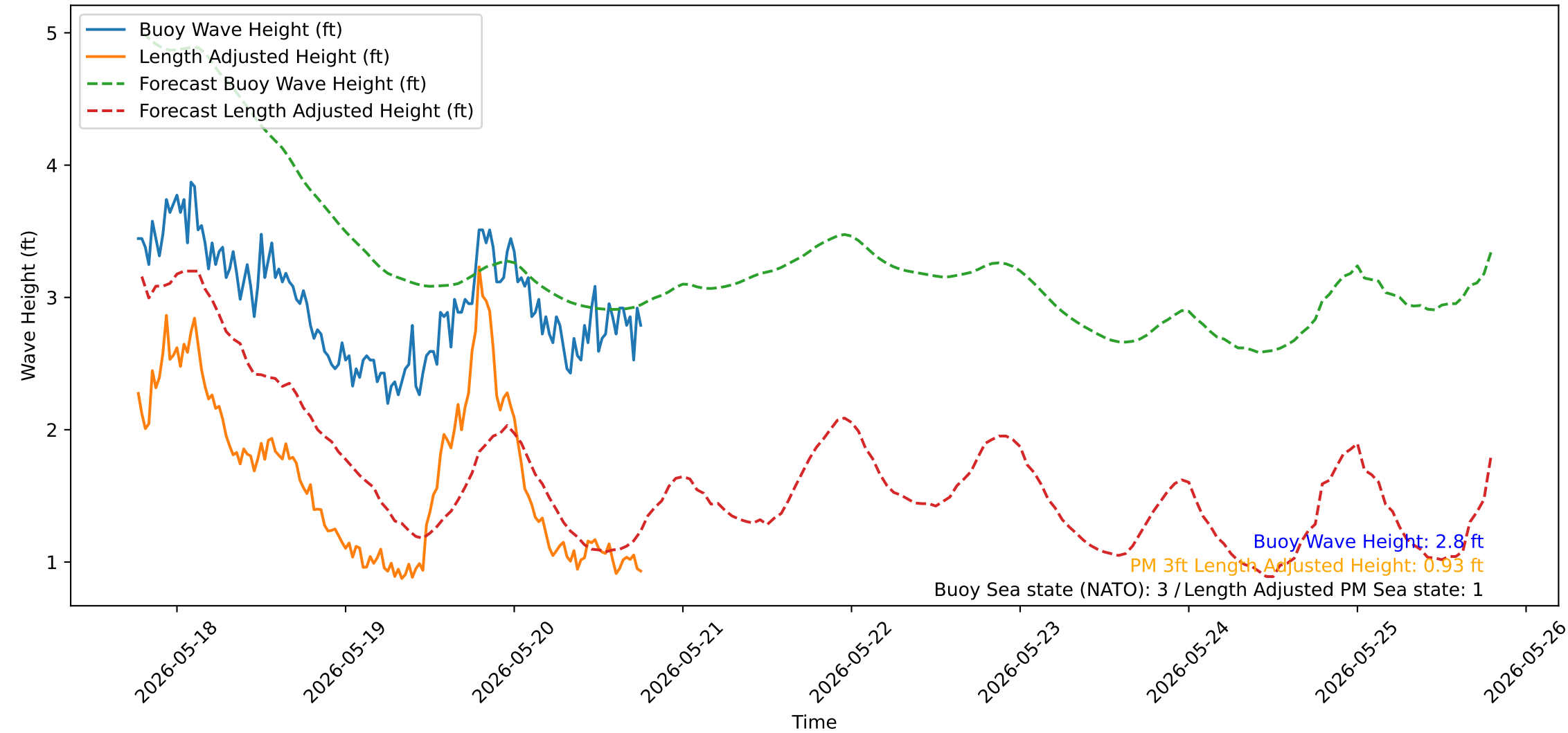
Wave Heights over Time for Oceanside Harbor at 2026-05-20 18:40:31
