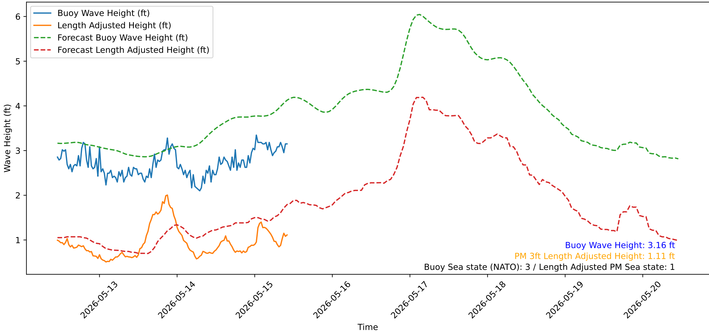
Wave Heights over Time for Green Beach at 2026-05-15 10:51:16
