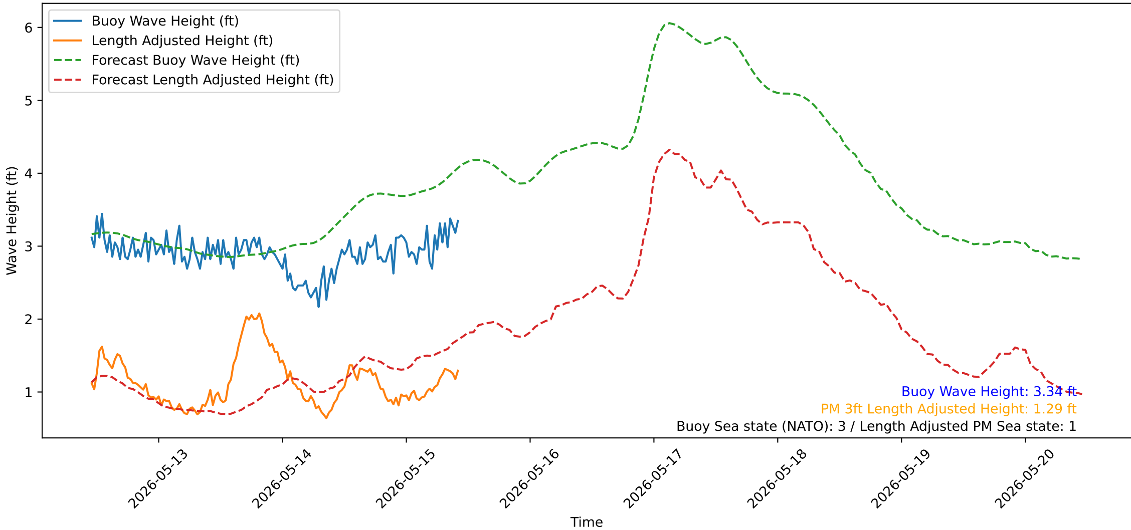
Wave Heights over Time for Oceanside Harbor at 2026-05-15 10:50:32
