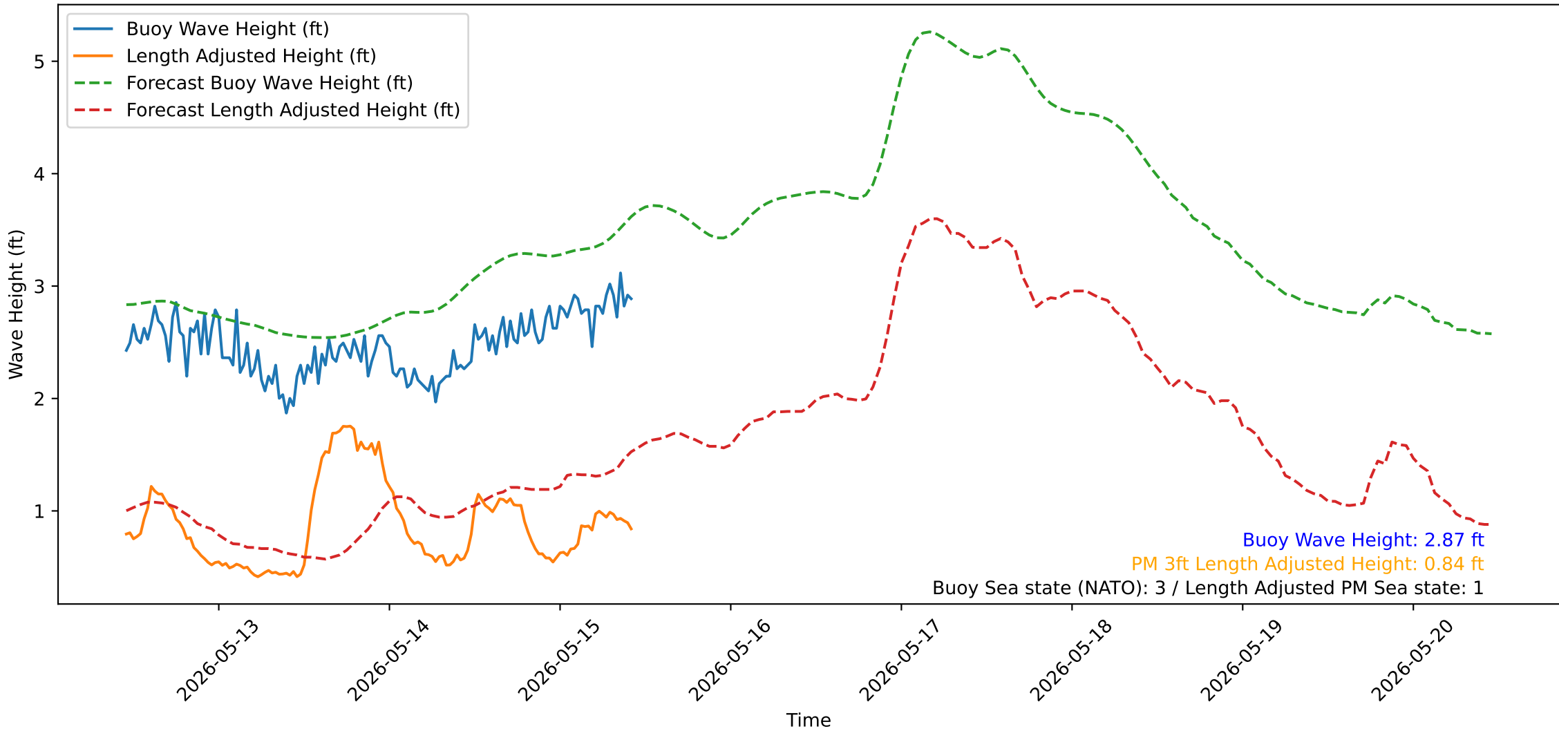
Wave Heights over Time for Red Beach at 2026-05-15 10:50:52
