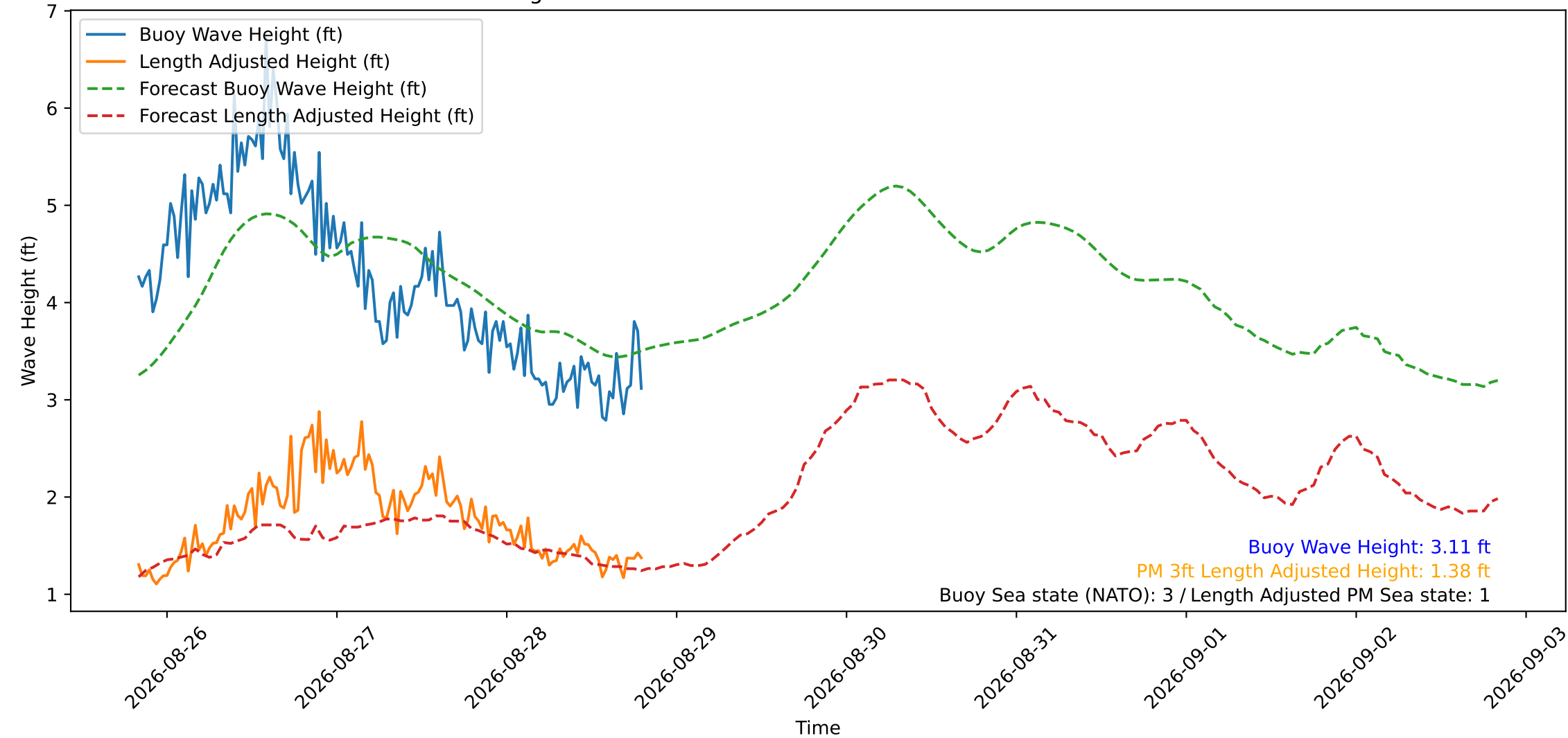
Wave Heights over Time for Oceanside Harbor at 2026-08-28 19:50:30
